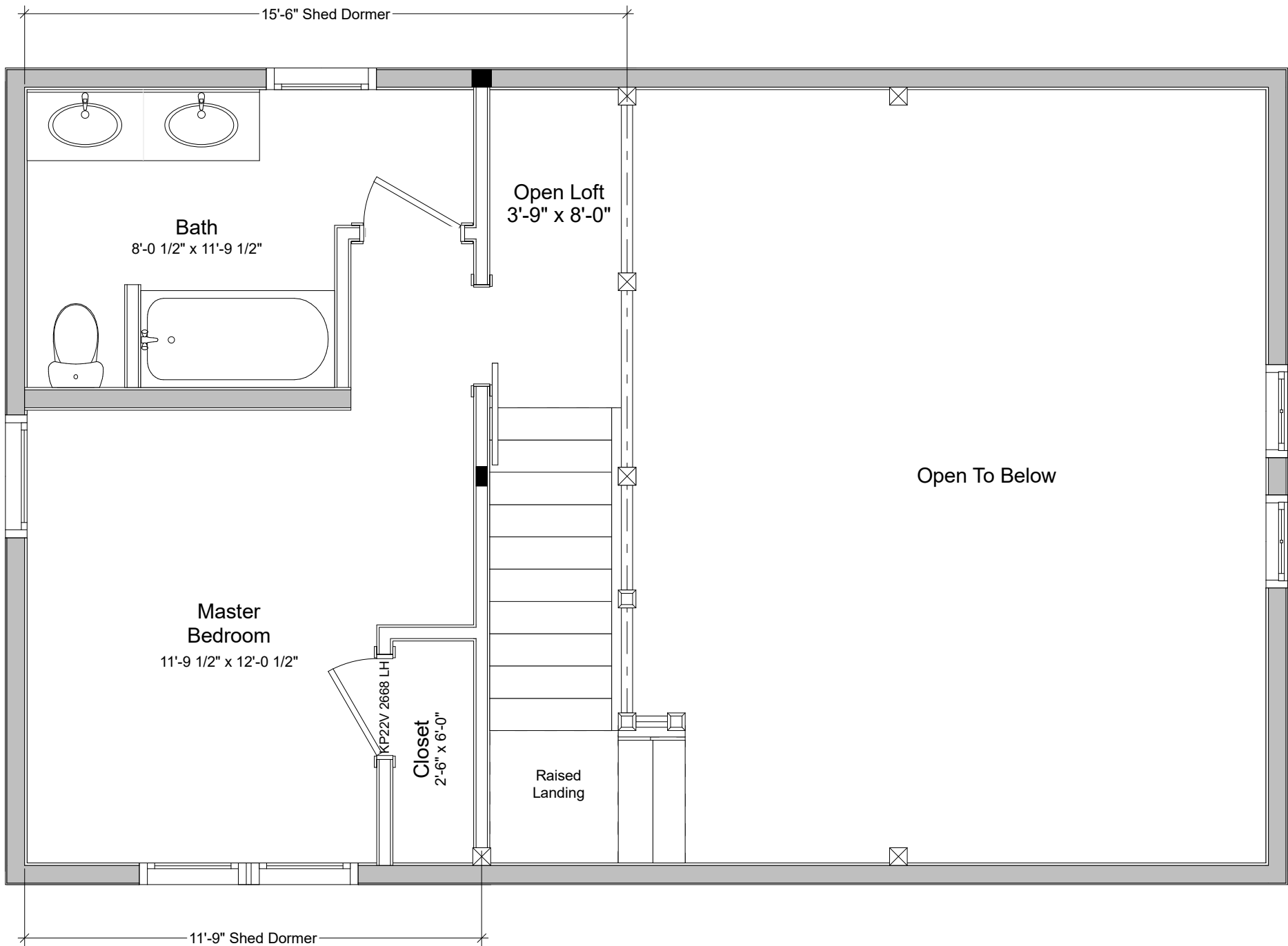
Second Floor Plan 317 sq. ft.
