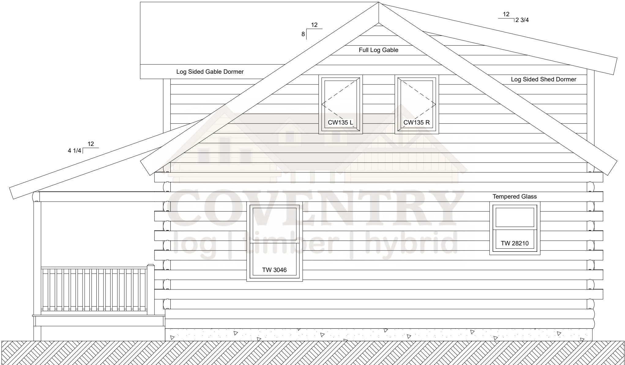
Clearwater Right Elevation
