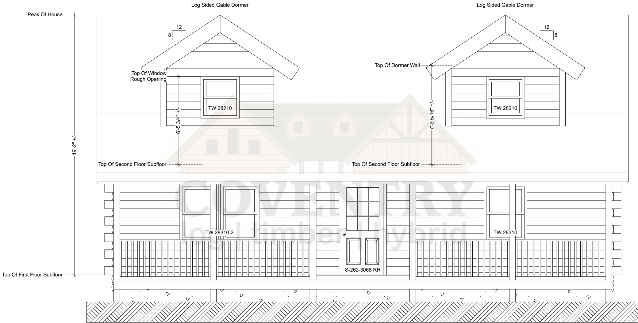
Clearwater Front Elevation
