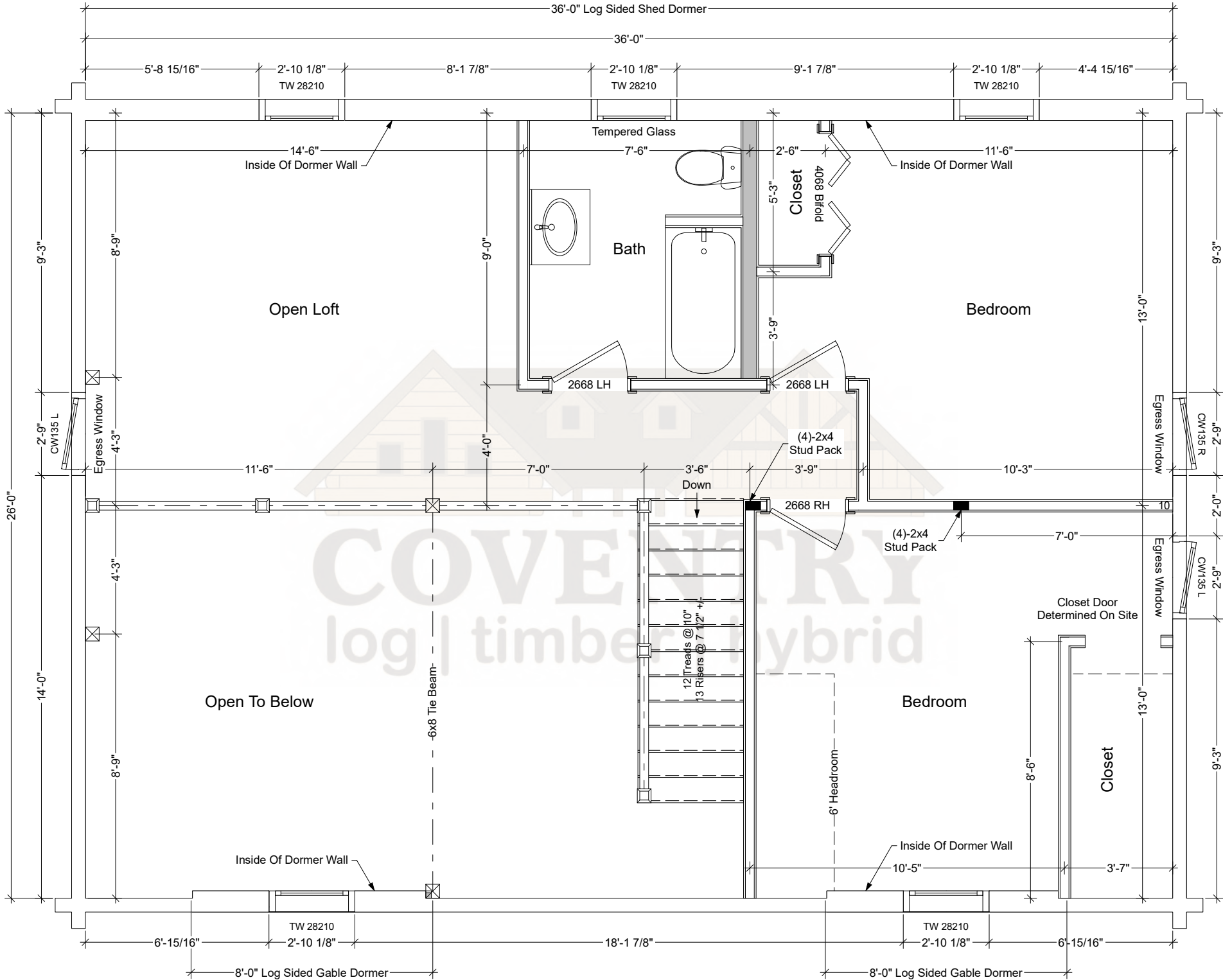
Clearwater Second Floor Plan
