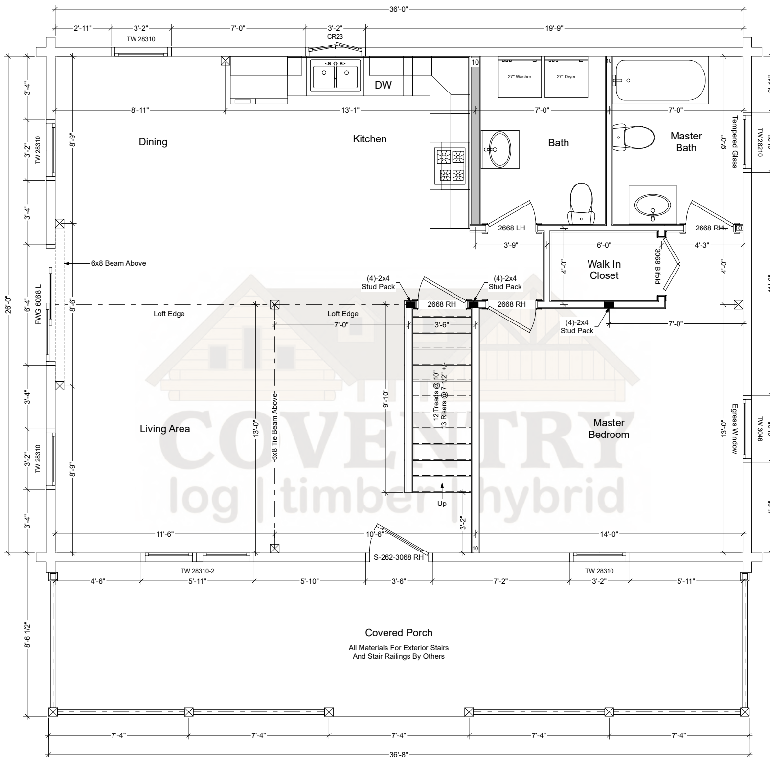
Clearwater First Floor Plan
