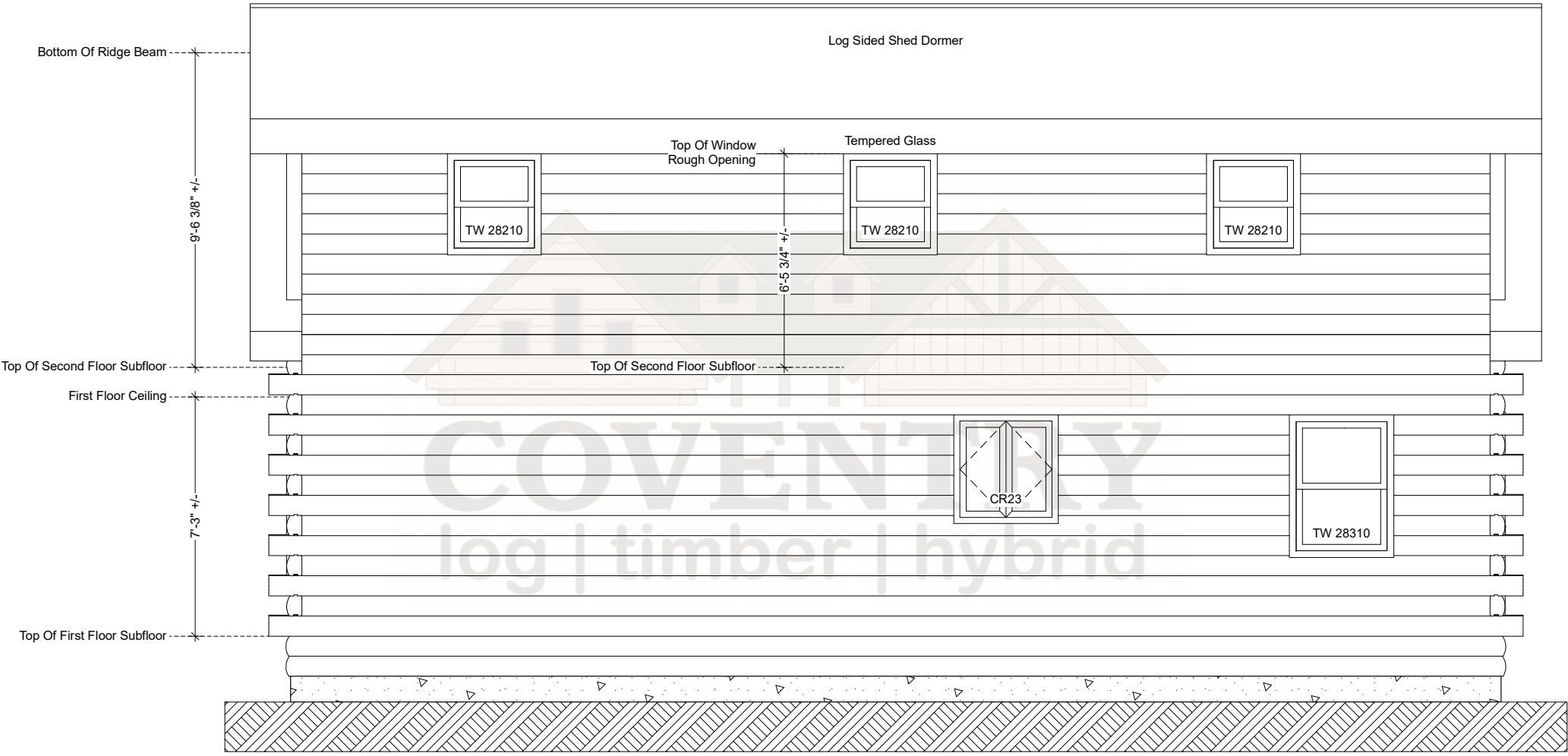
Clearwater Rear Elevation
