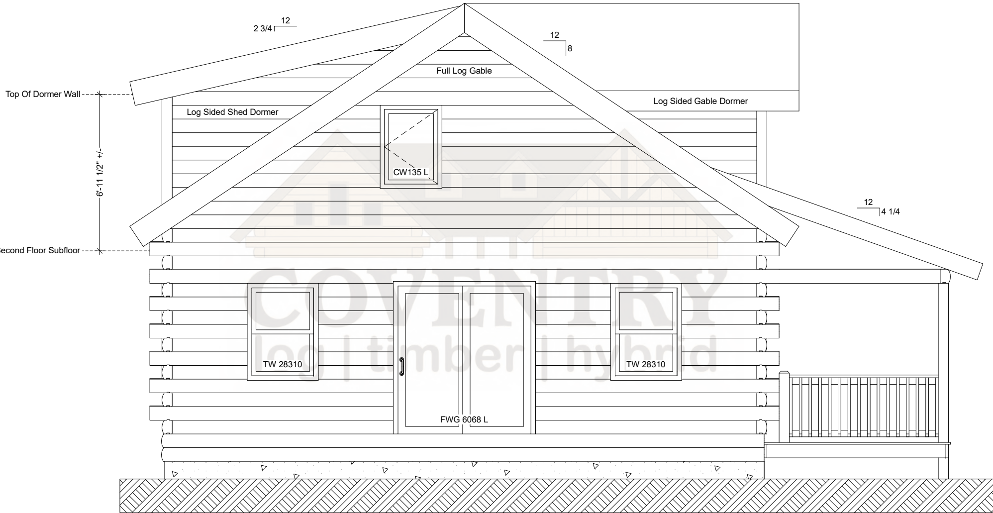
Clearwater Left Elevation
