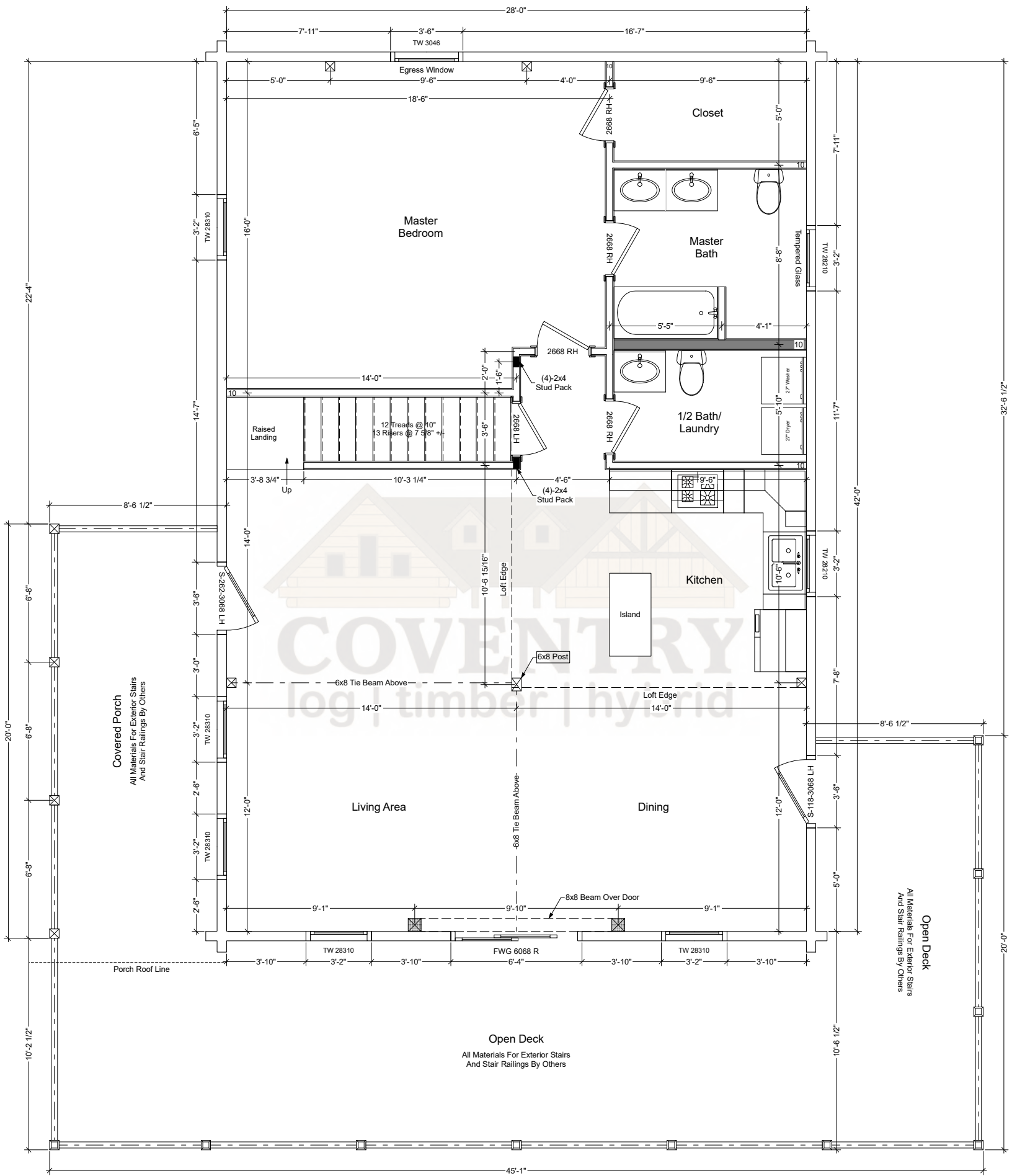
Hillside First Floor Plan
