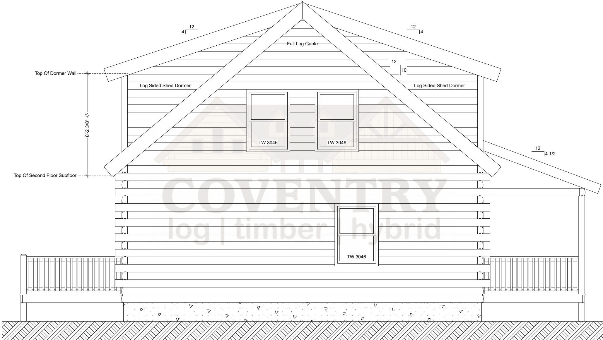
Hillside Rear Elevation
