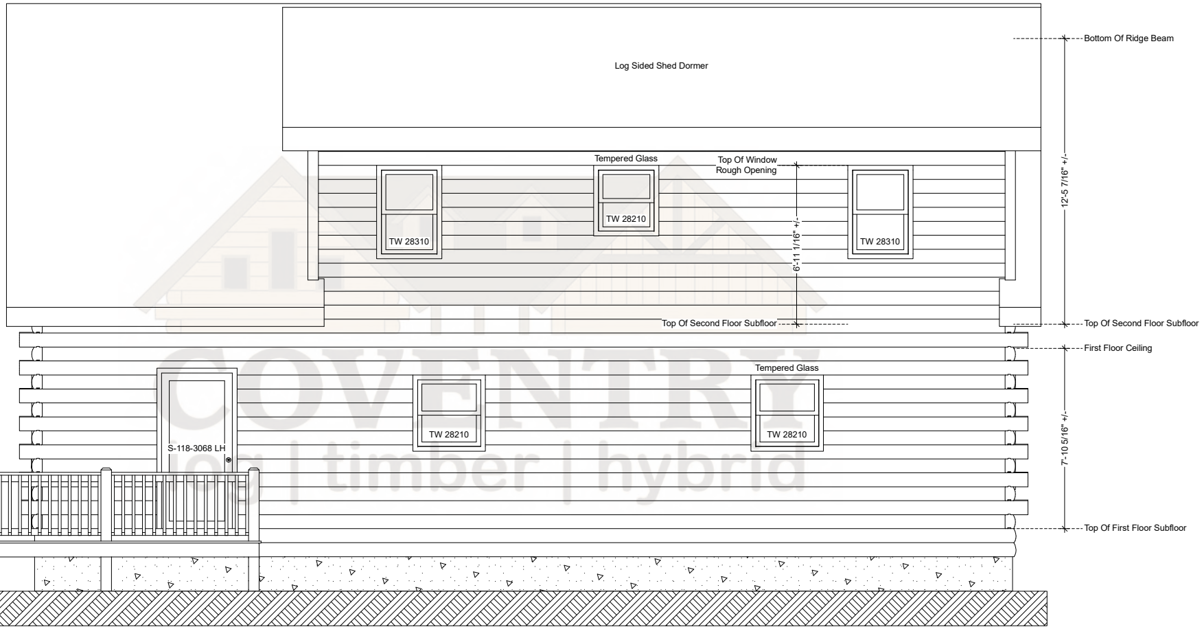
Hillside Right Elevation
