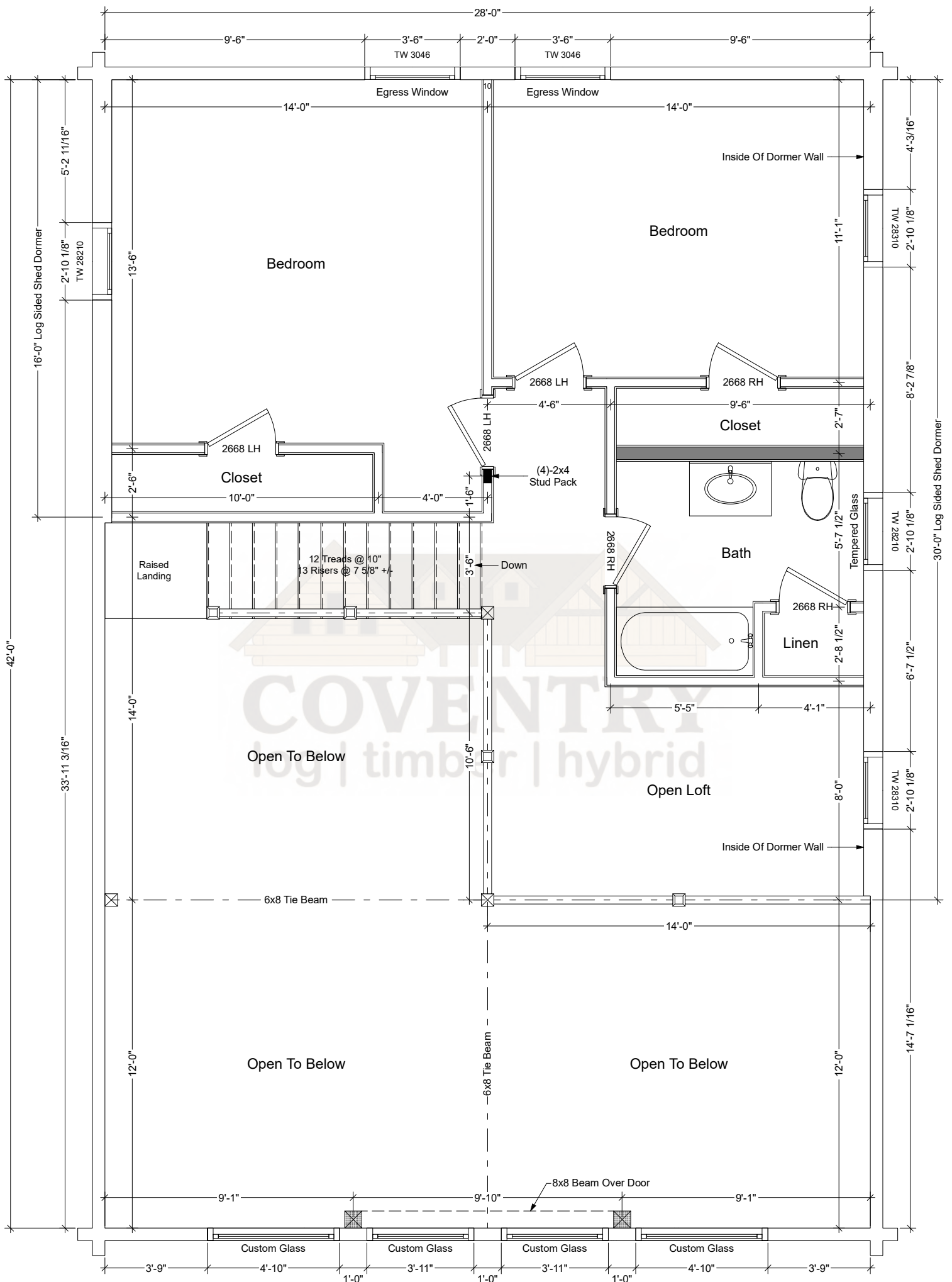
Hillside Second Floor Plan
