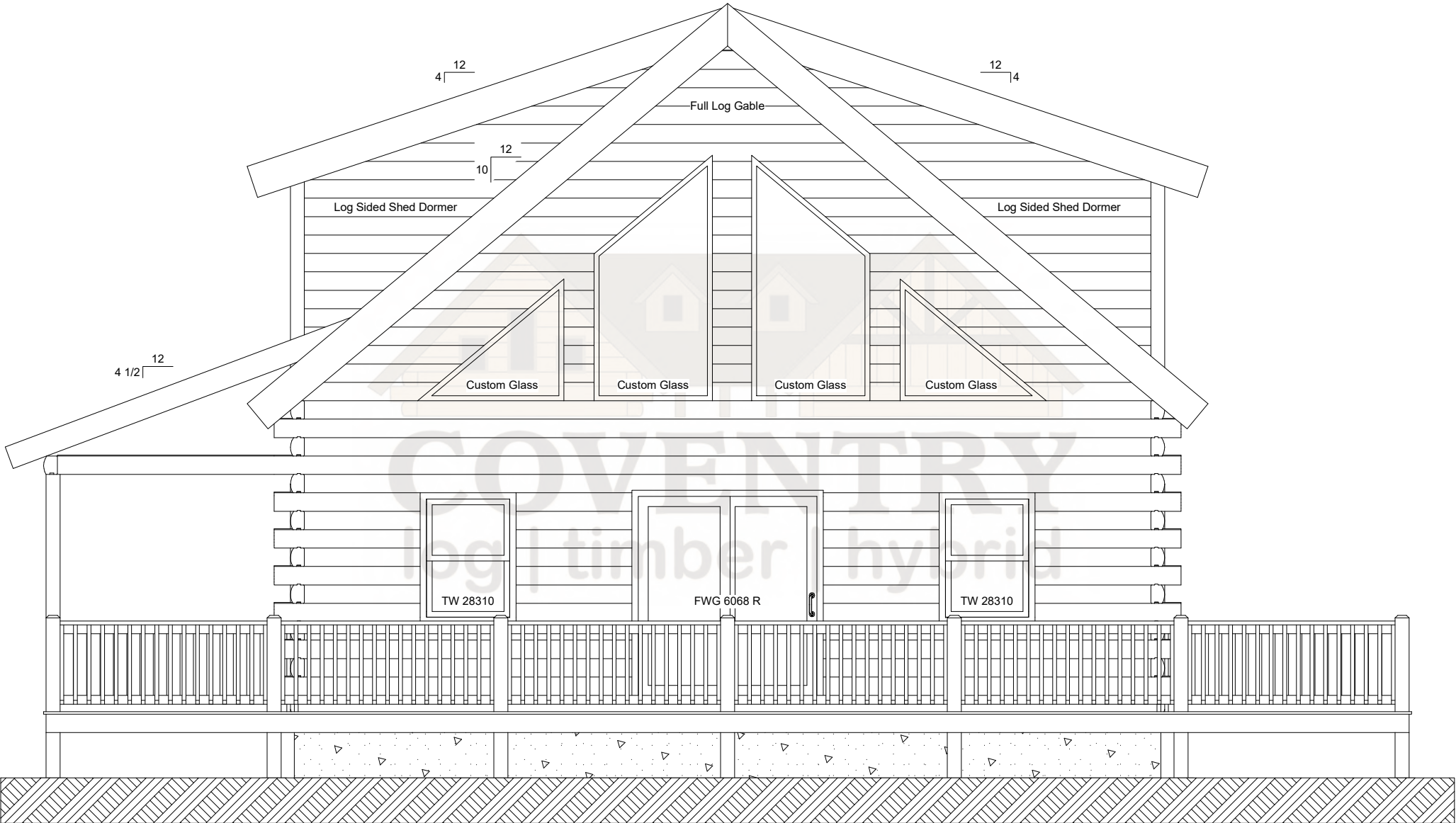
Hillside Front Elevation
