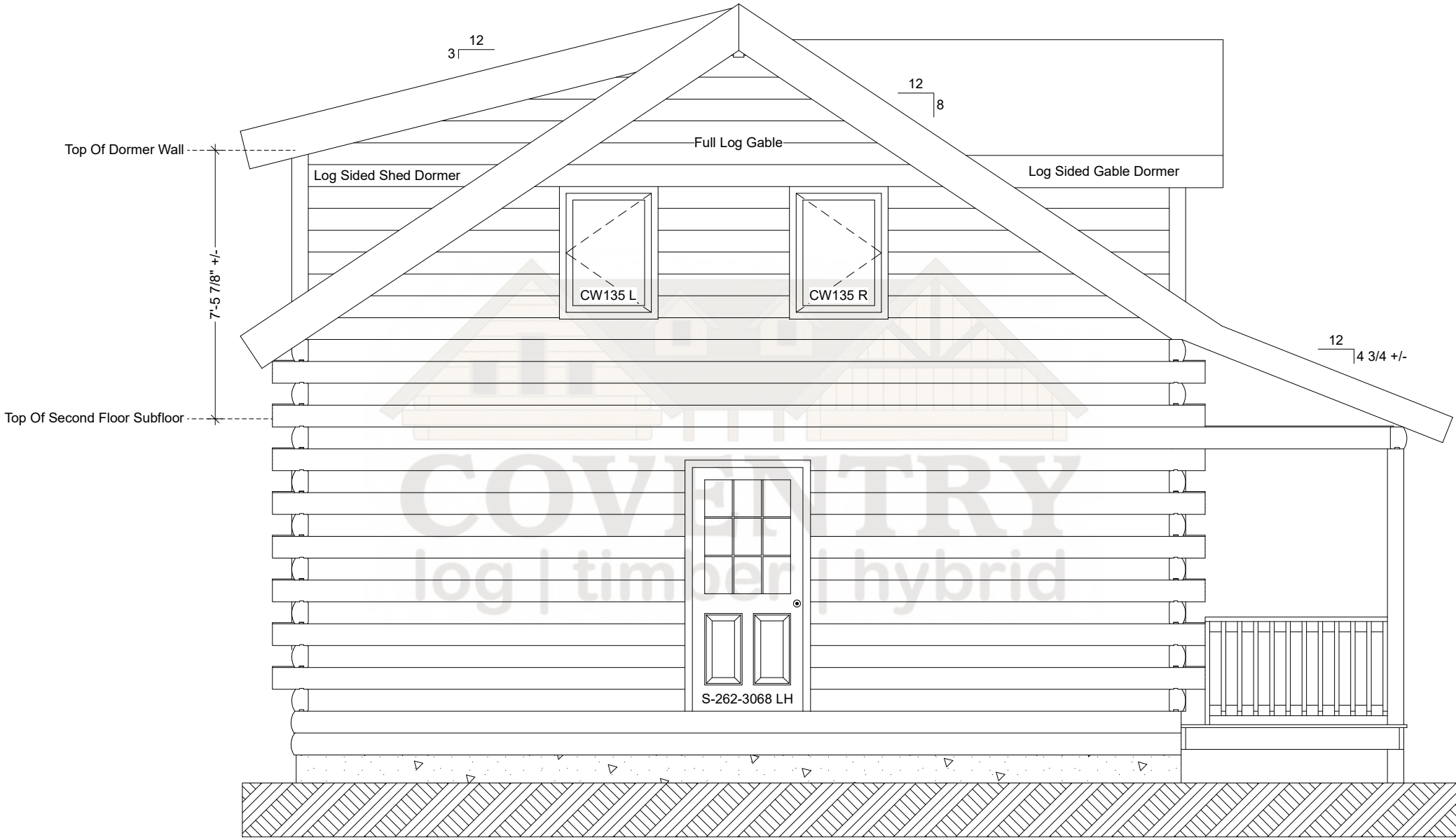
Homestead Left Elevation
