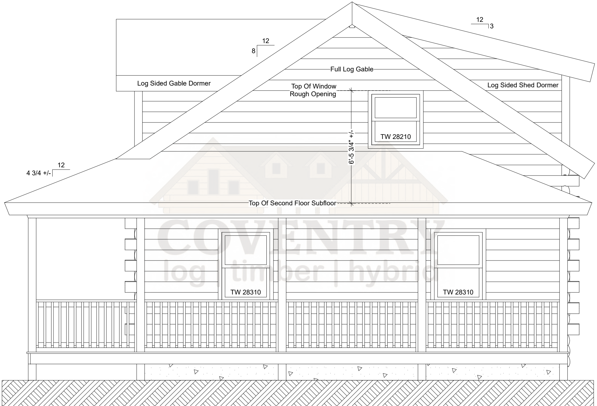
Homestead Right Elevation
