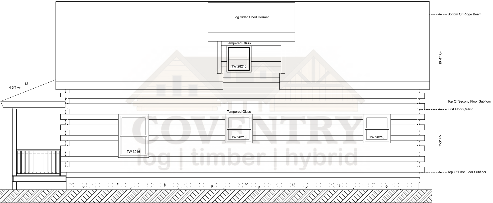
Homestead Rear Elevation
