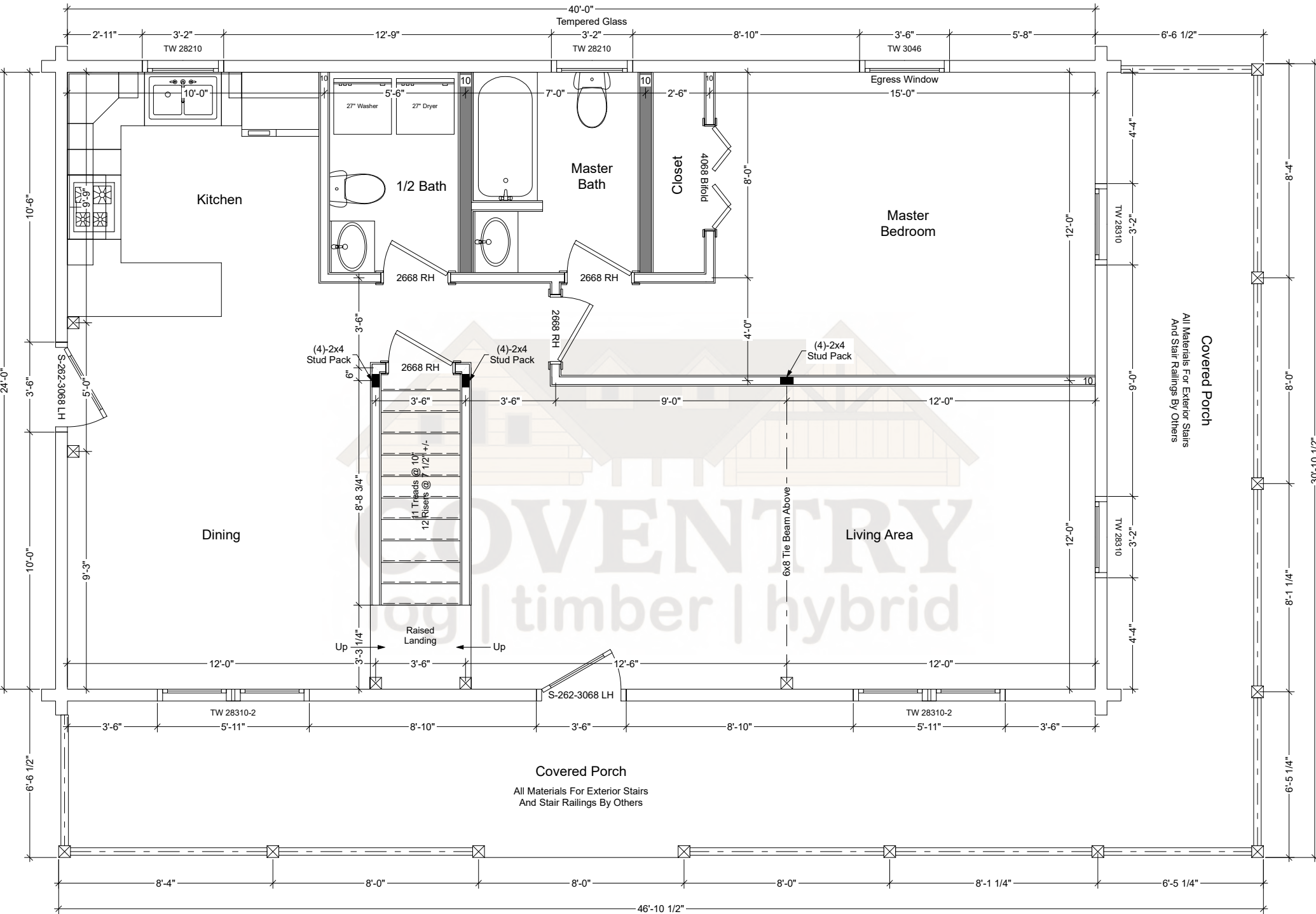
Homestead First Floor Plan
