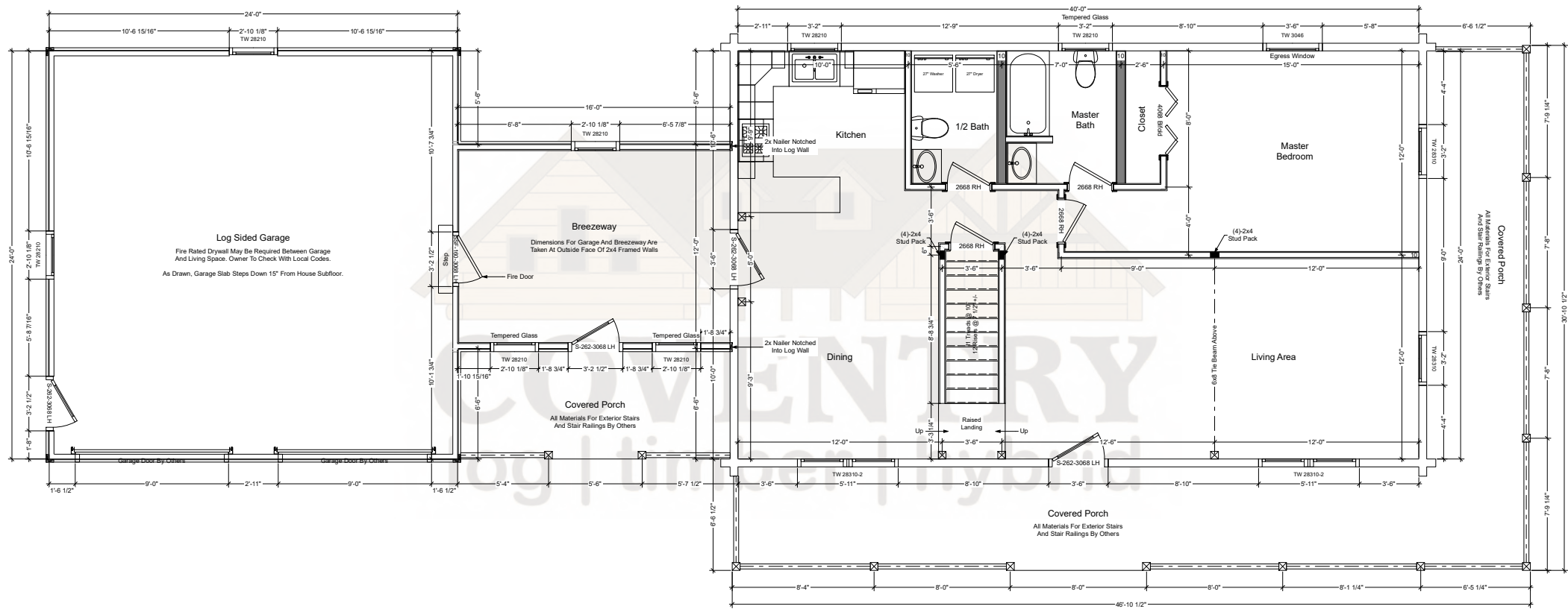
Homestead First Floor Plan
