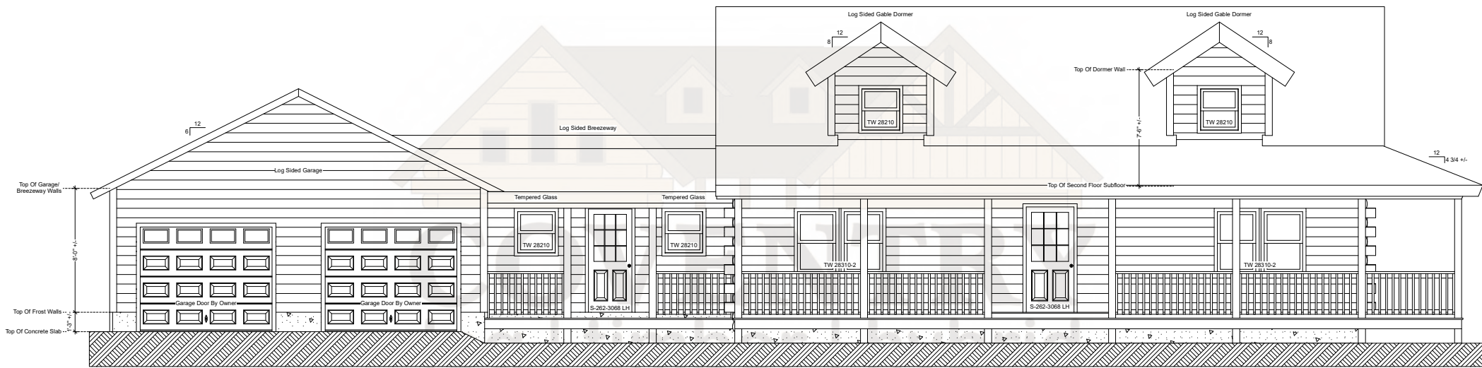
Homestead Front Elevation
