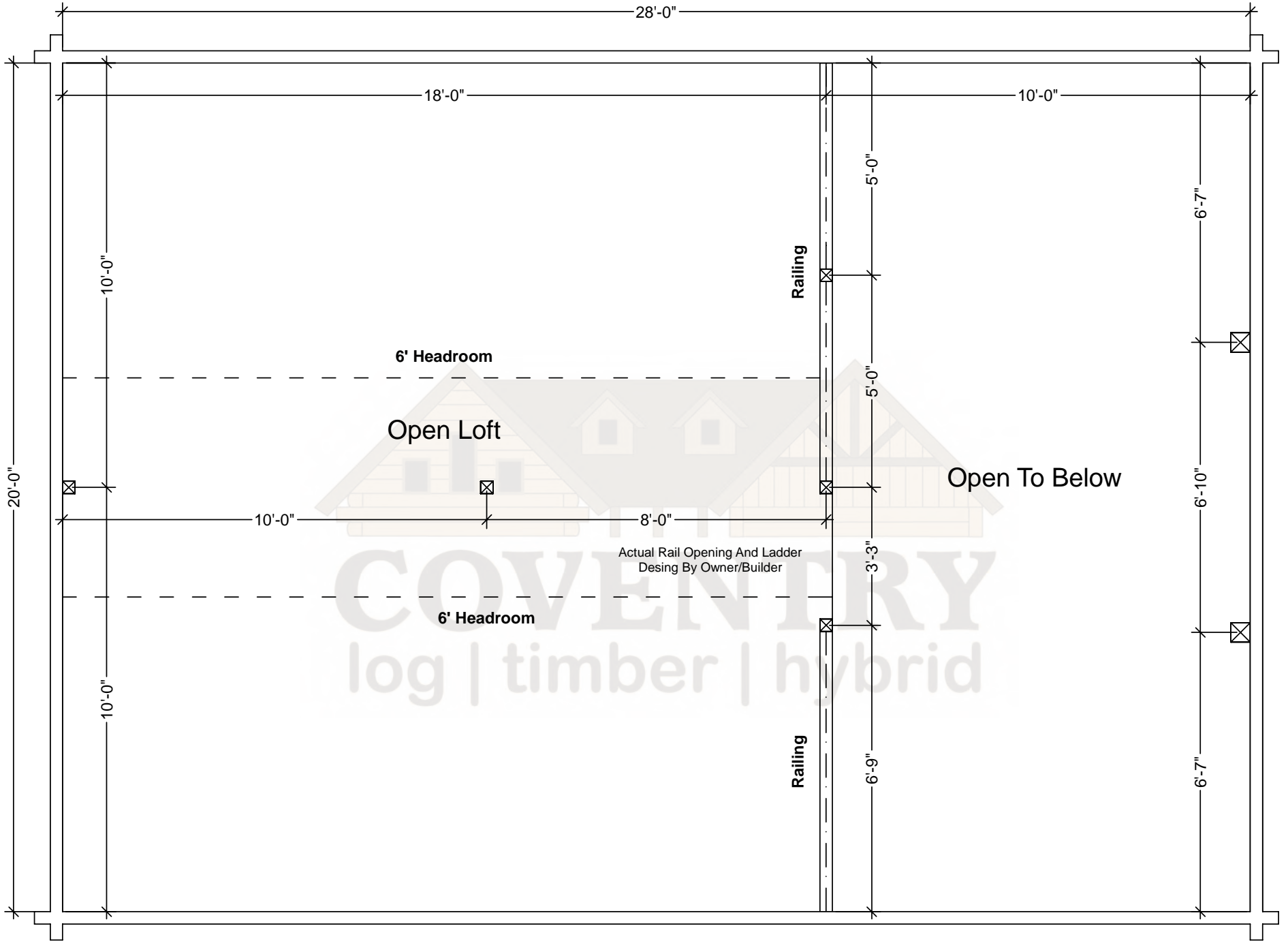
Lakeview Second Floor Plan
