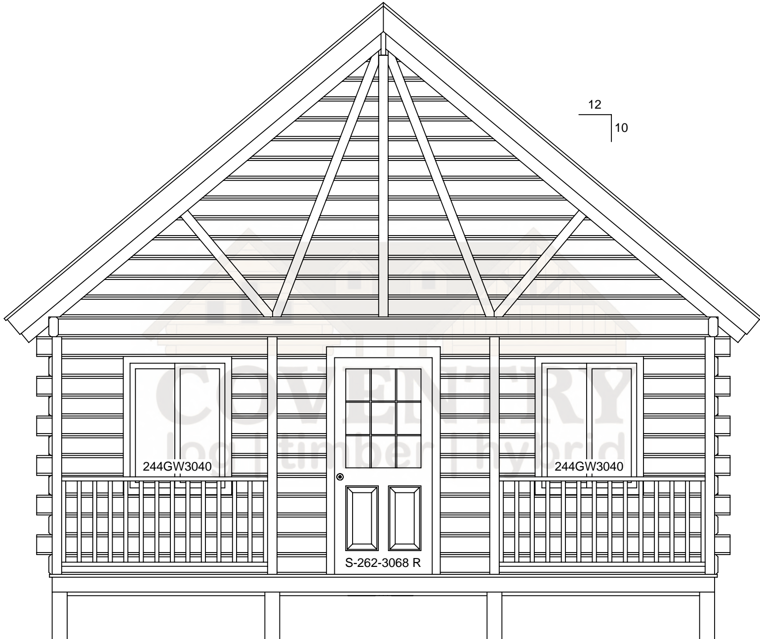
Lakeview Right Elevation
