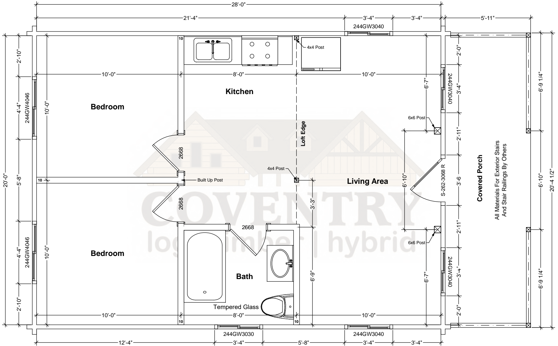
Lakeview First Floor Plan
