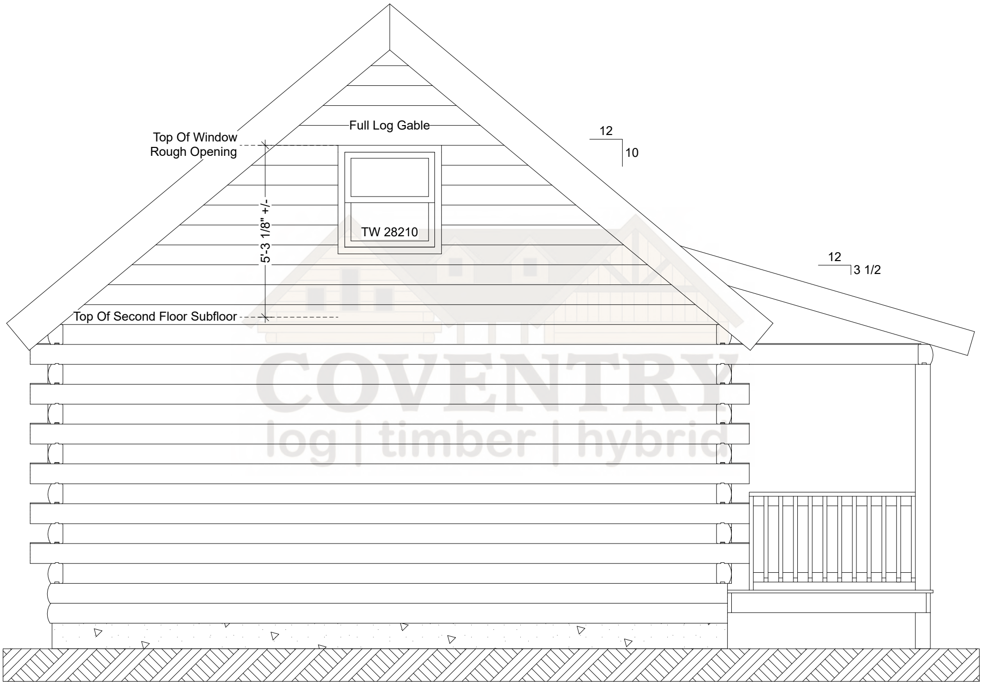
Adventurer Left Elevation
