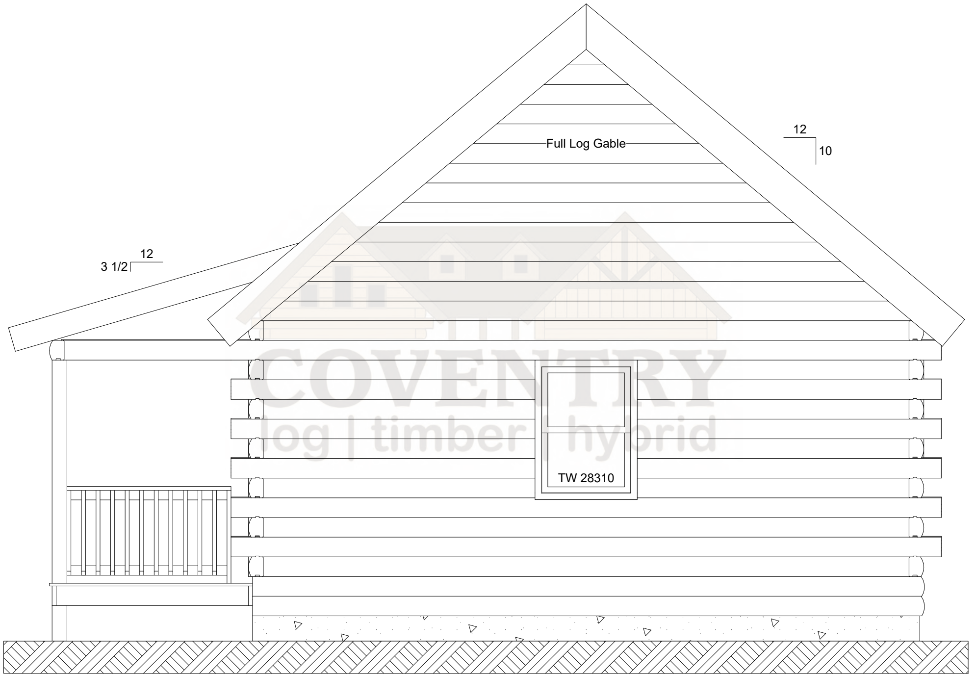
Adventurer Right Elevation
