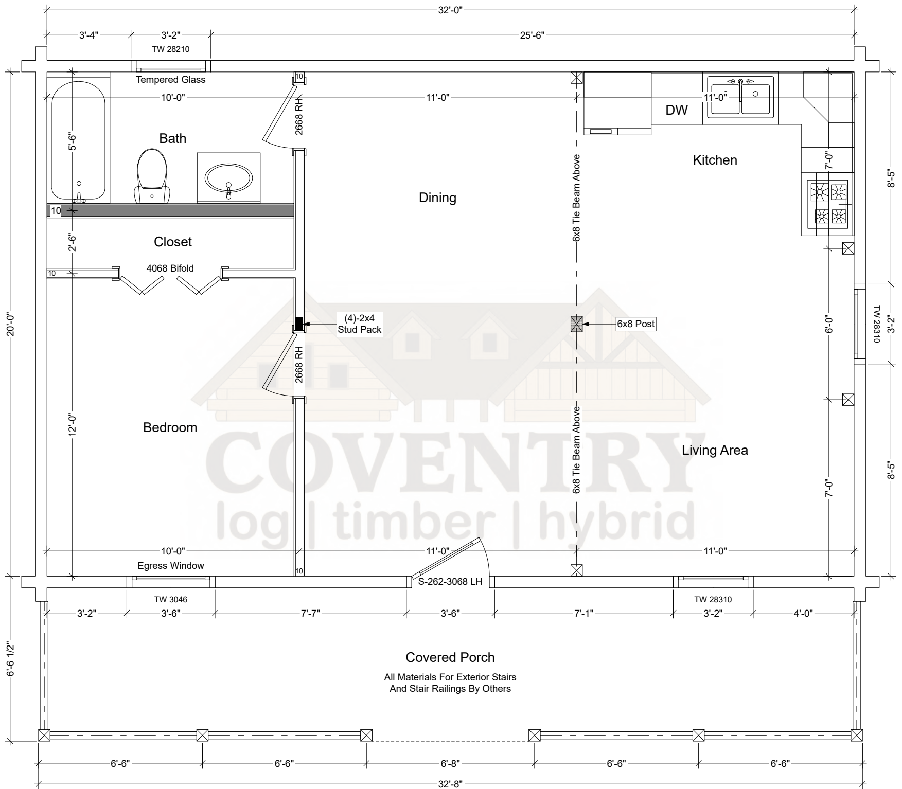
Adventurer First Floor Plan
