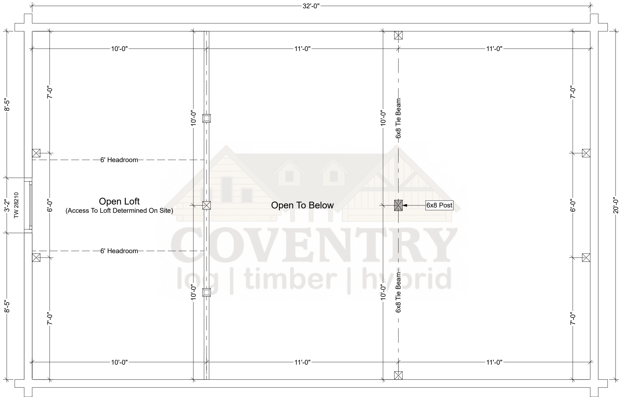
Adventurer Second Floor Plan
