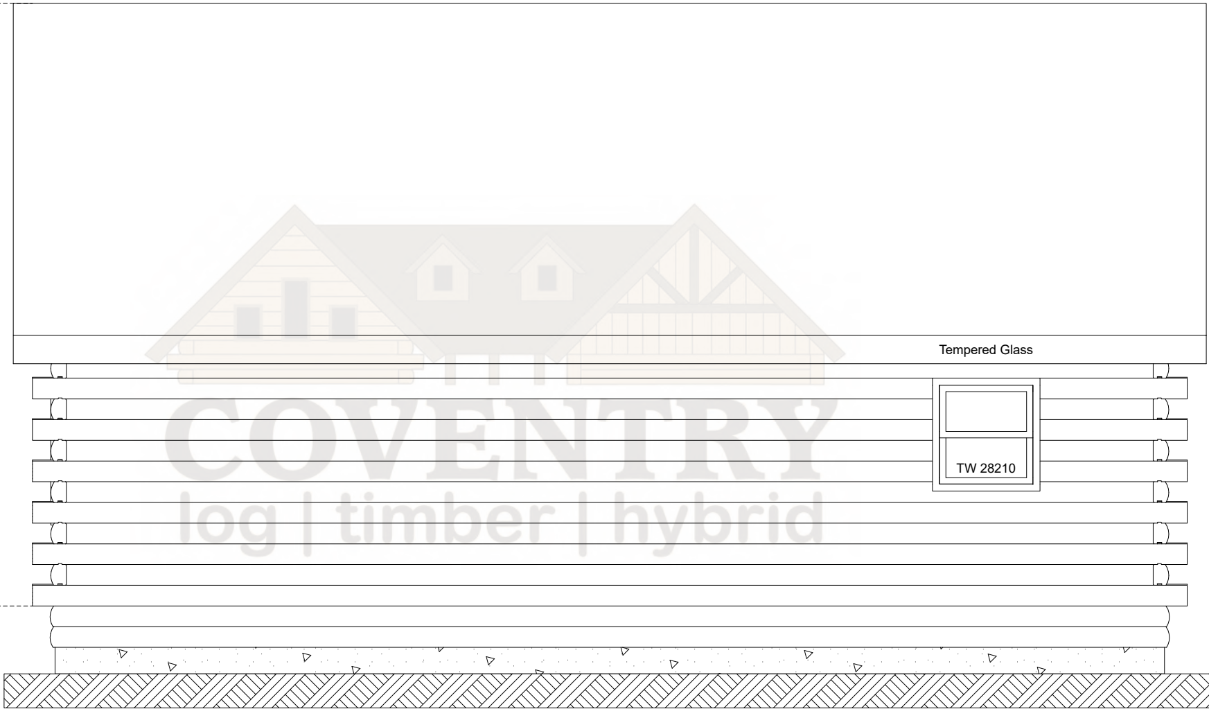
Adventurer Rear Elevation
