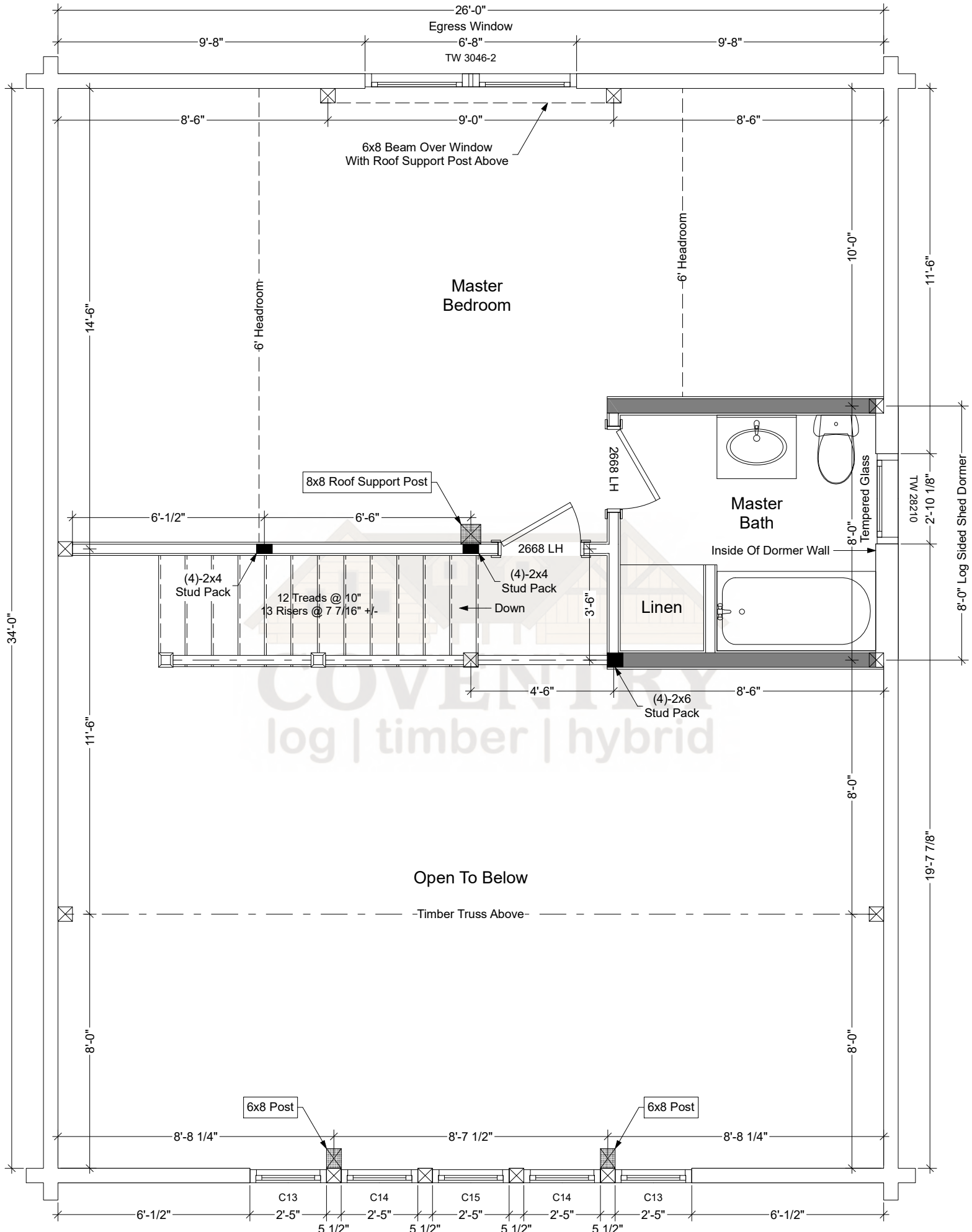
Alpine Second Floor Plan
