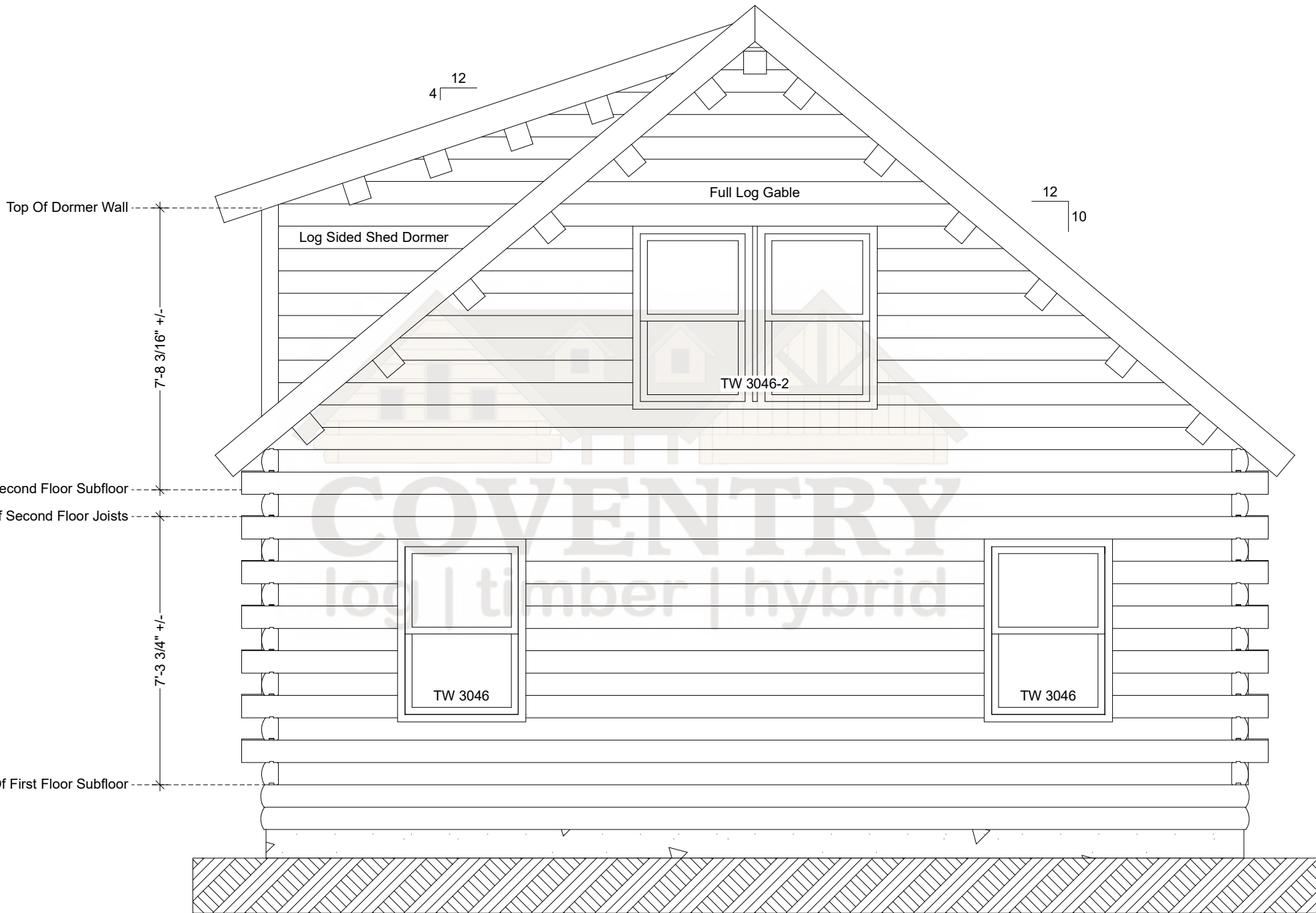
Alpine Rear Elevation
