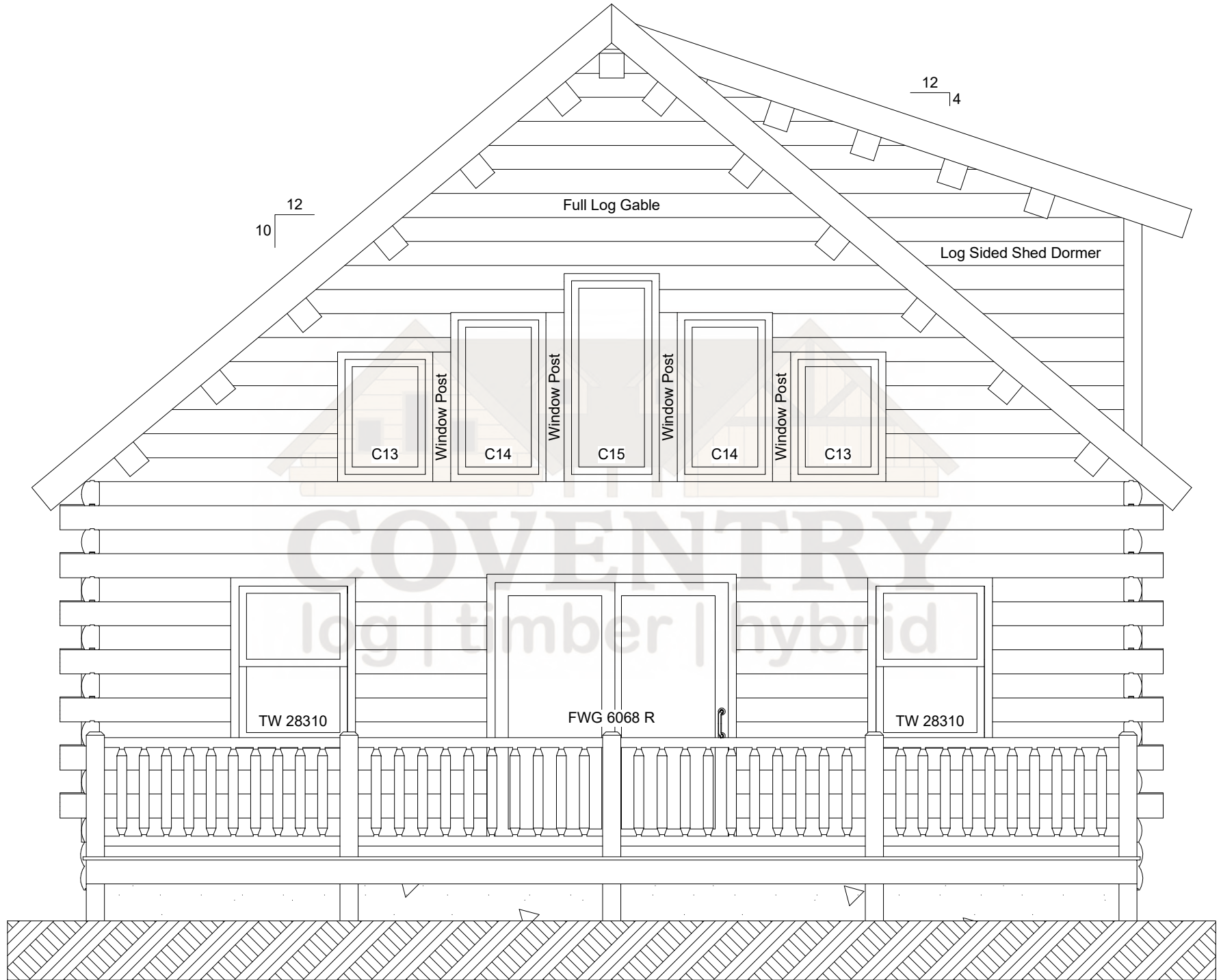
Alpine Front Elevation
