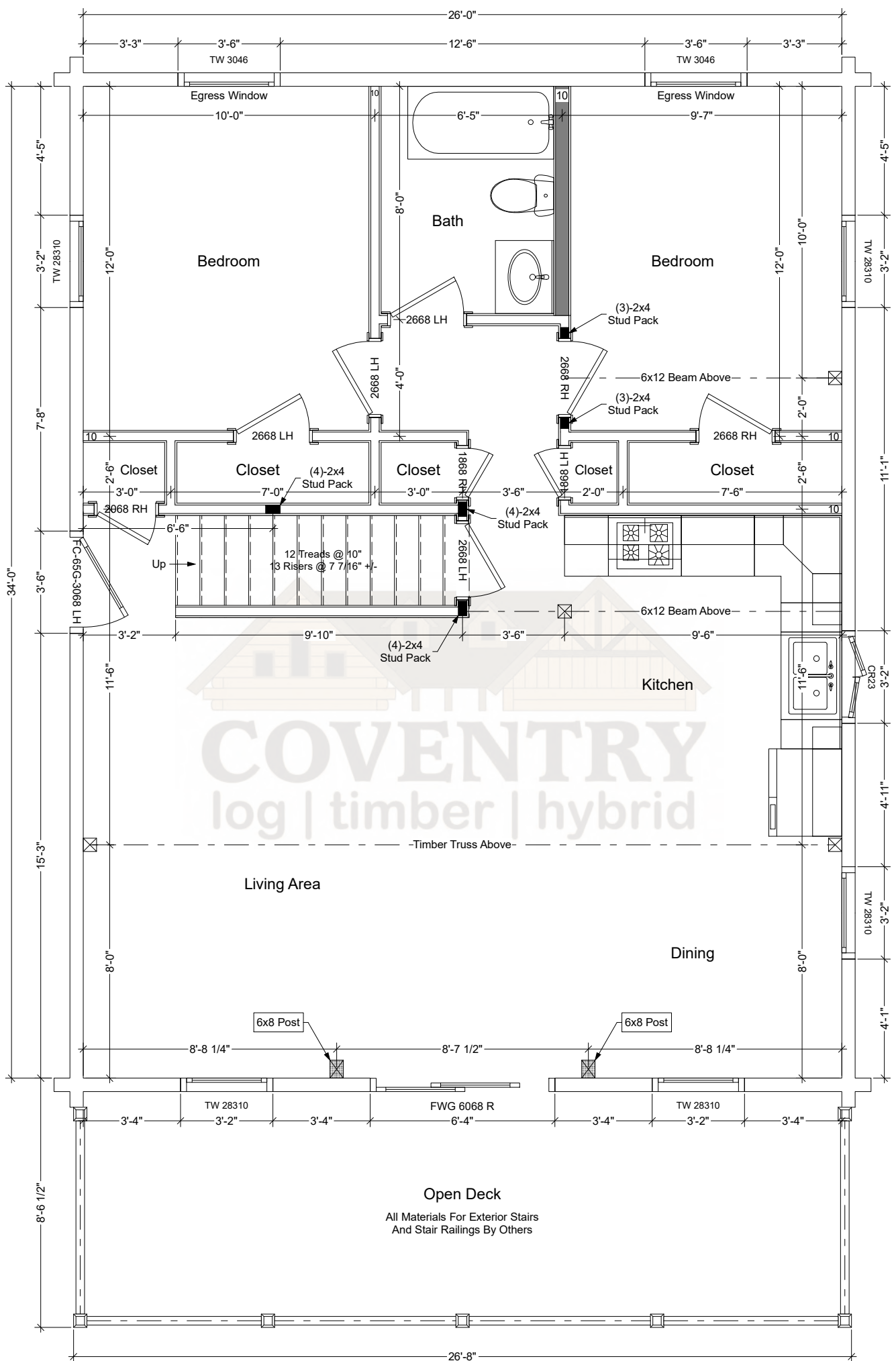
Alpine First Floor Plan
