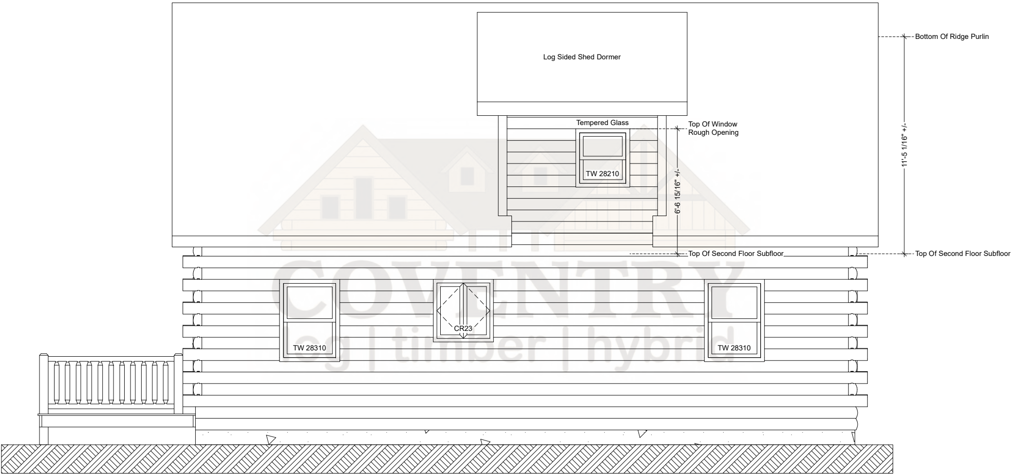
Alpine Right Elevation
