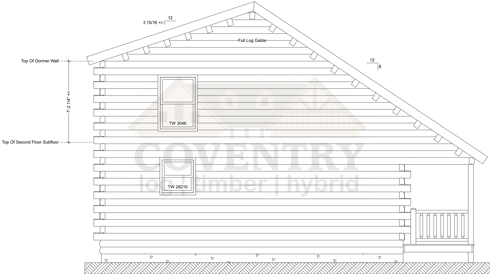
Andover Left Elevation
