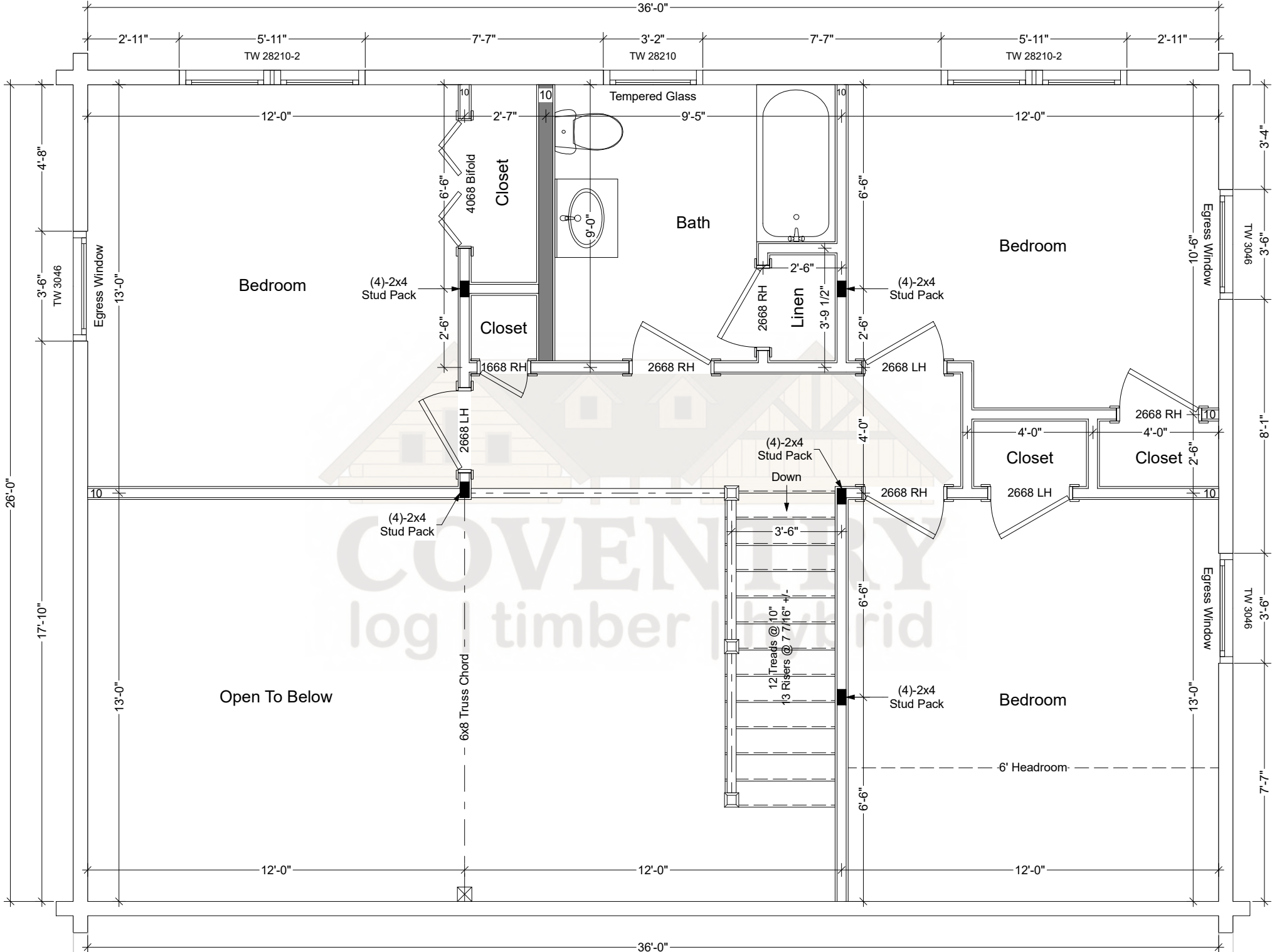
Andover Second Floor Plan
