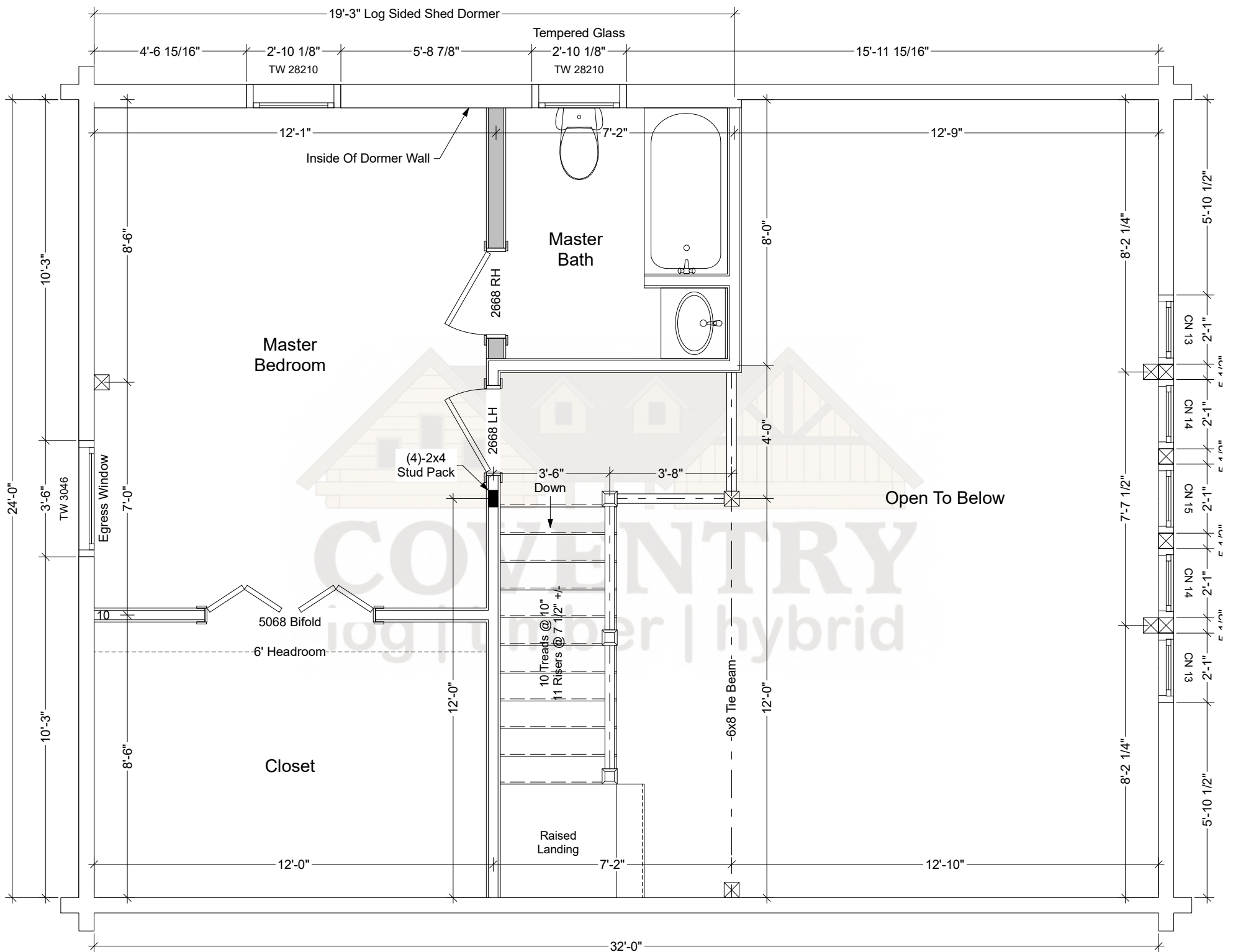
Ascutney Second Floor Plan
