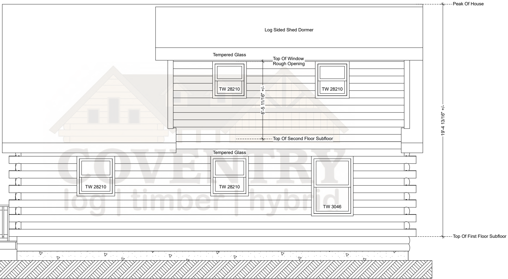
Ascutney Rear Elevation
