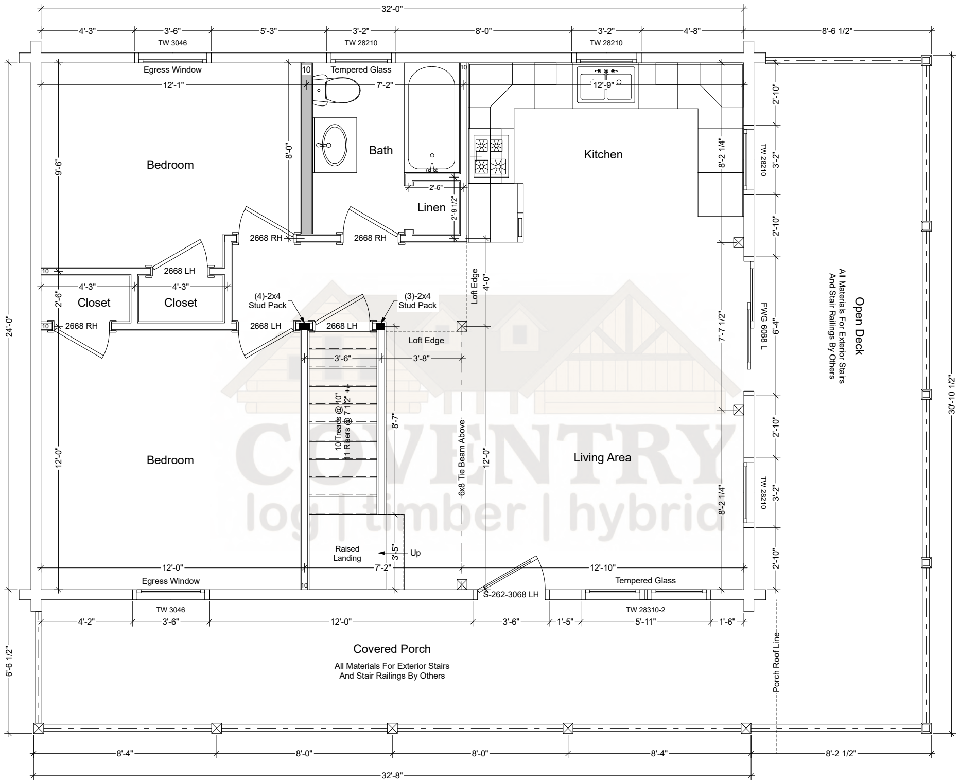
Ascutney First Floor Plan
