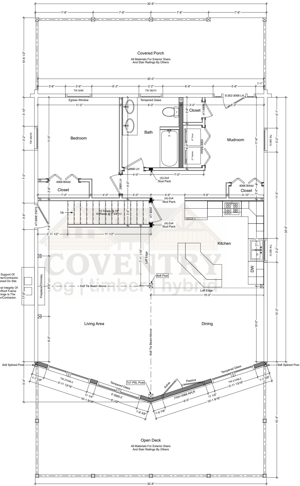
Aspen First Floor Plan
