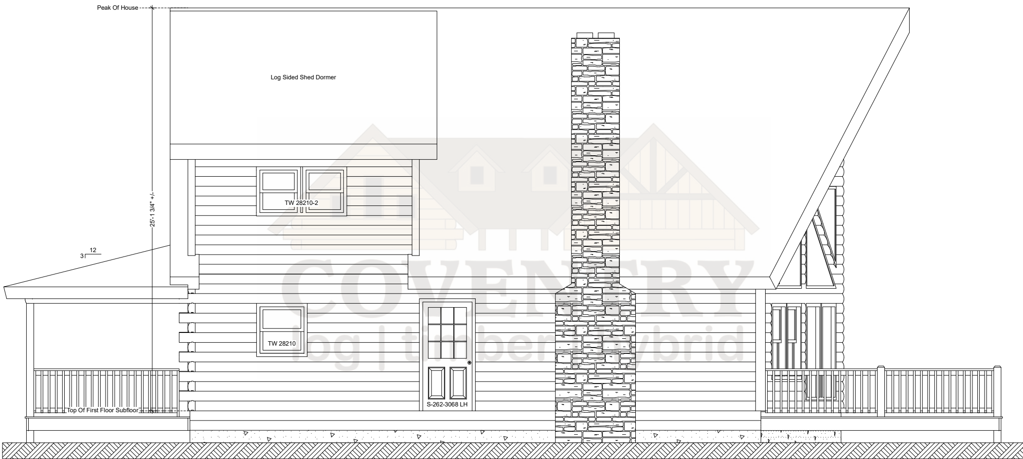
Aspen Left Elevation
