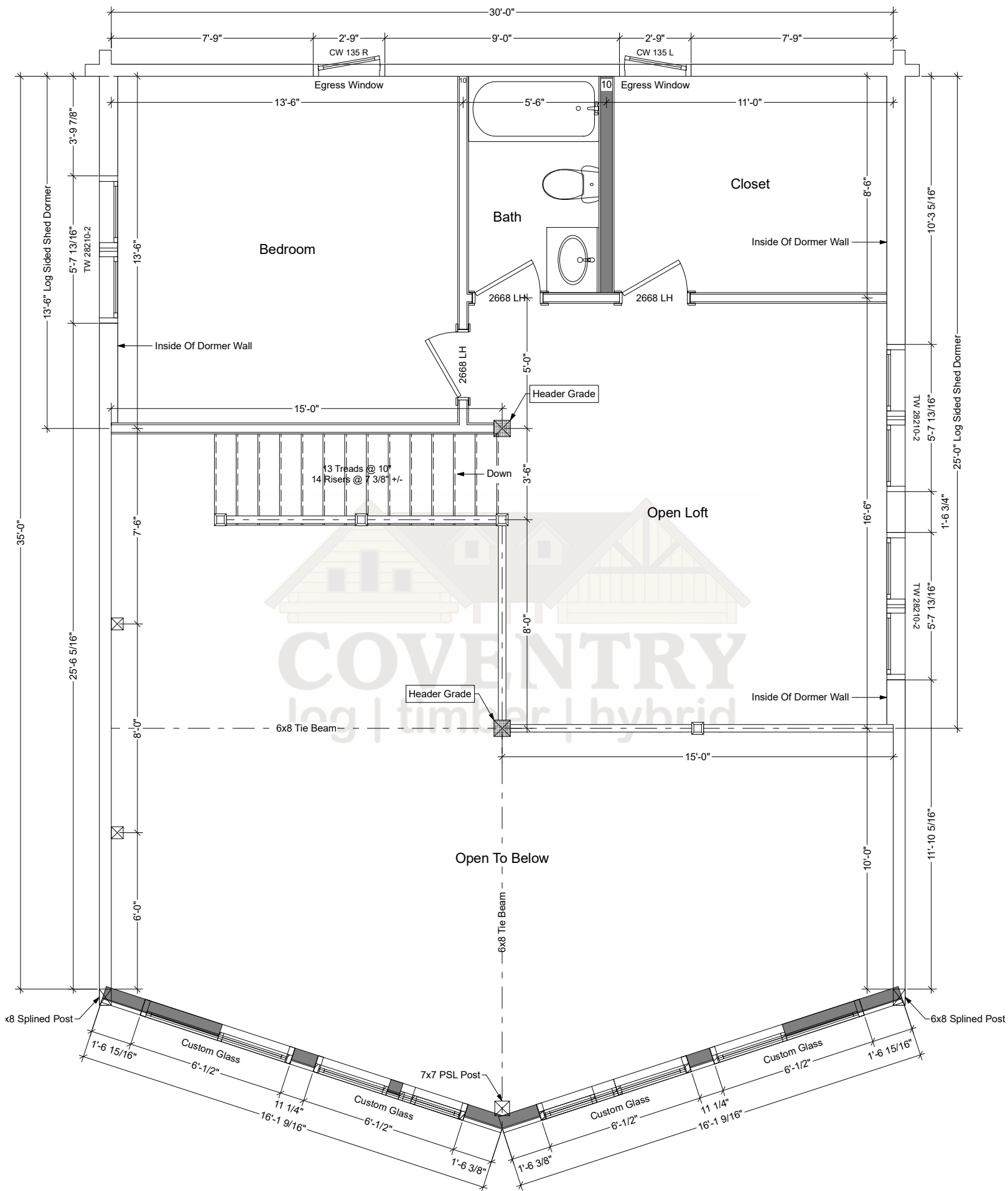
Aspen Second Floor Plan
