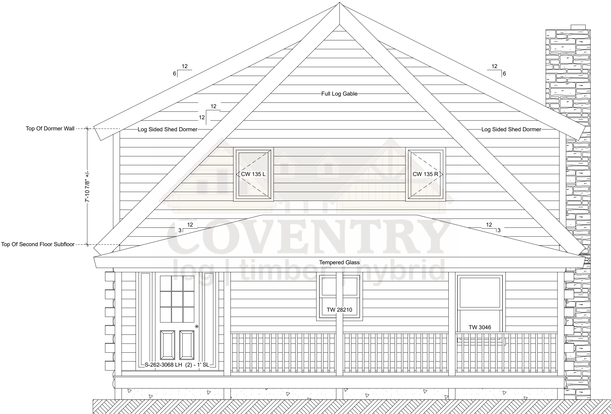
Aspen Rear Elevation
