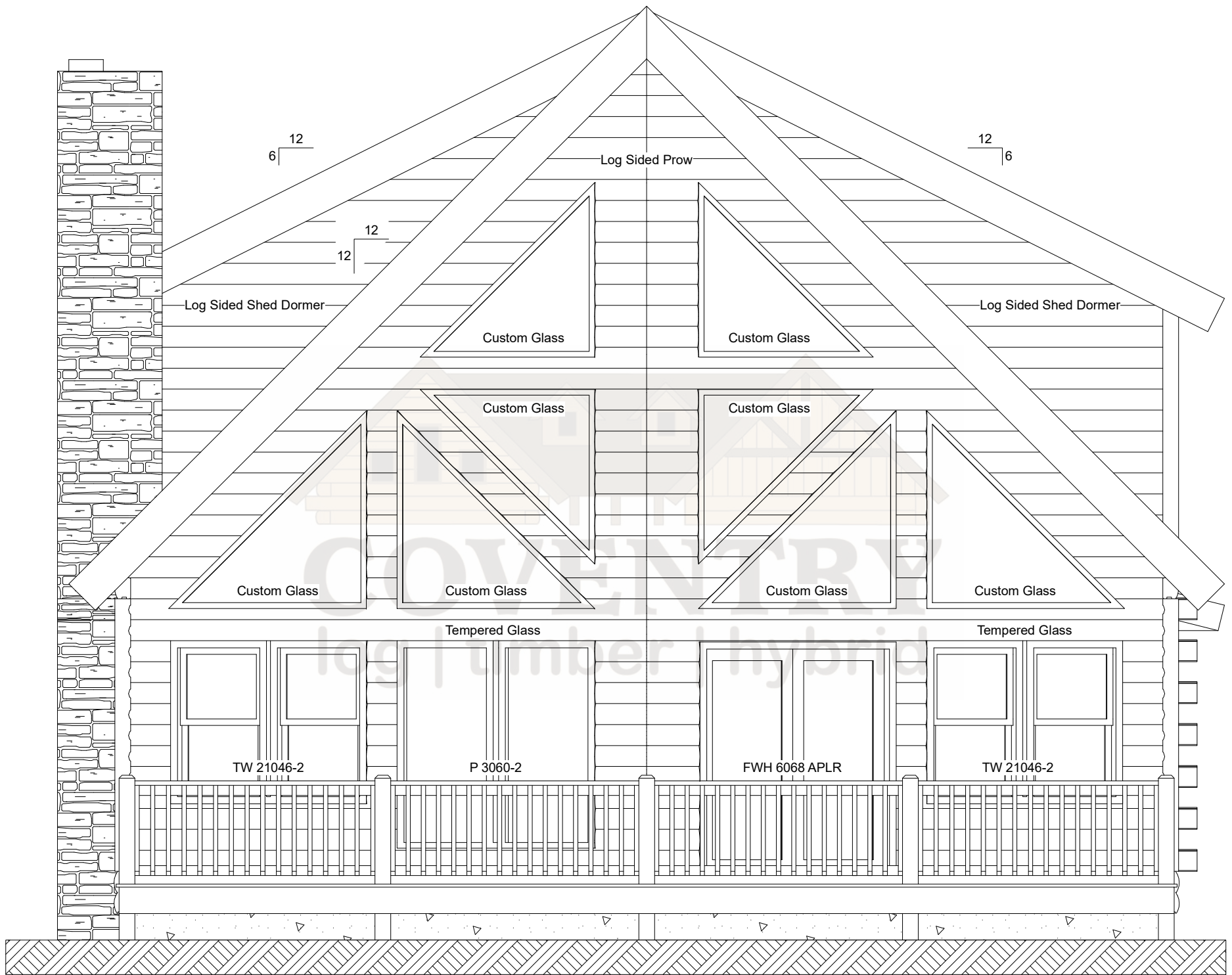
Aspen Front Elevation
