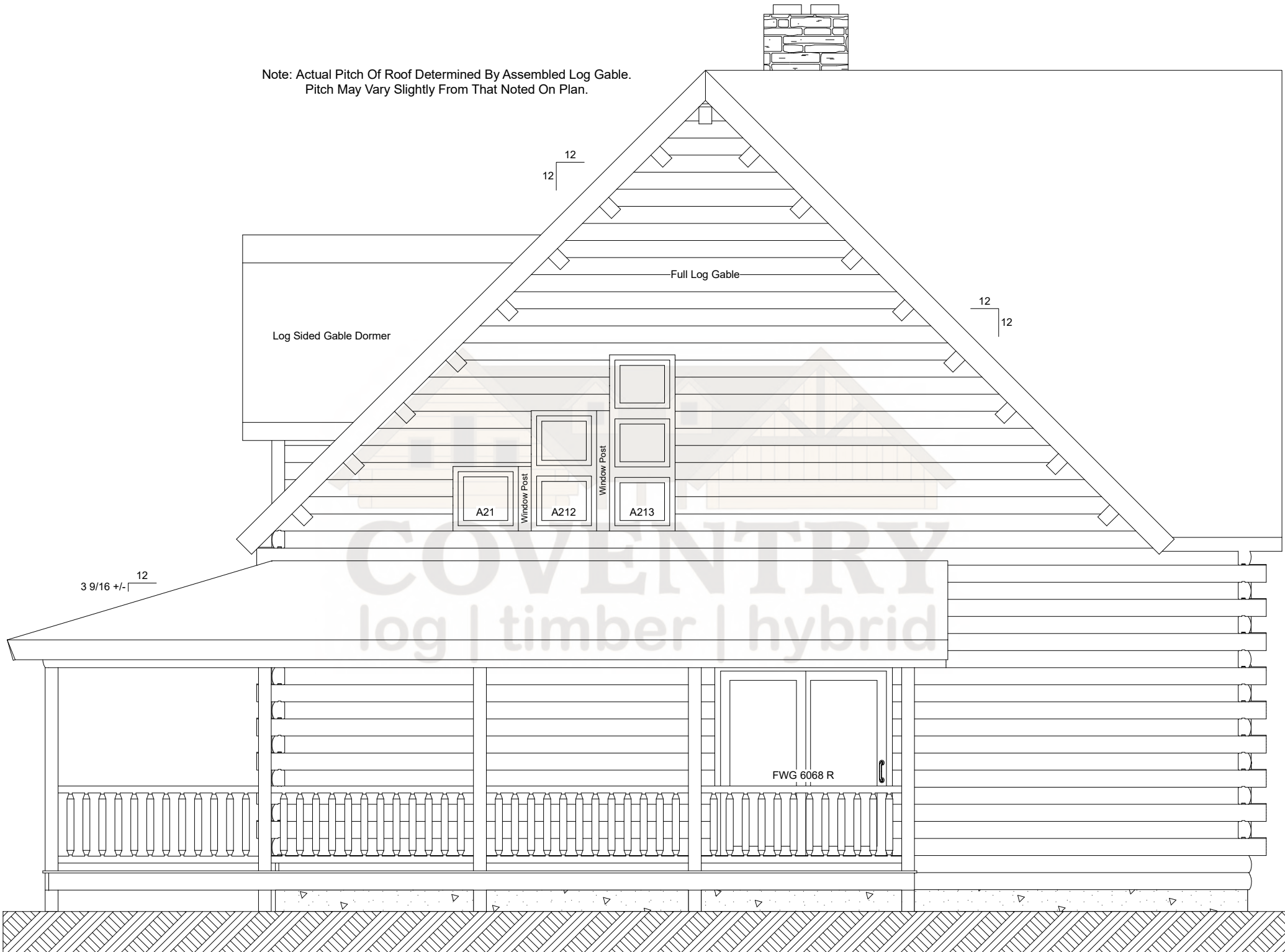
Athens Right Elevation
