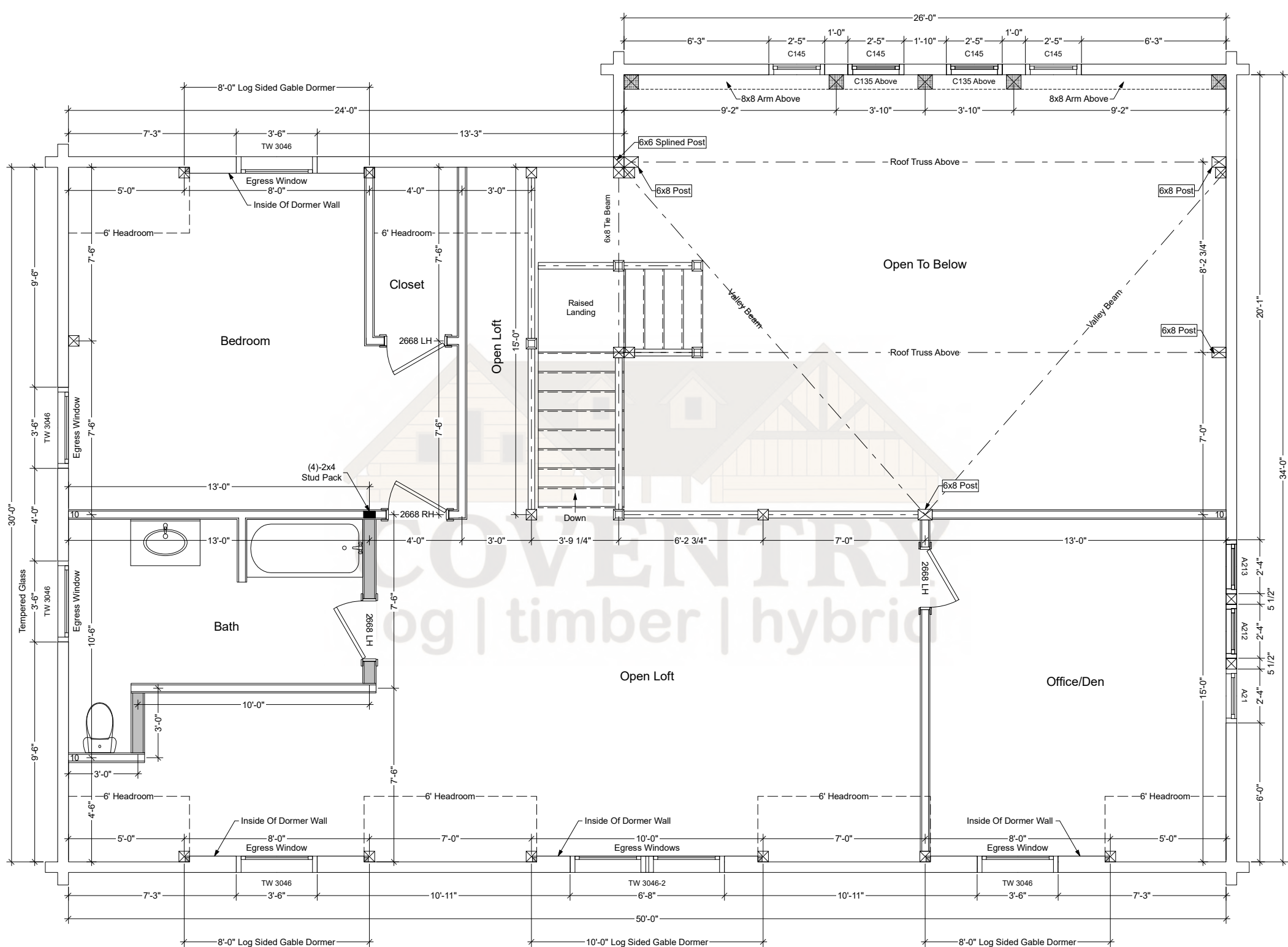
Athens Second Floor Plan
