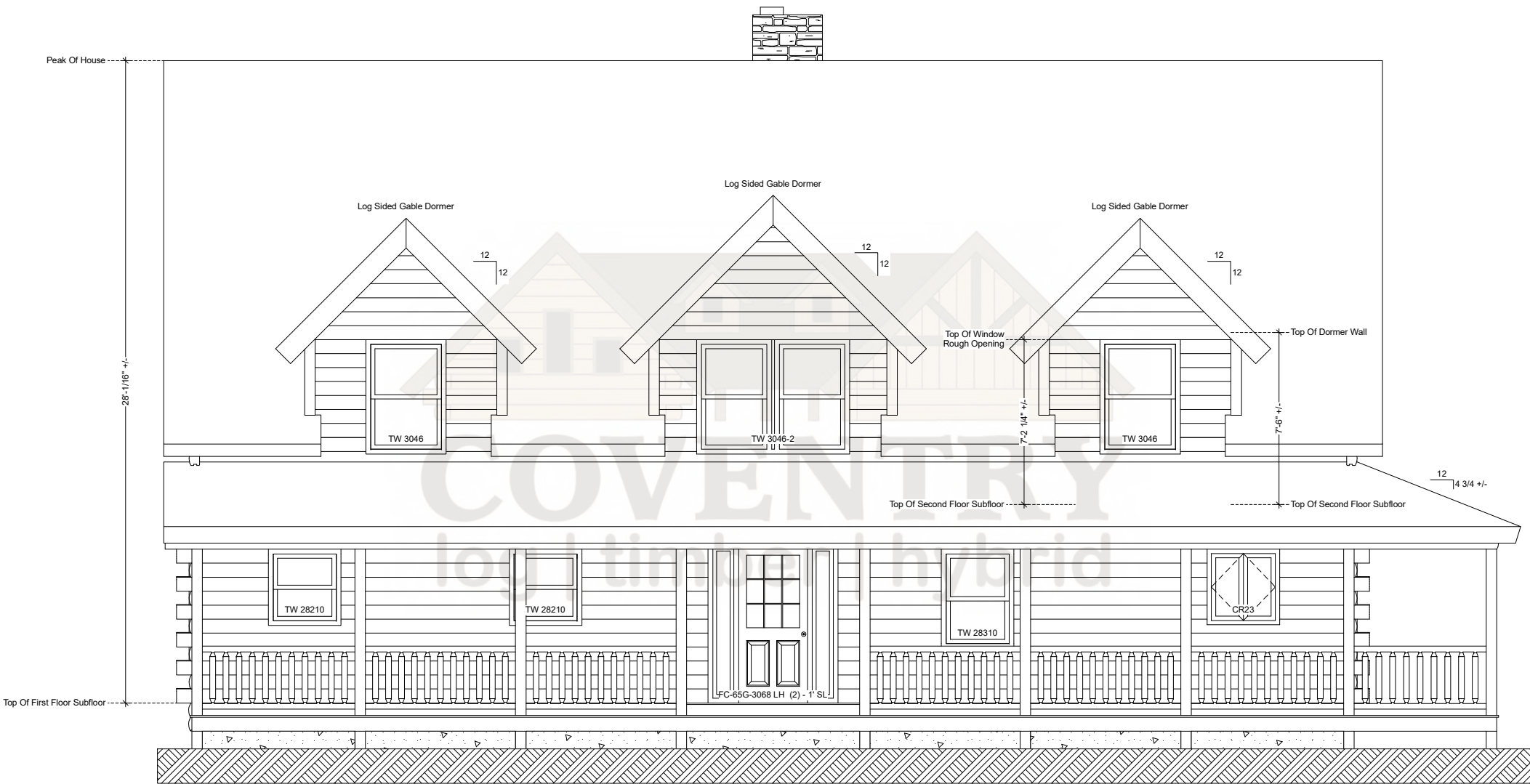
Athens Front Elevation
