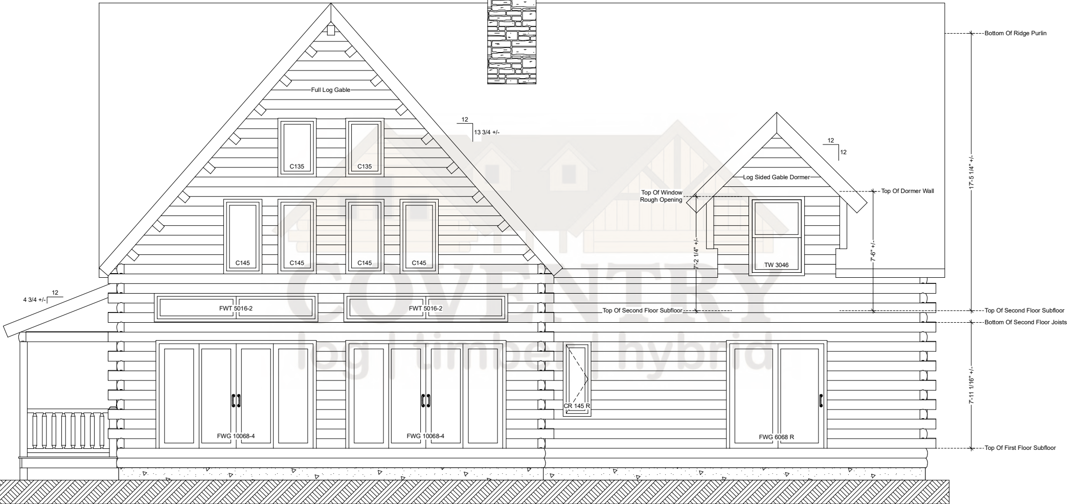
Athens Rear Elevation
