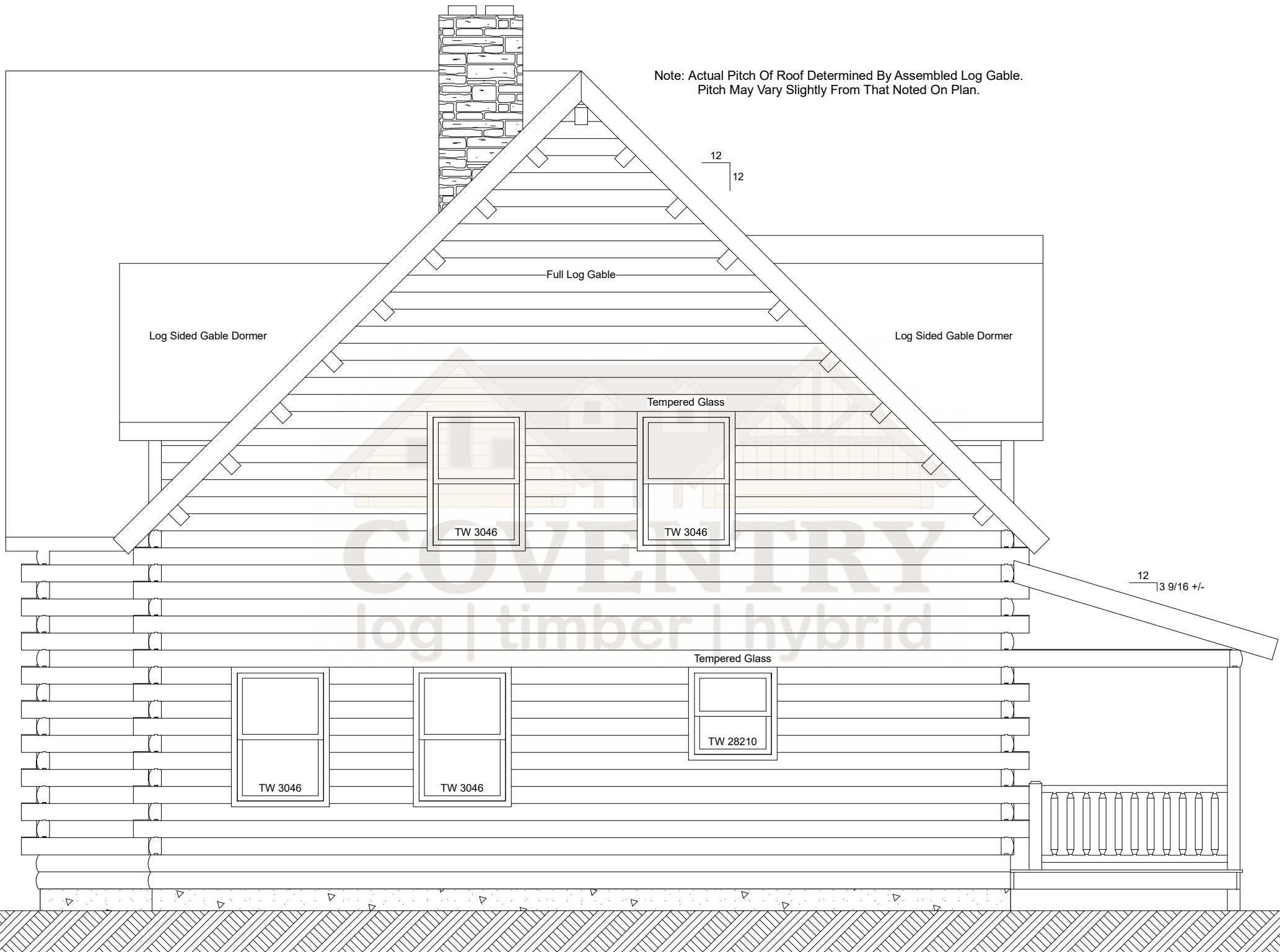
Athens Left Elevation
