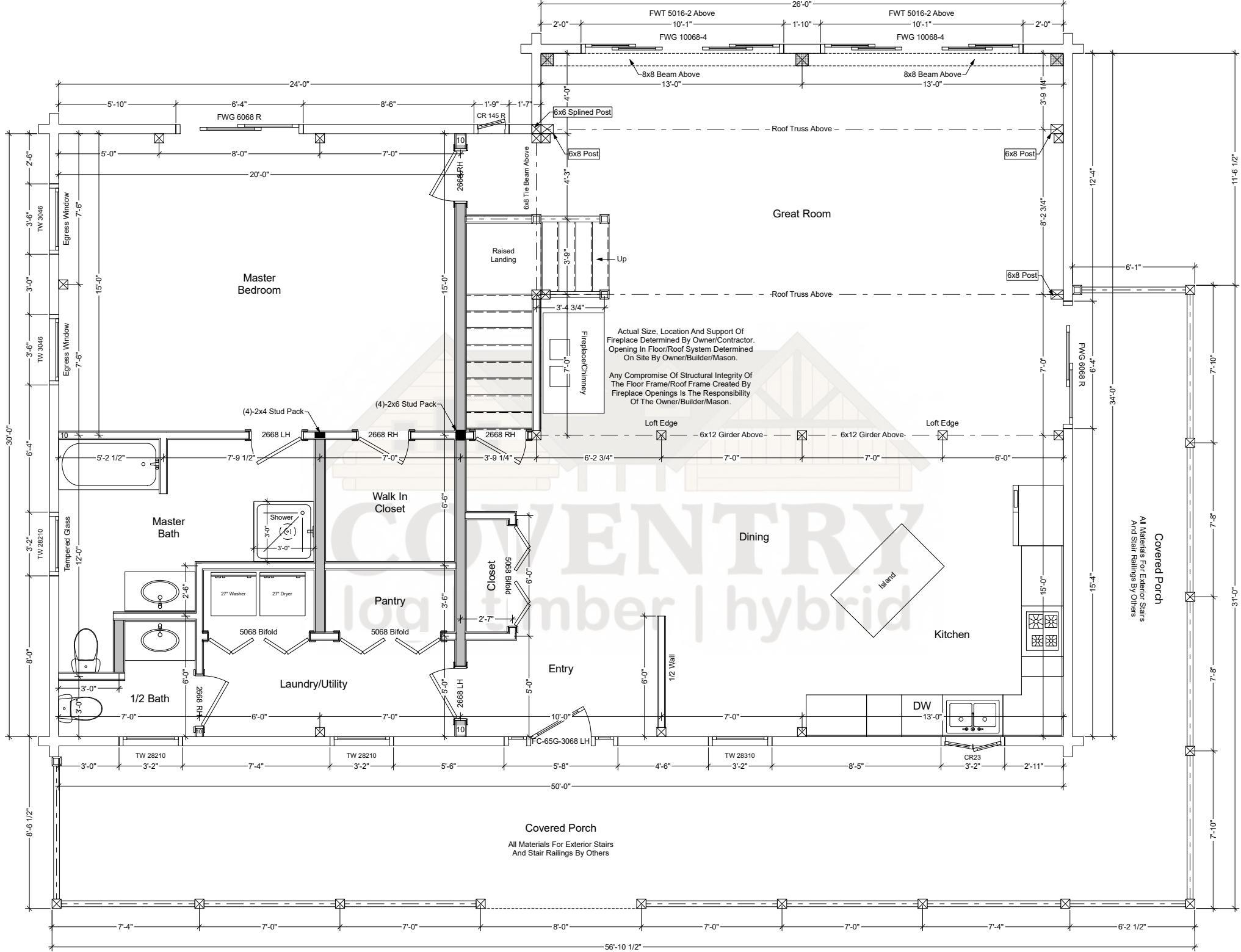
Athens First Floor Plan
