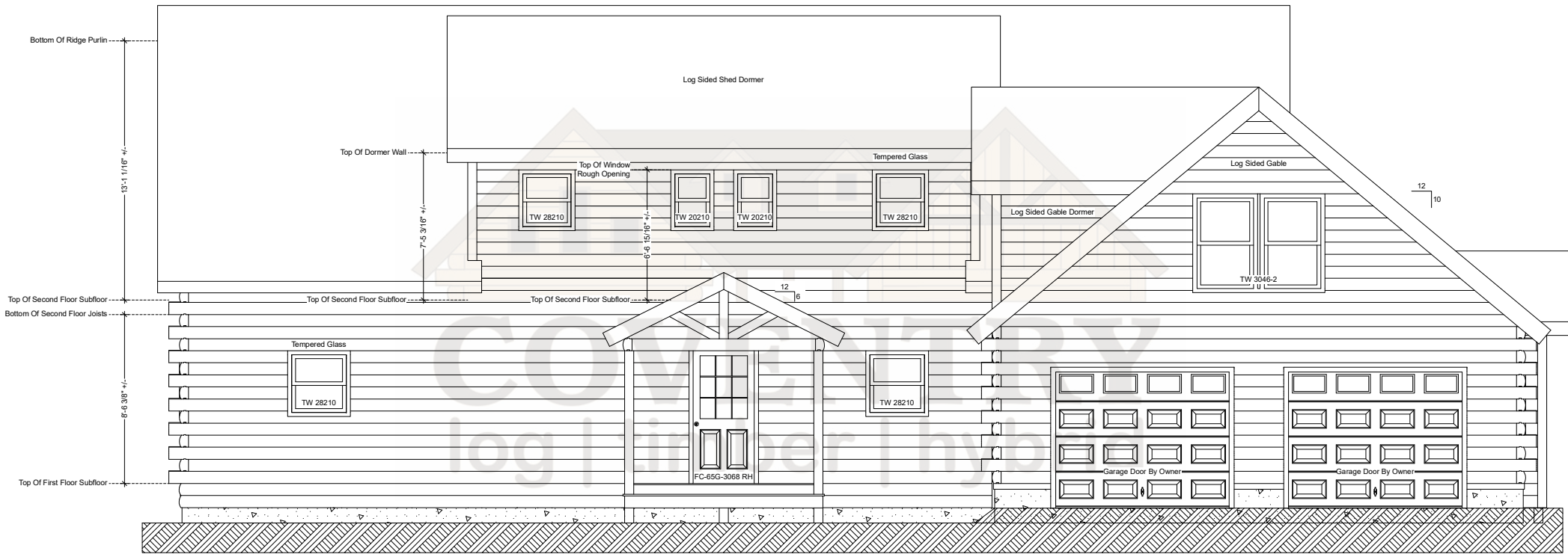
Bayview Front Elevation
