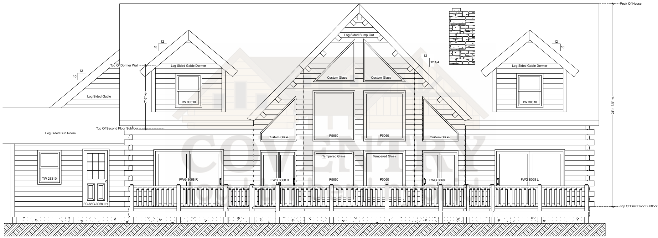
Bayview Rear Elevation
