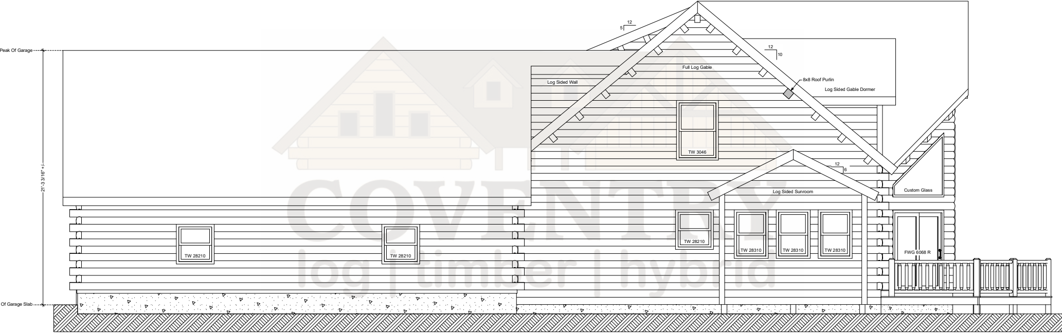
Bayview Right Elevation
