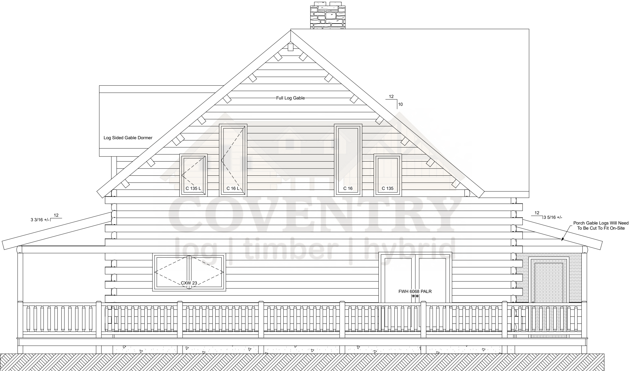
Bear Rock Right Elevation
