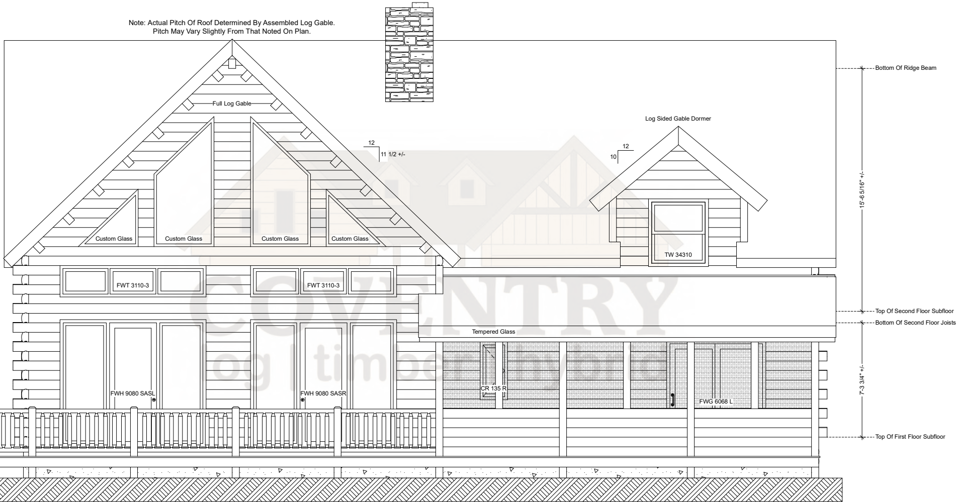
Bear Rock Rear Elevation
