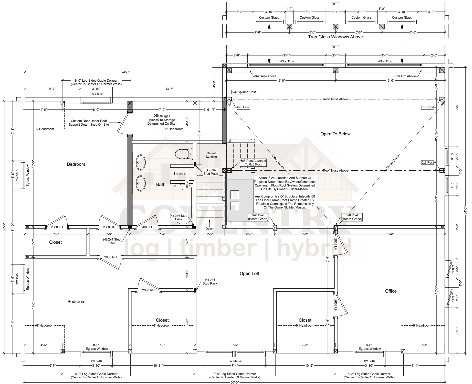
Bear Rock Second Floor Plan
