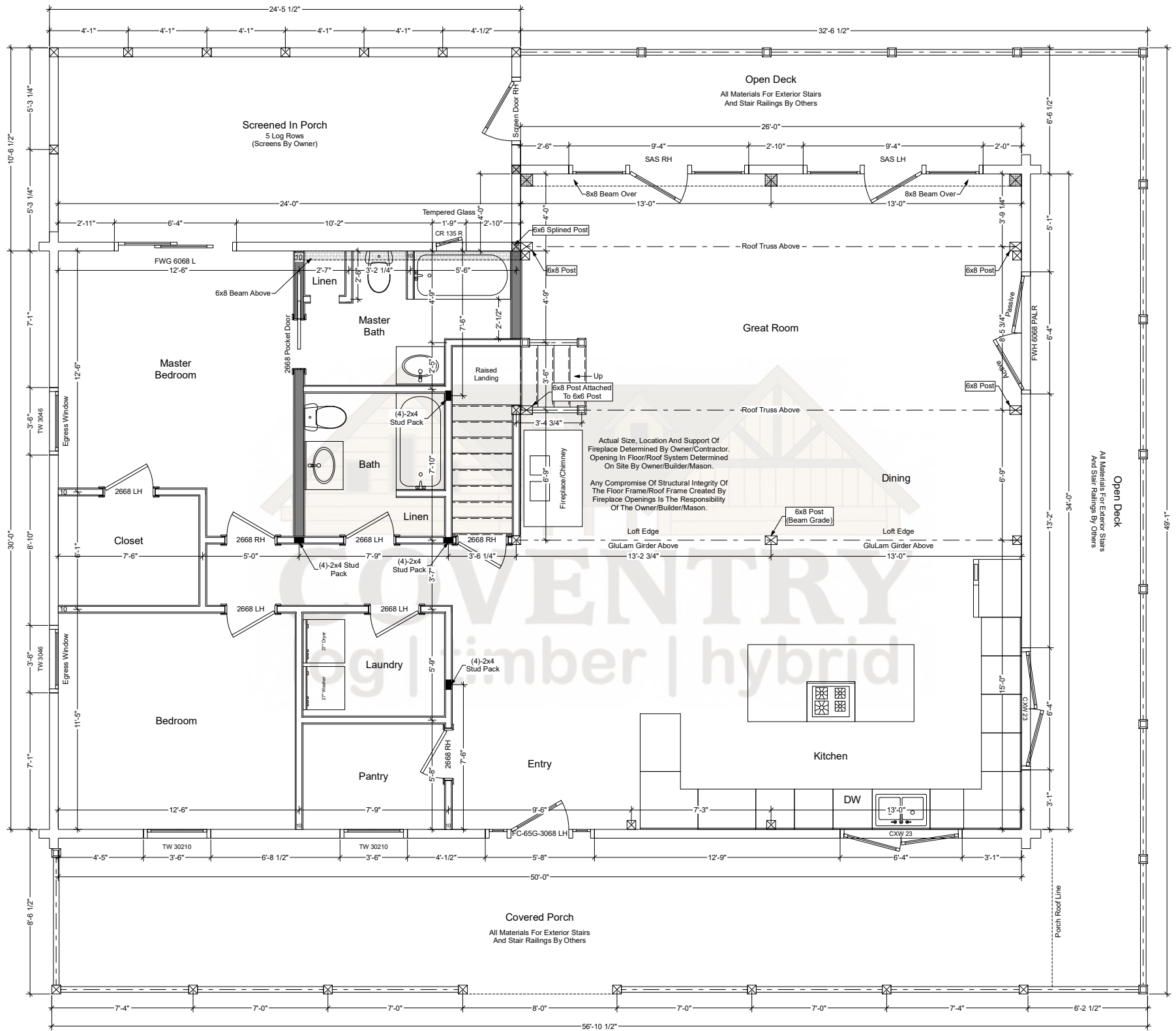
Bear Rock First Floor Plan
