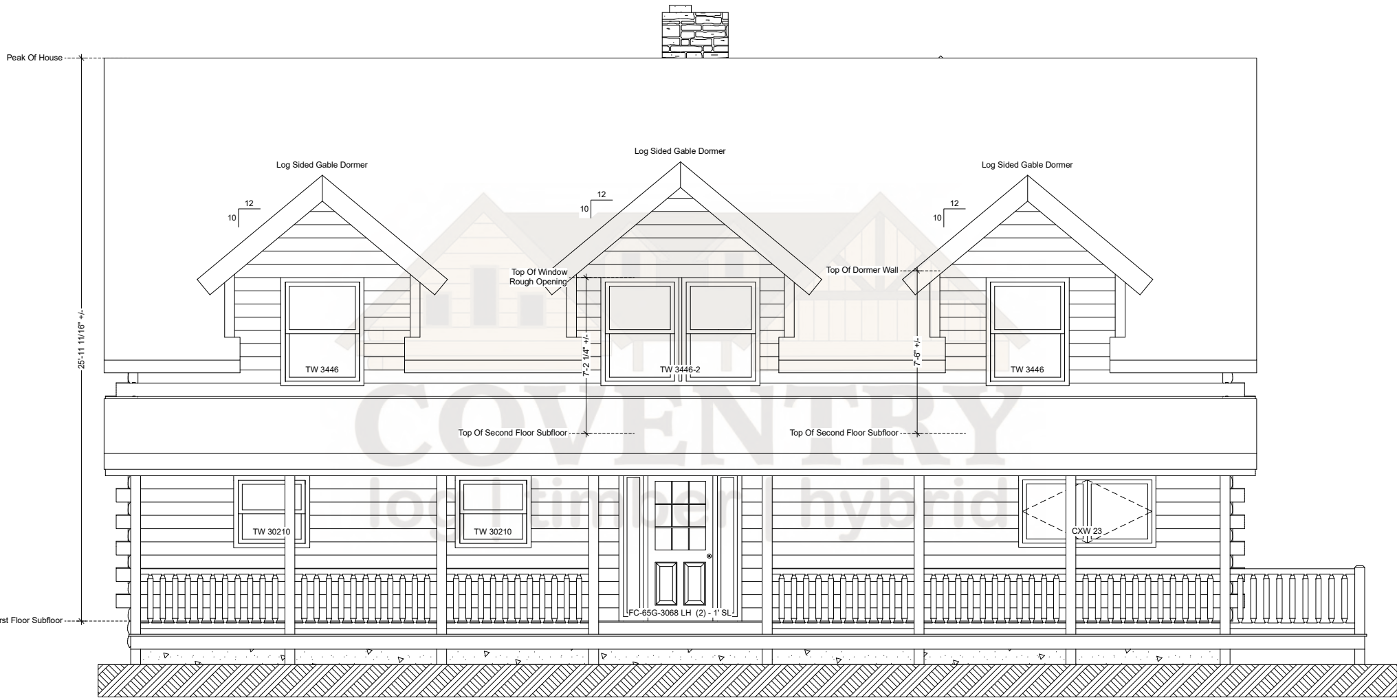
Bear Rock Front Elevation
