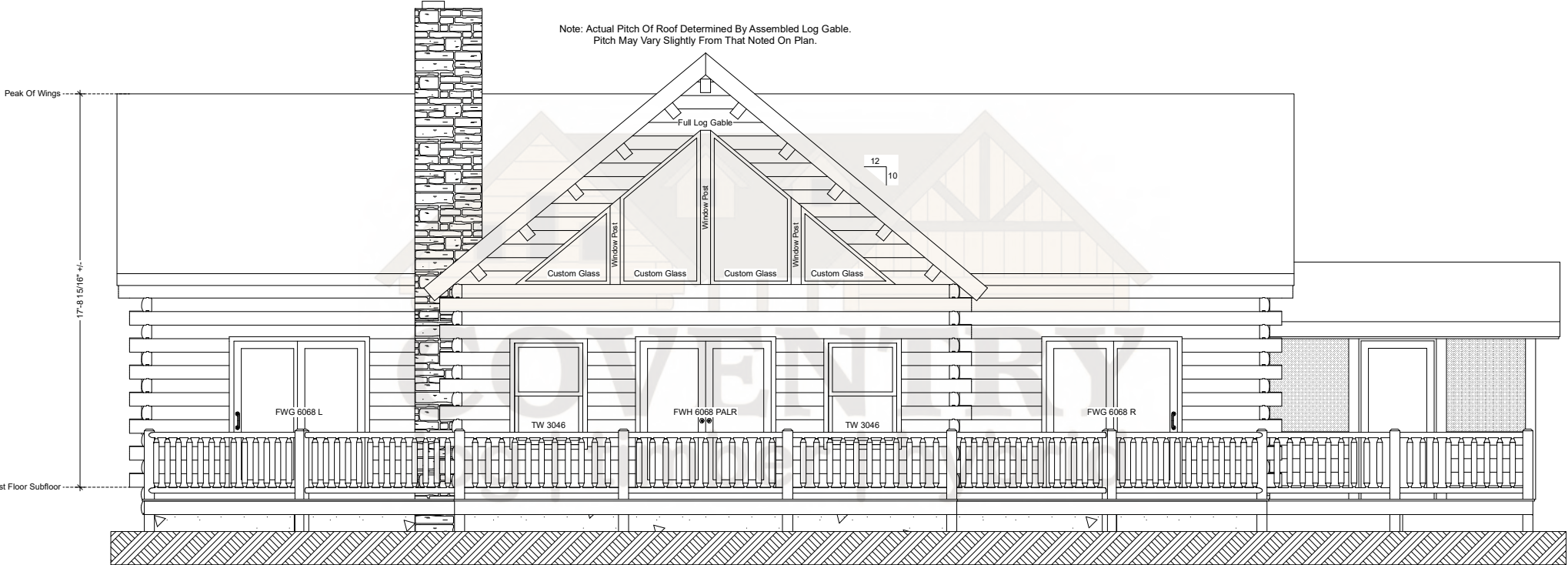
Big Sky Front Elevation
