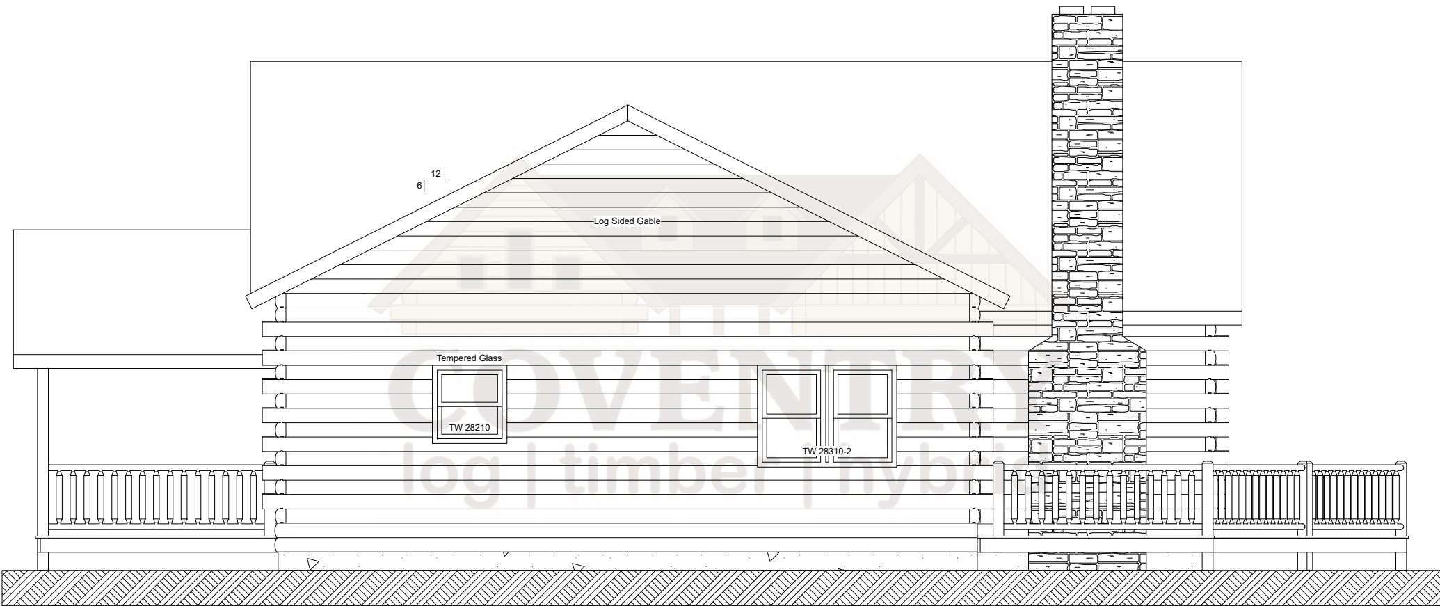
Big Sky Left Elevation
