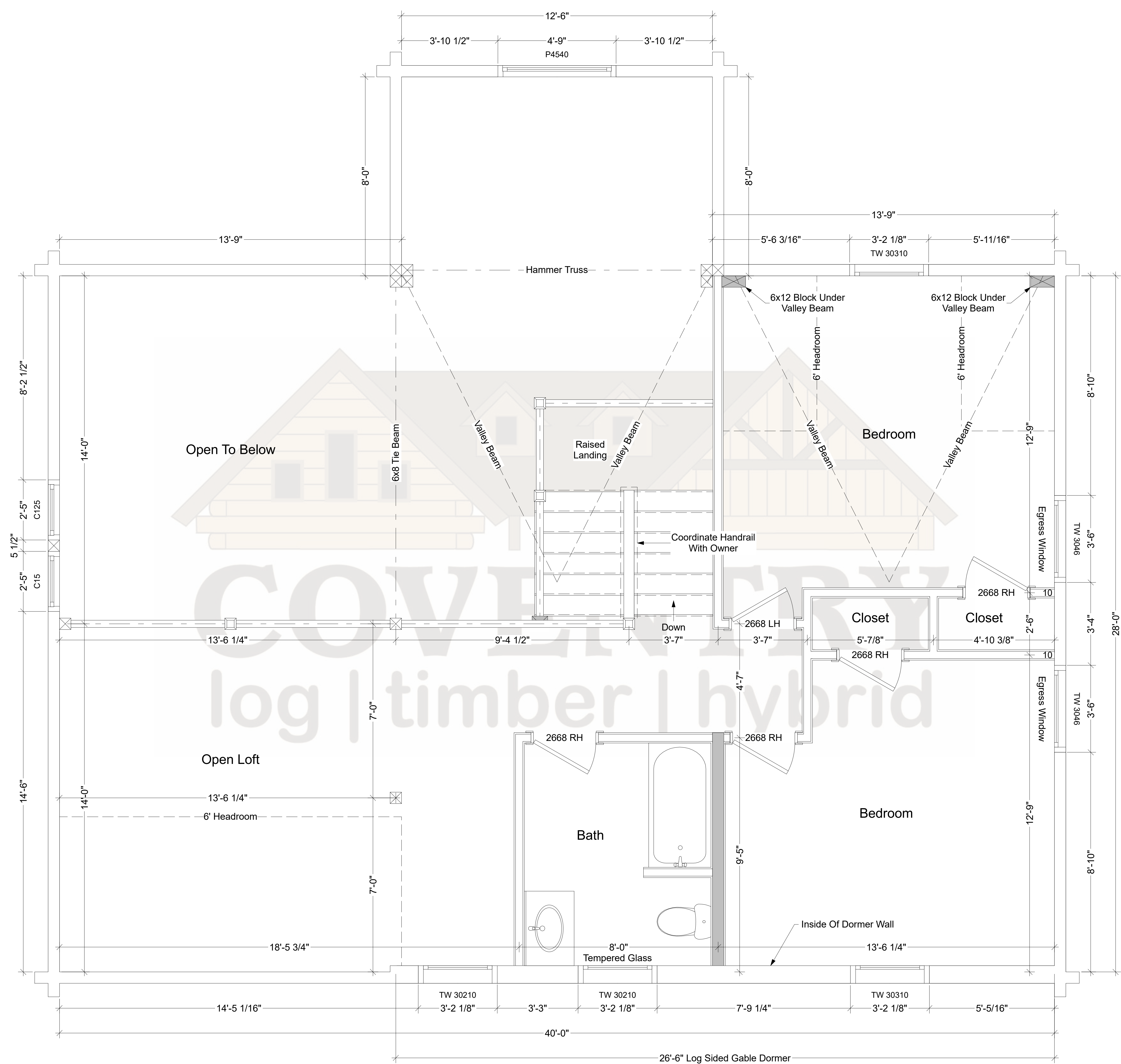
Birchwood Second Floor Plan
