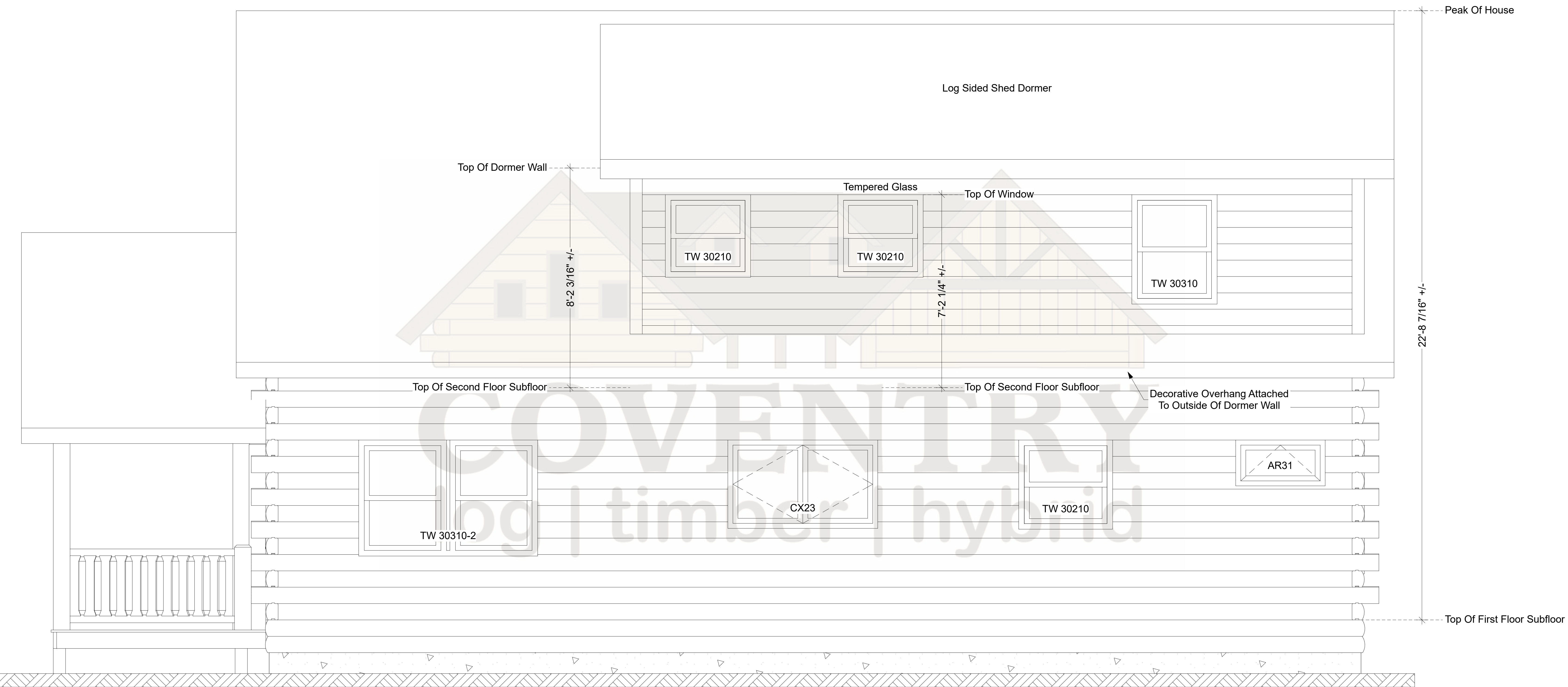
Birchwood Front Elevation
