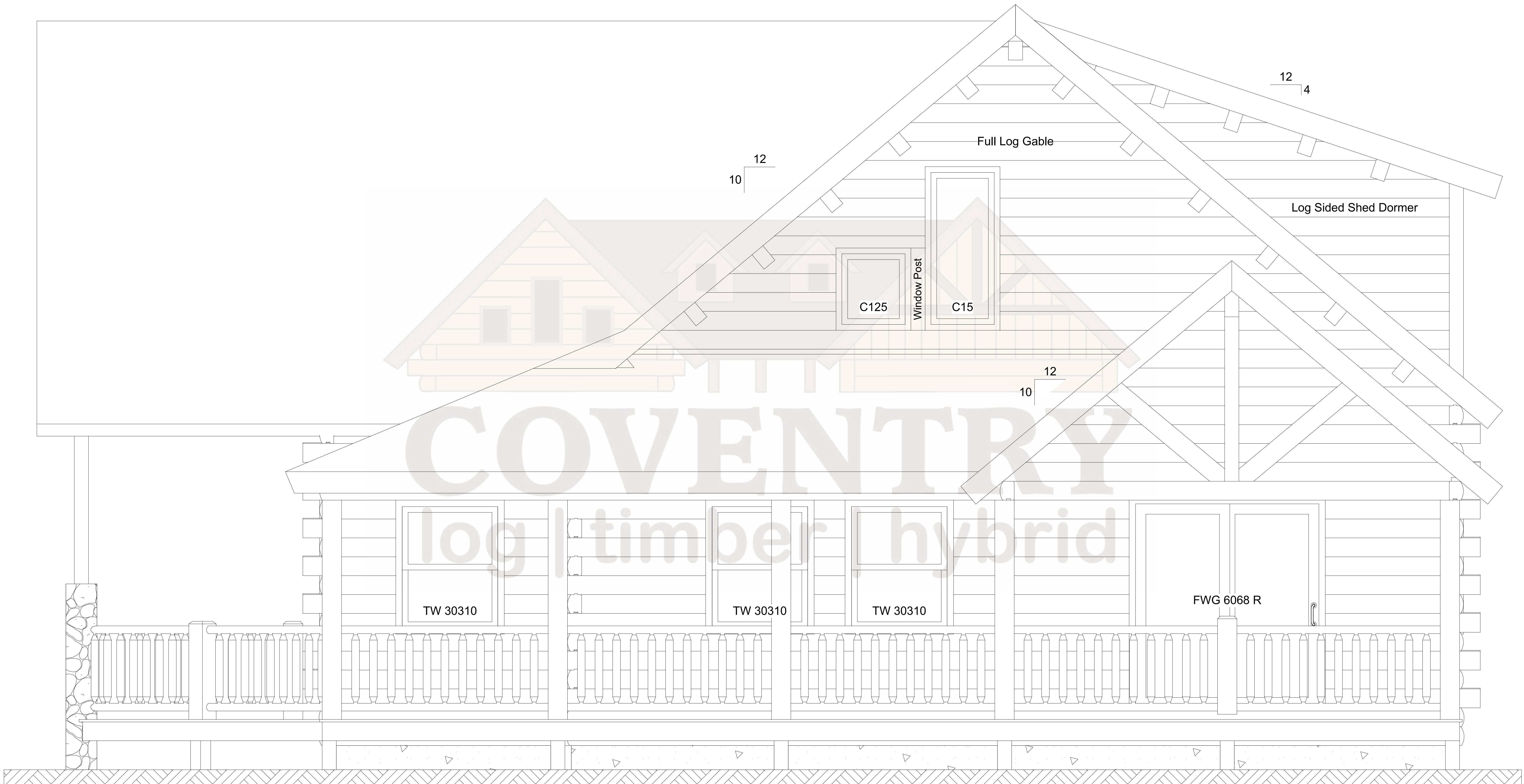
Birchwood Left Elevation
