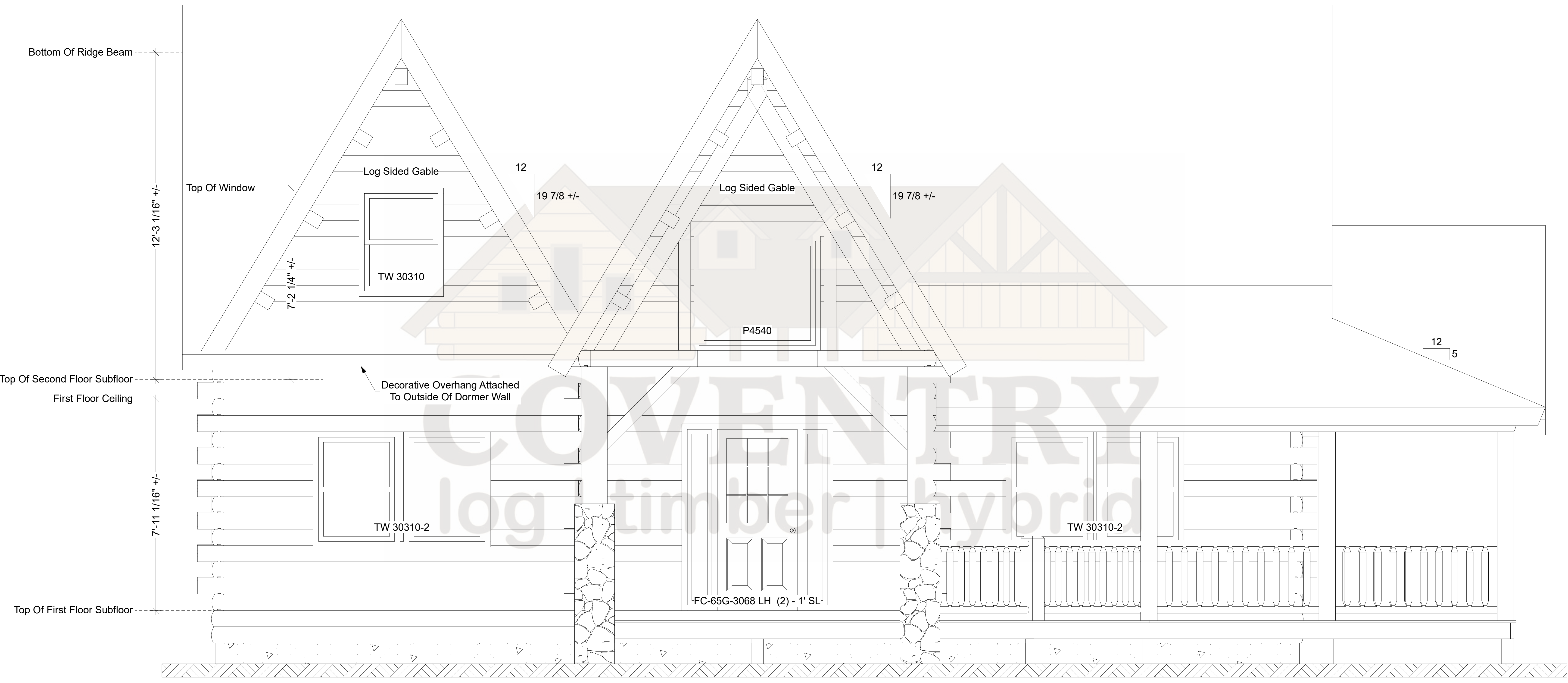
Birchwood Rear Elevation
