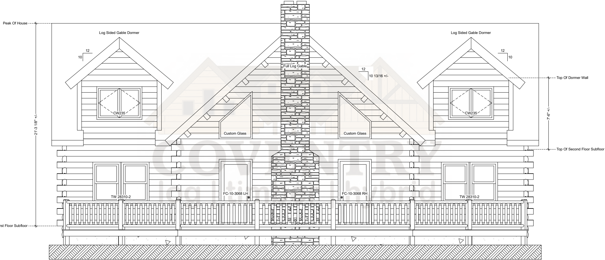
Brentwood Front Elevation
