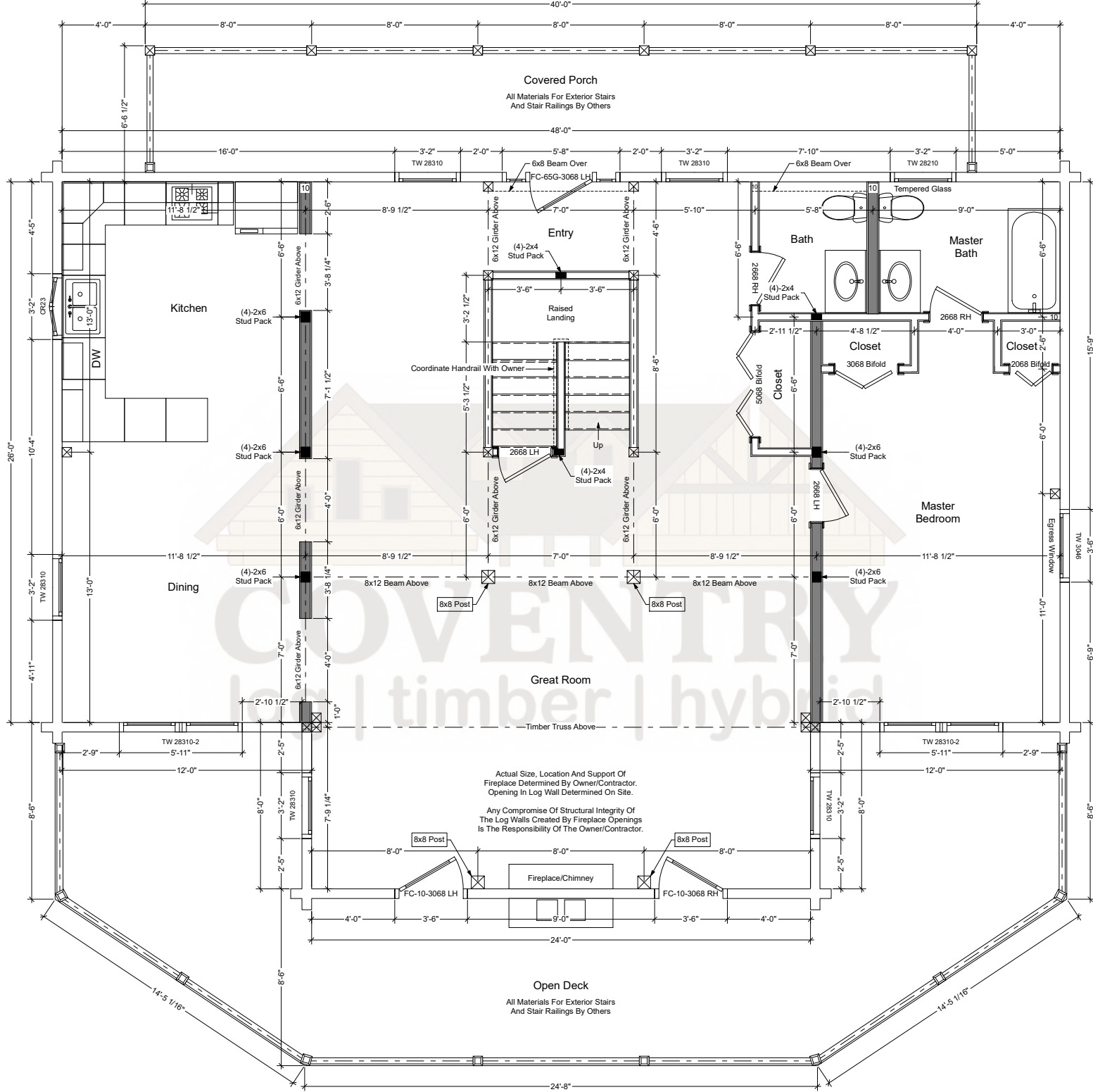
Brentwood First Floor Plan
