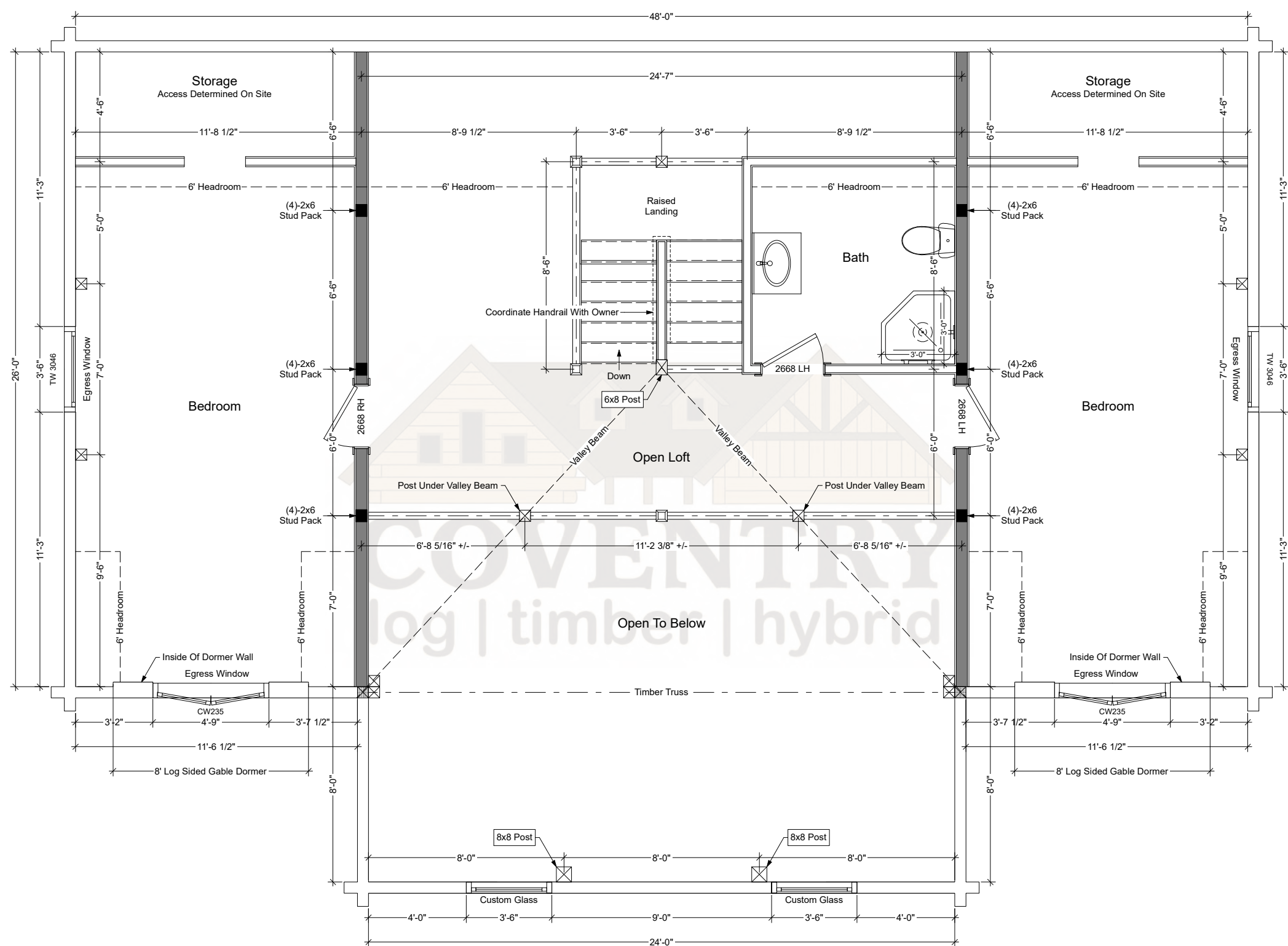
Brentwood Second Floor Plan
