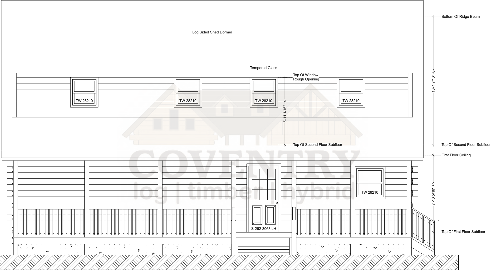
Cascade Front Elevation
