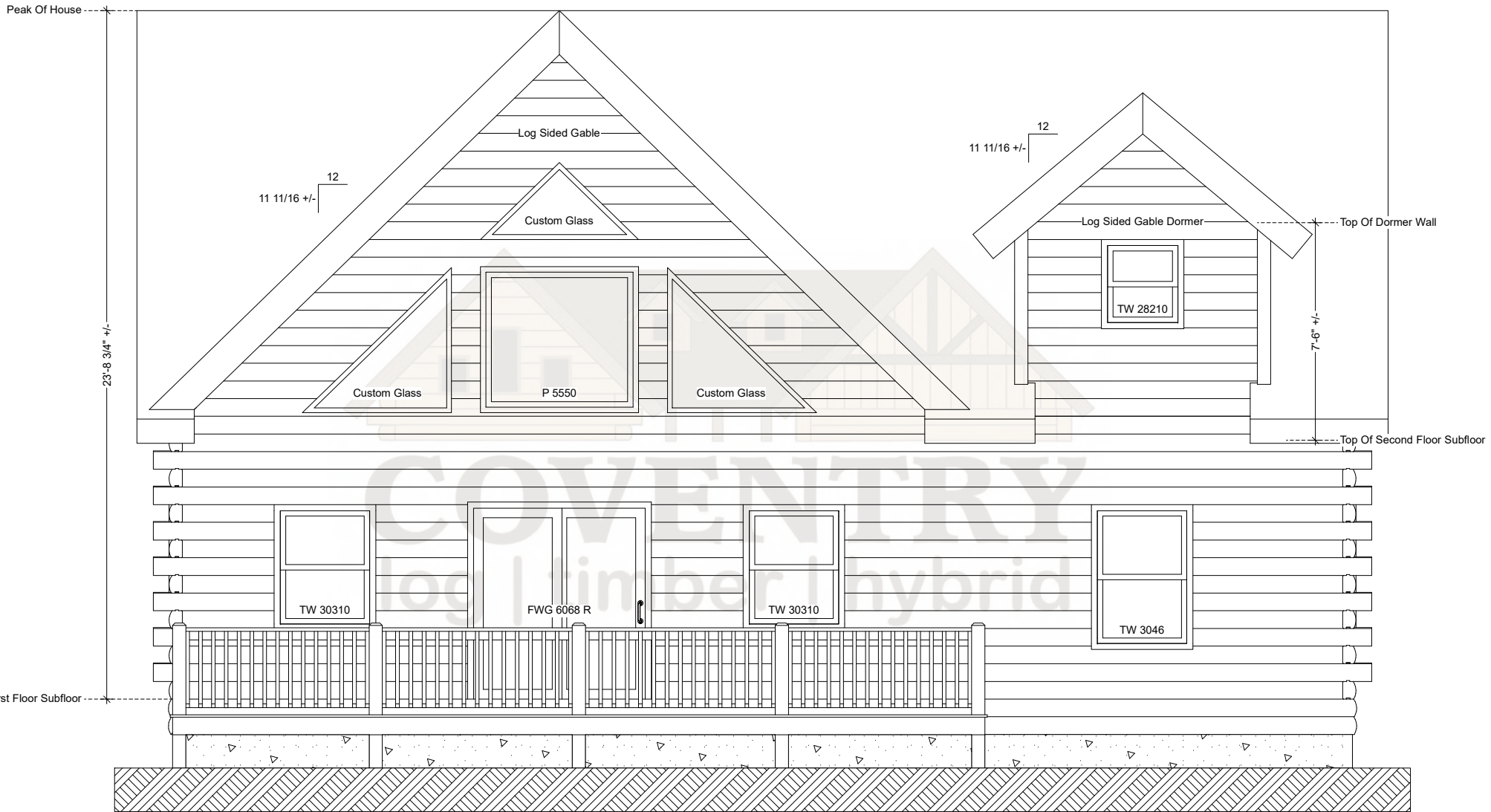
Cascade Rear Elevation
