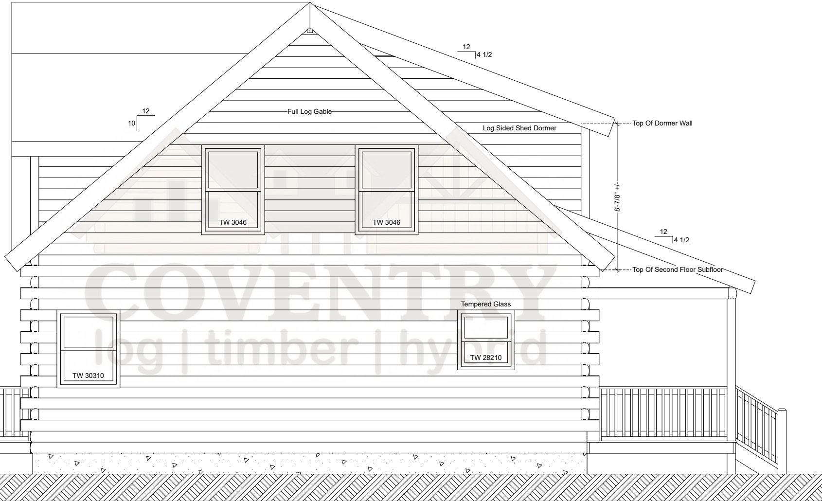
Cascade Left Elevation
