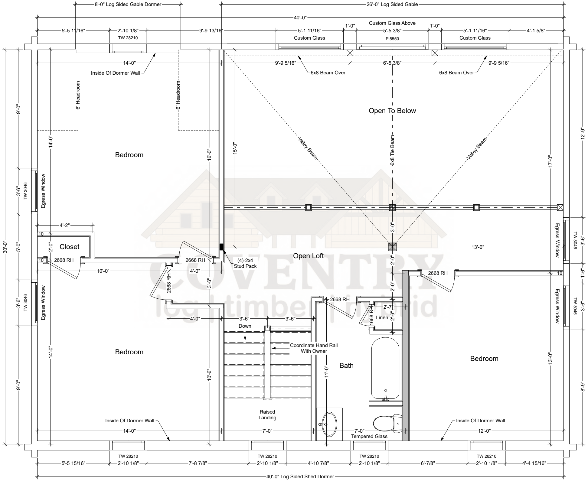
Cascade Second Floor Plan
