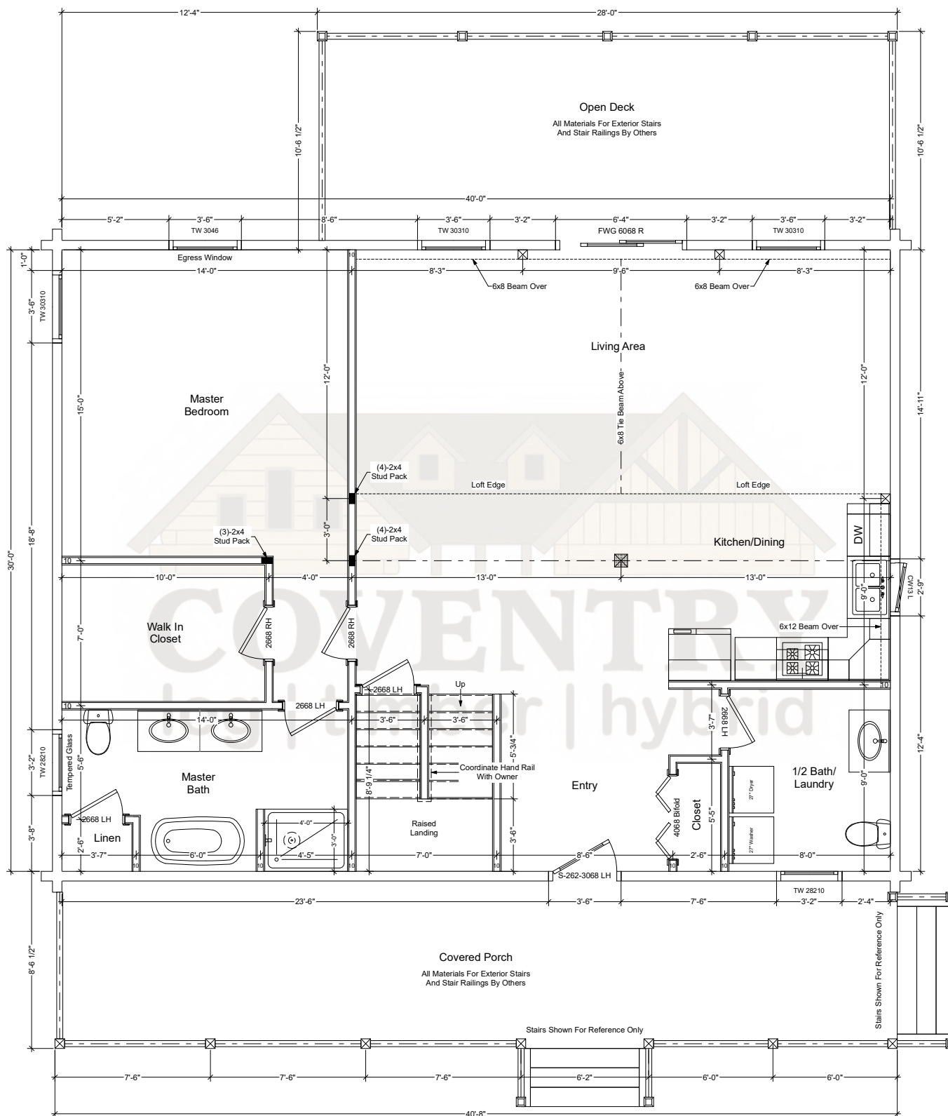
Cascade First Floor Plan
