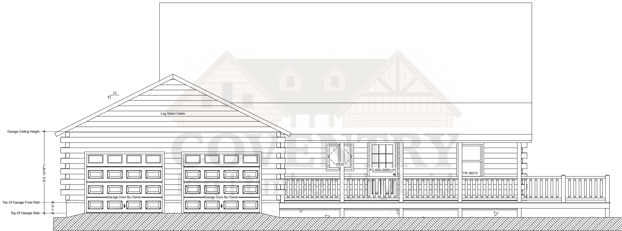
Cheyenne Left Elevation
