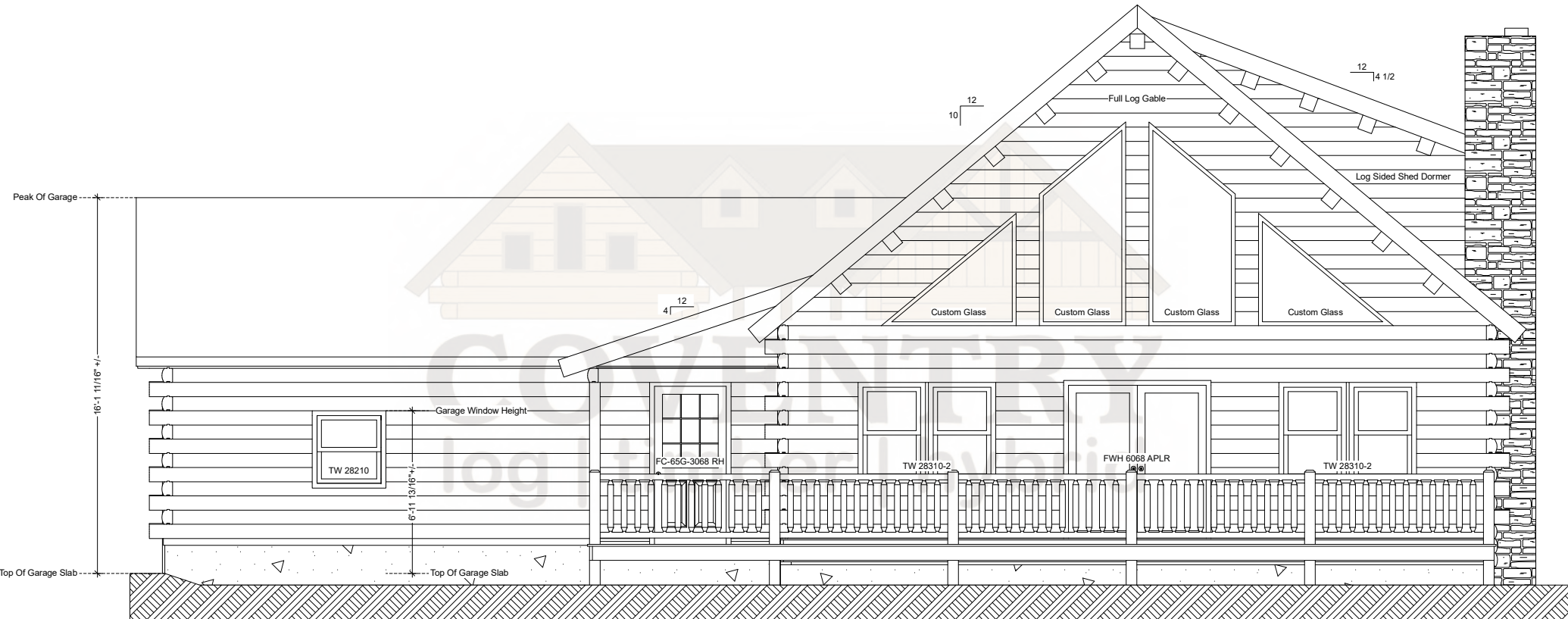
Cheyenne Front Elevation
