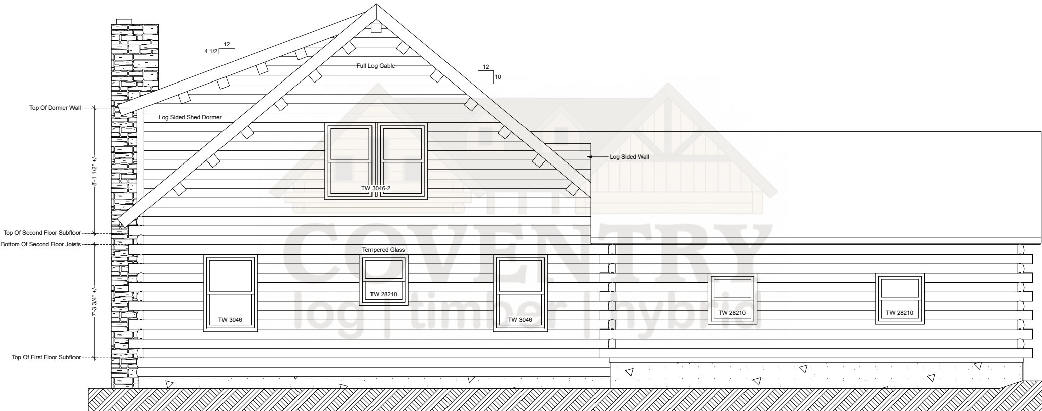
Cheyenne Rear Elevation
