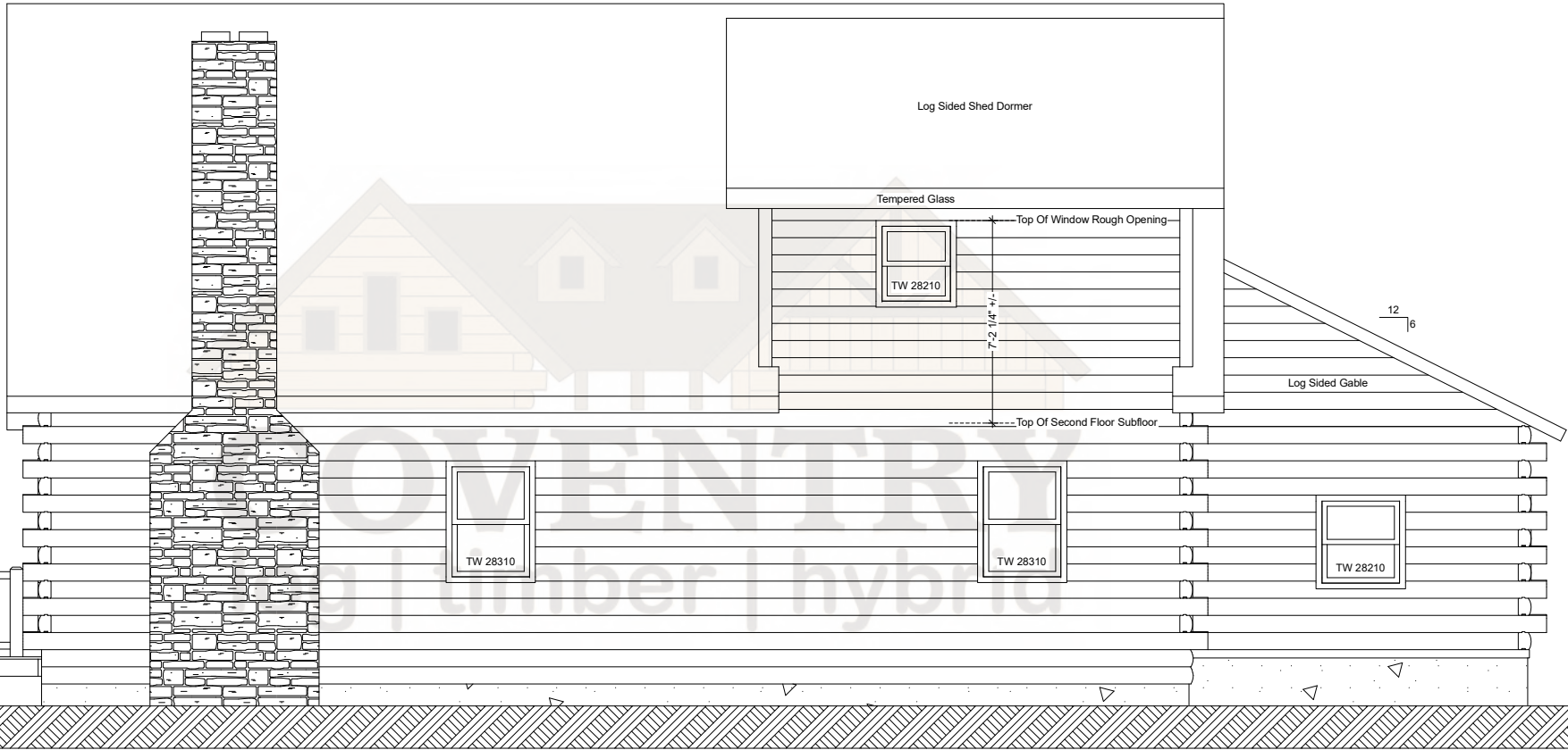
Cheyenne Right Elevation
