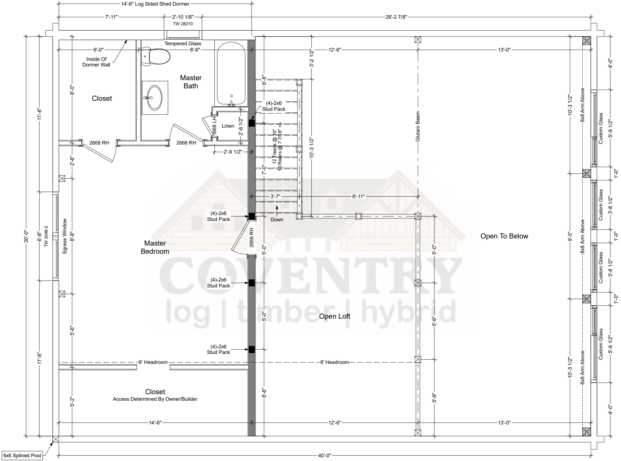
Cheyenne Second Floor Plan
