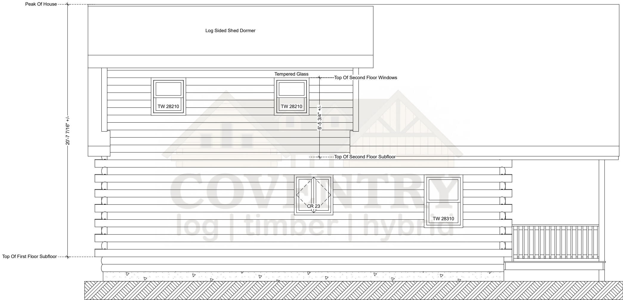
Driftwood Rear Elevation
