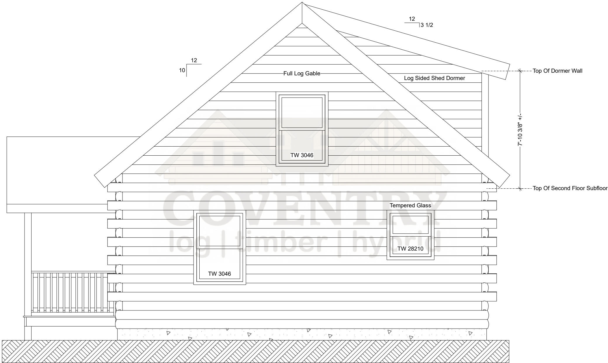
Driftwood Right Elevation
