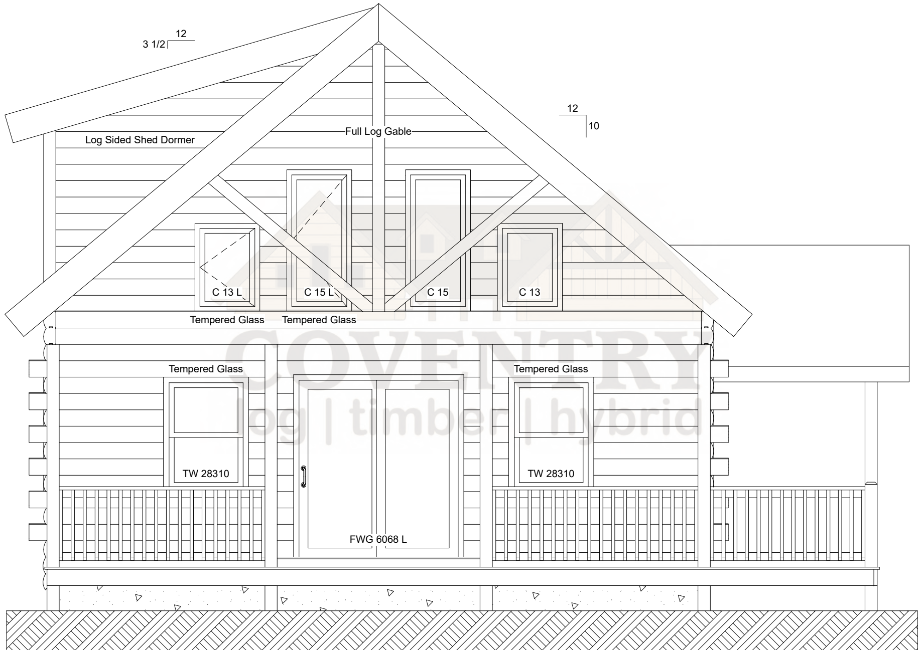
Driftwood Left Elevation
