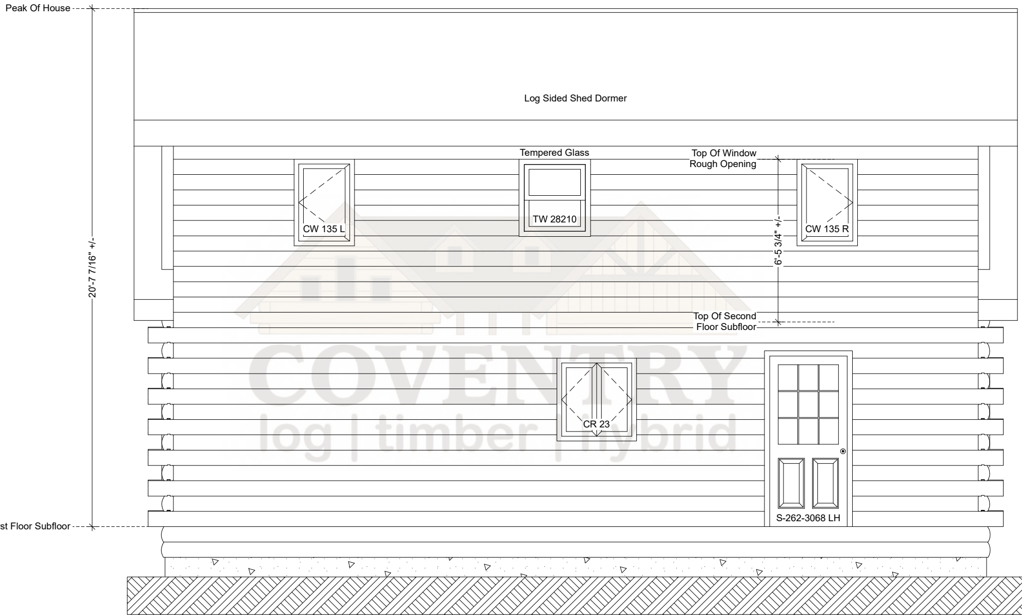
Fairfield Rear Elevation
