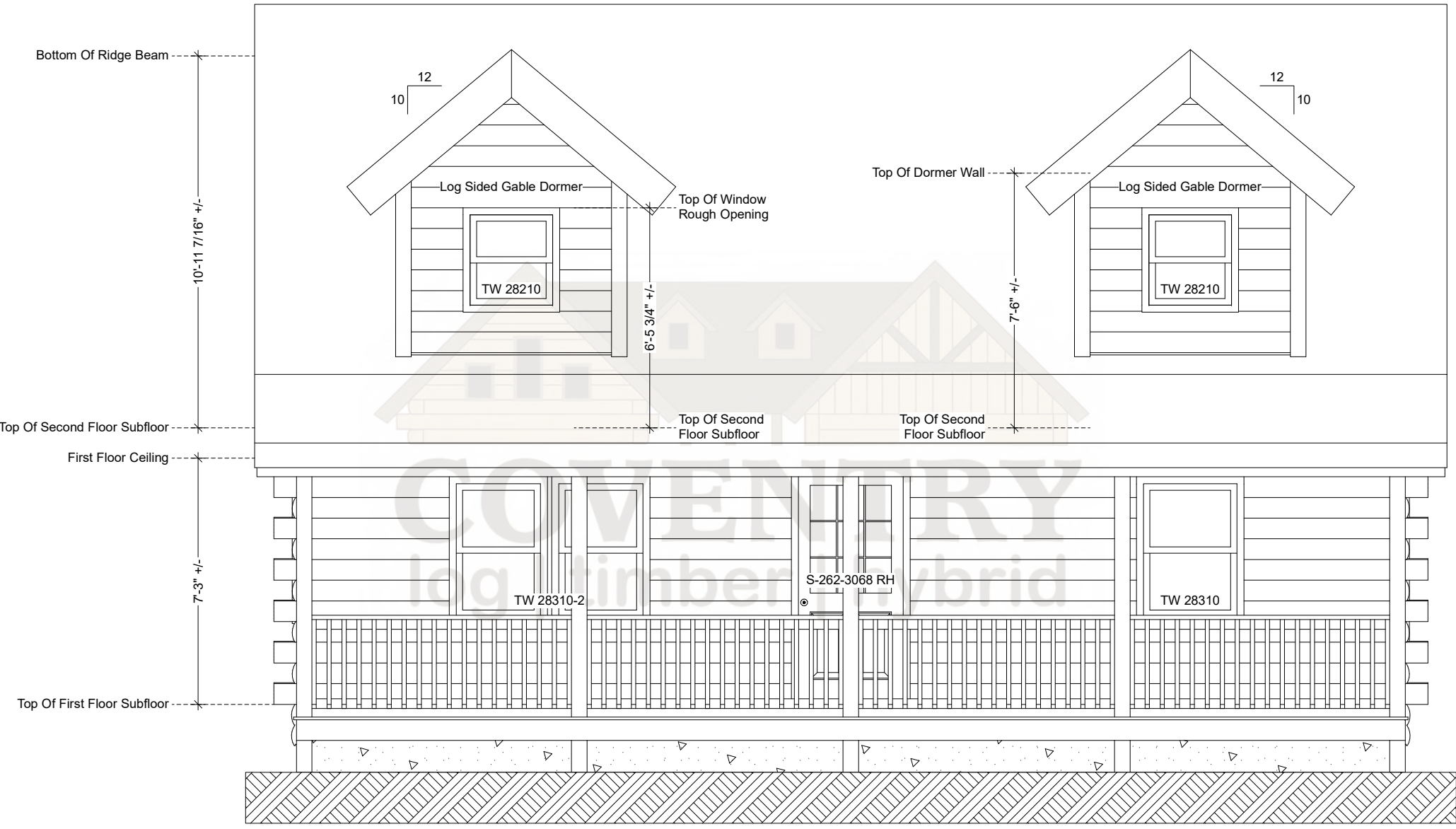
Fairfield Front Elevation
