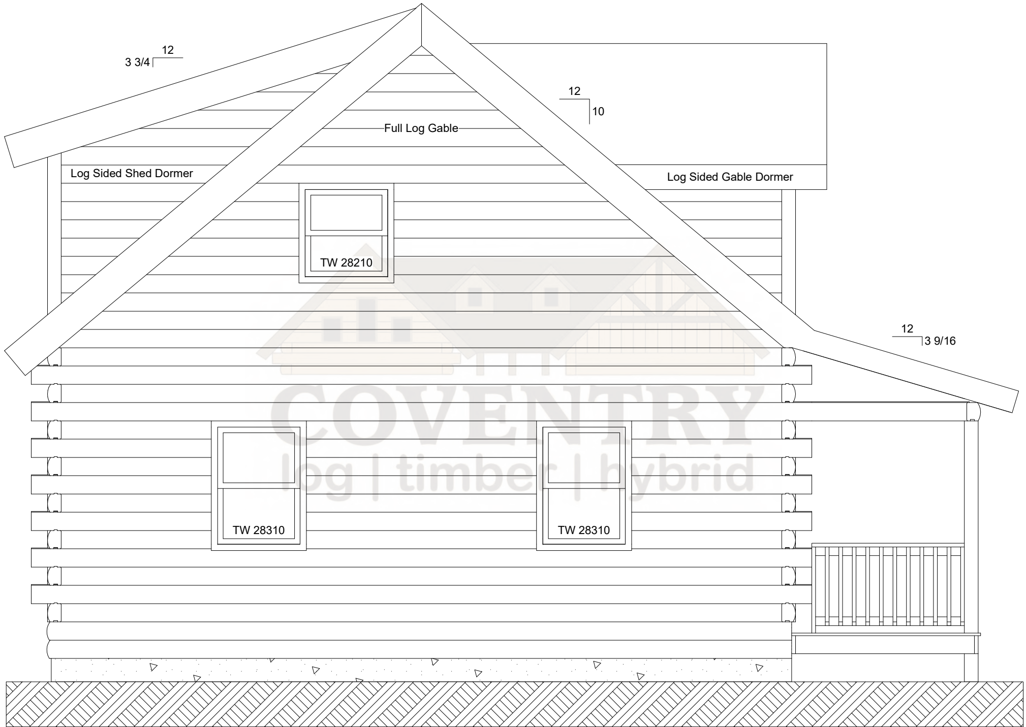
Fairfield Left Elevation
