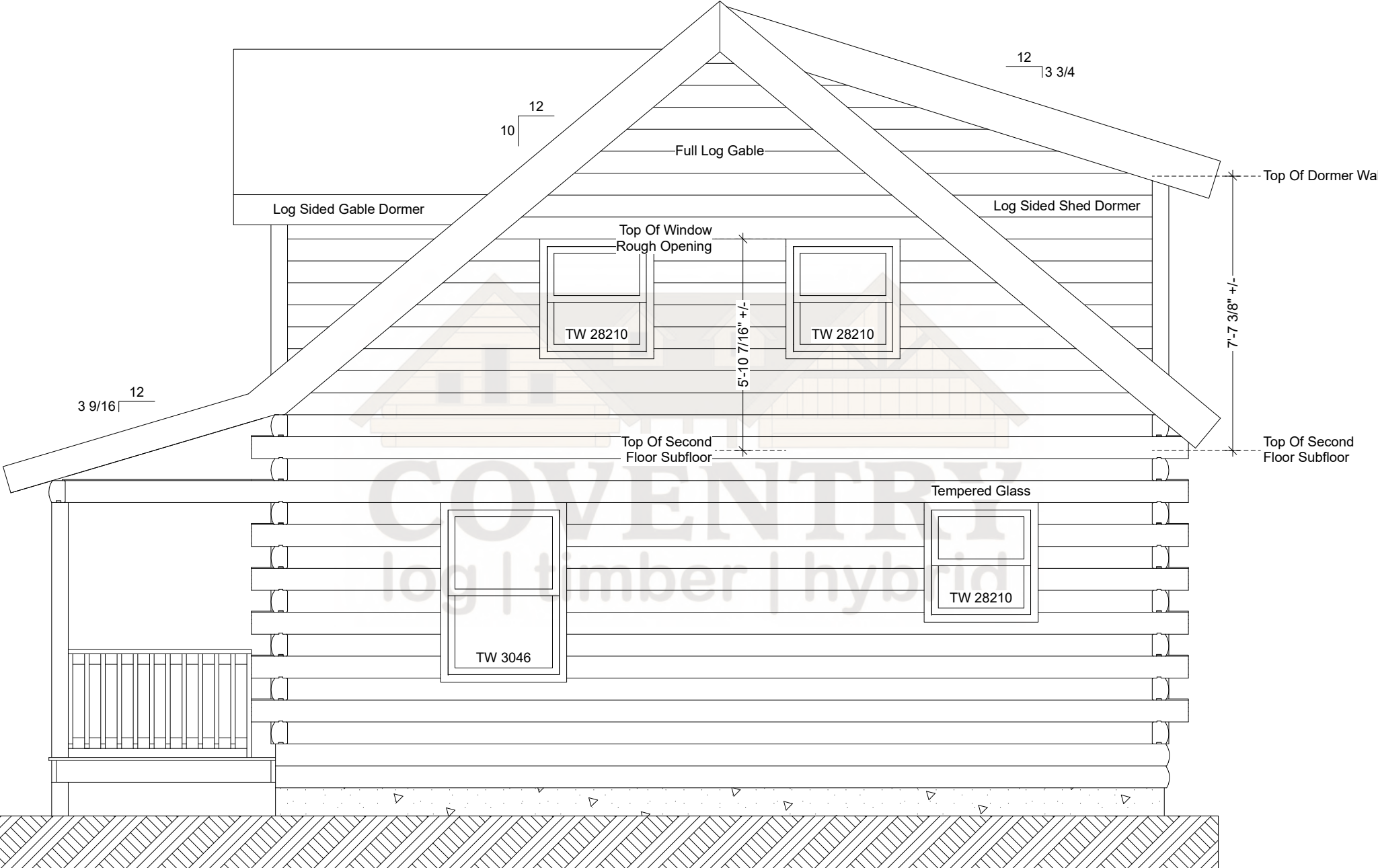
Fairfield Right Elevation
