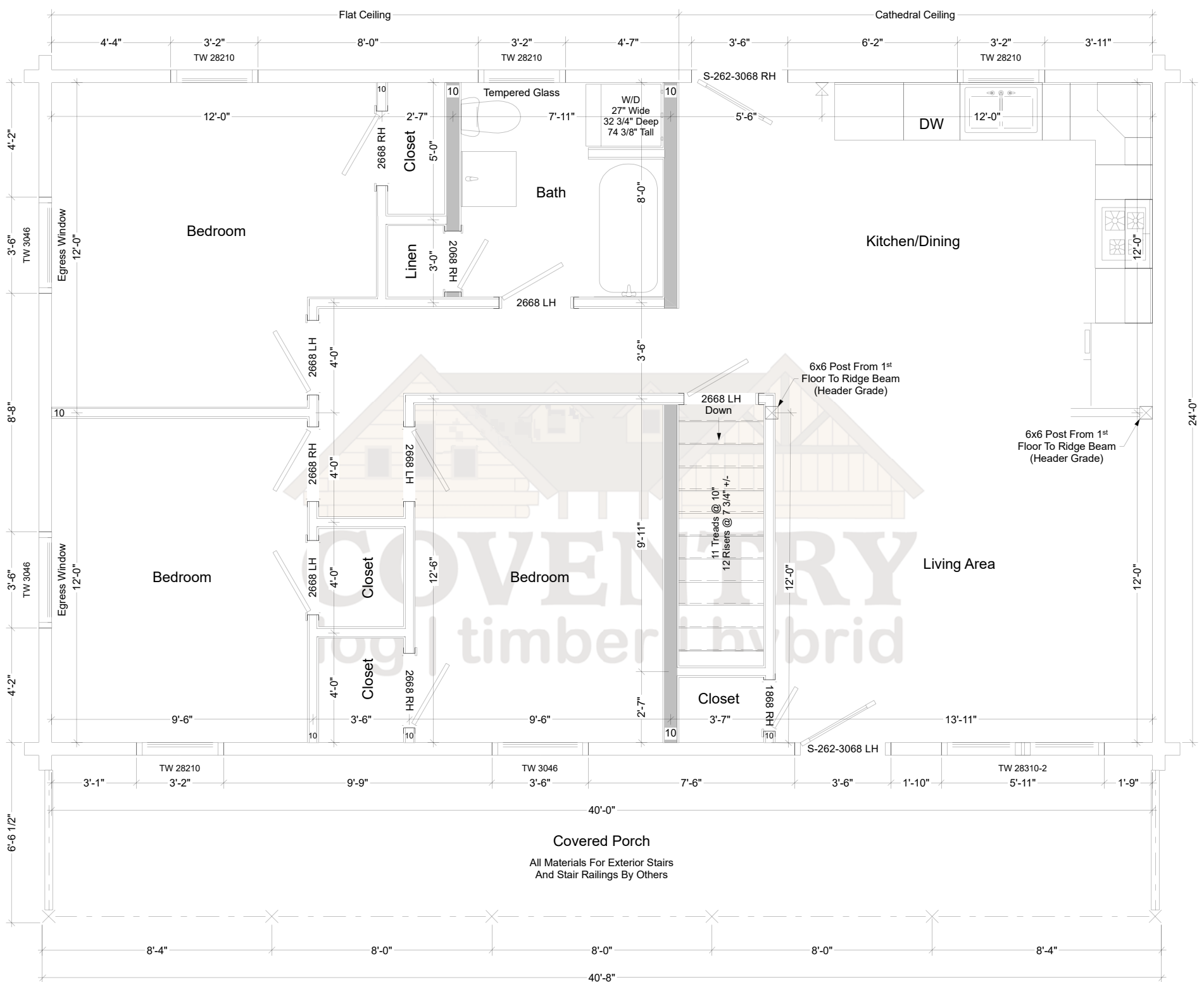
Franklin First Floor Plan
