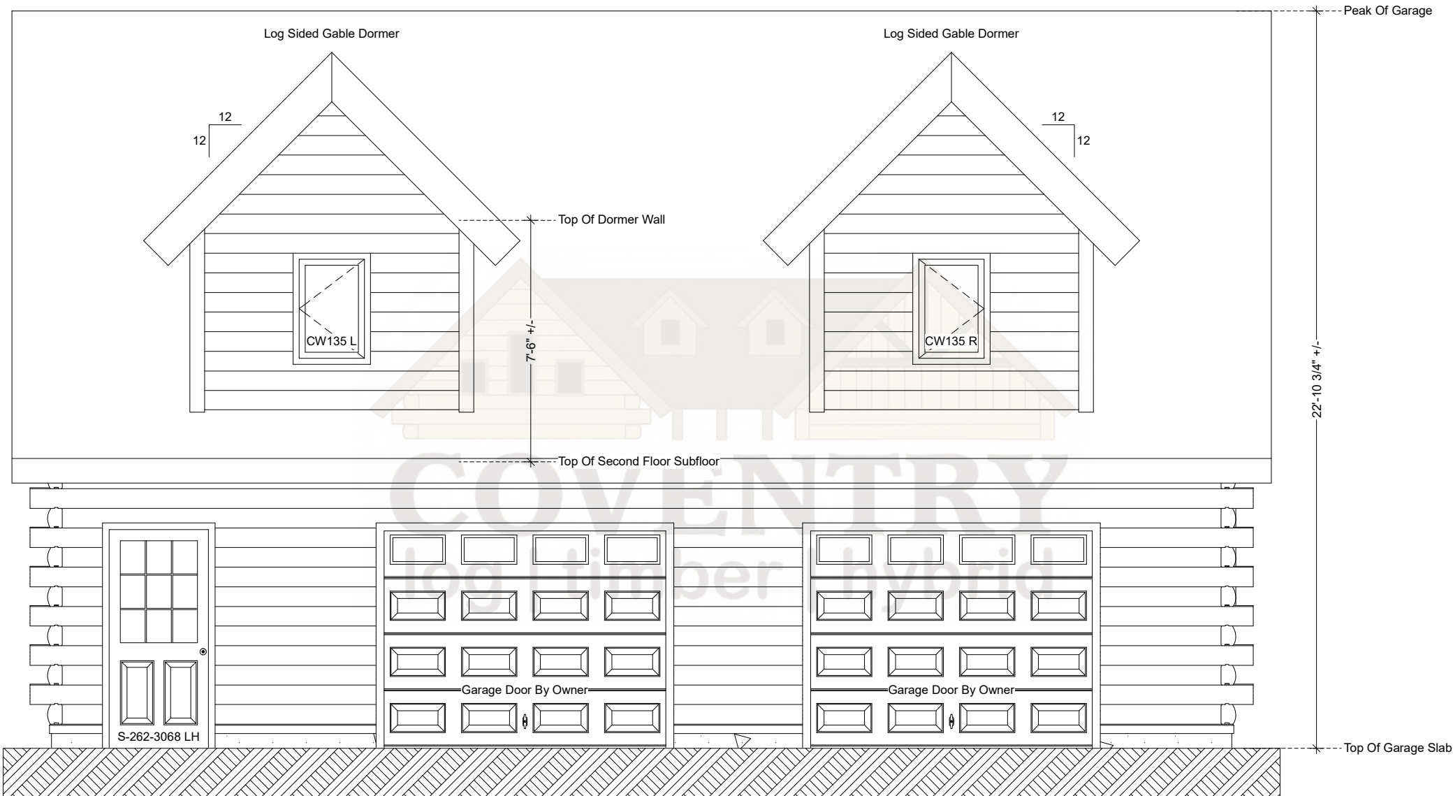
Garage Apartment Front Elevation
