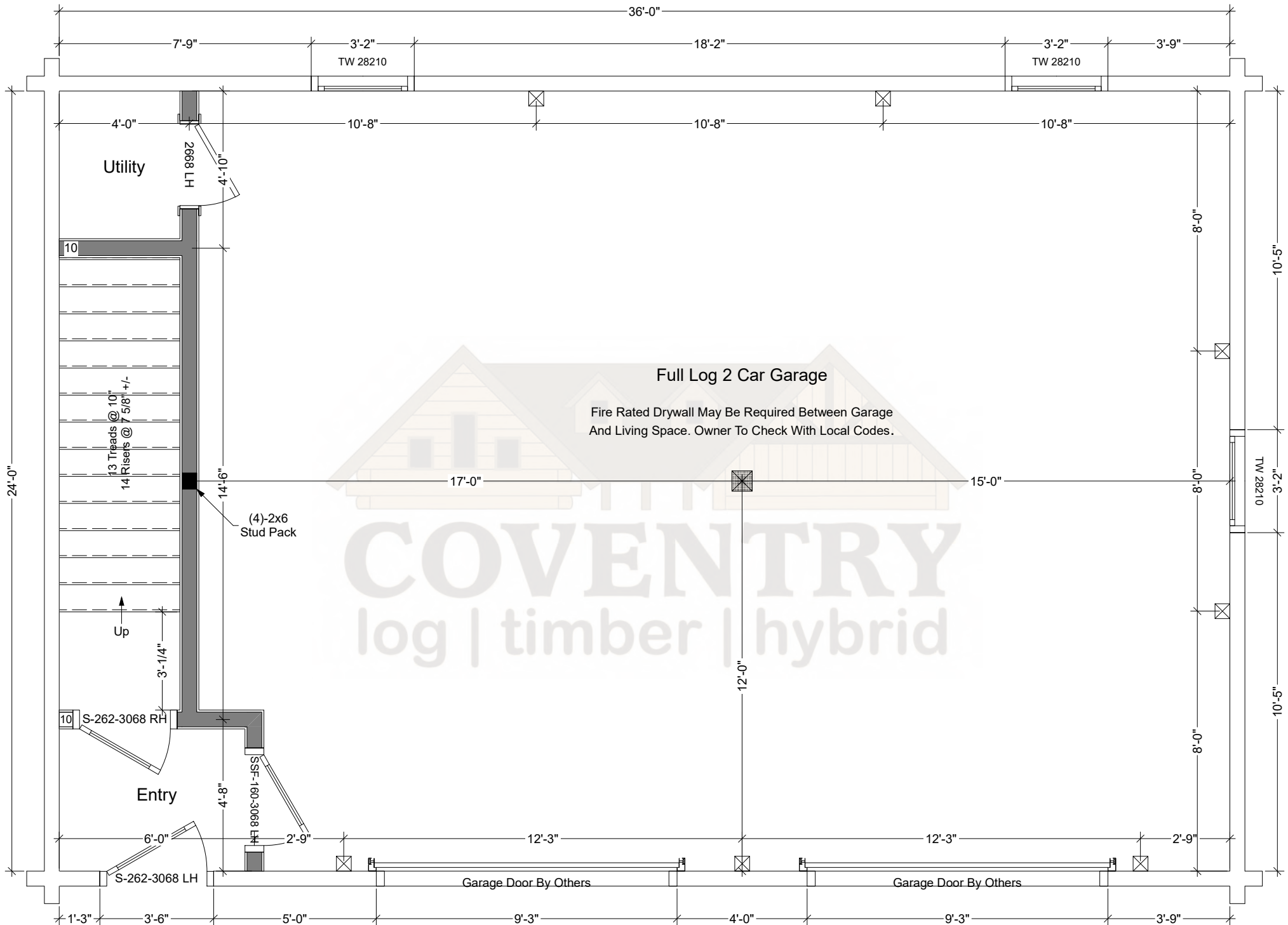
Garage Apartment First Floor Plan
