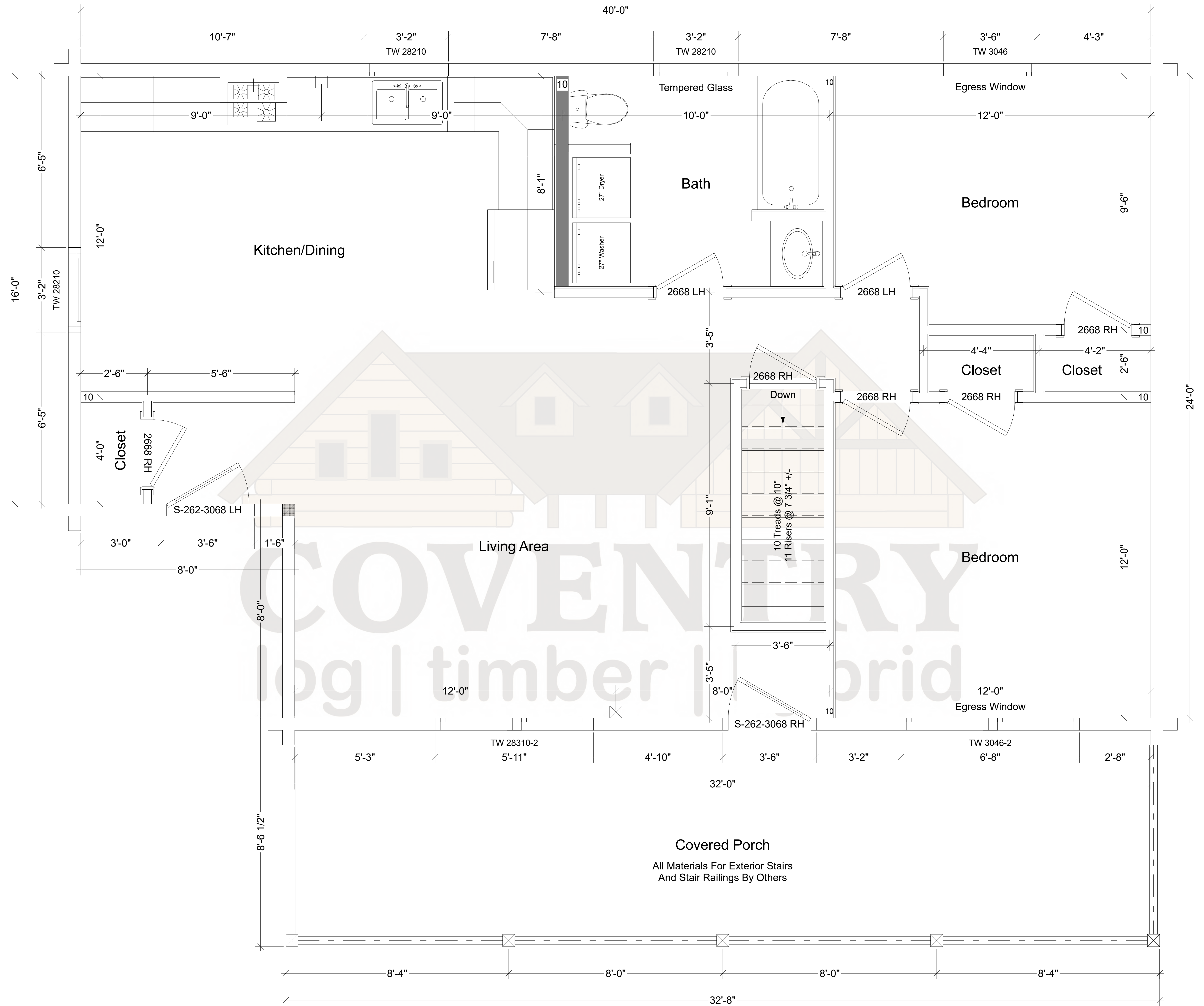
Glenwood Floor Plan
