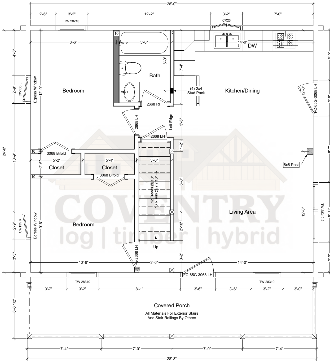
Hickory First Floor Plan
