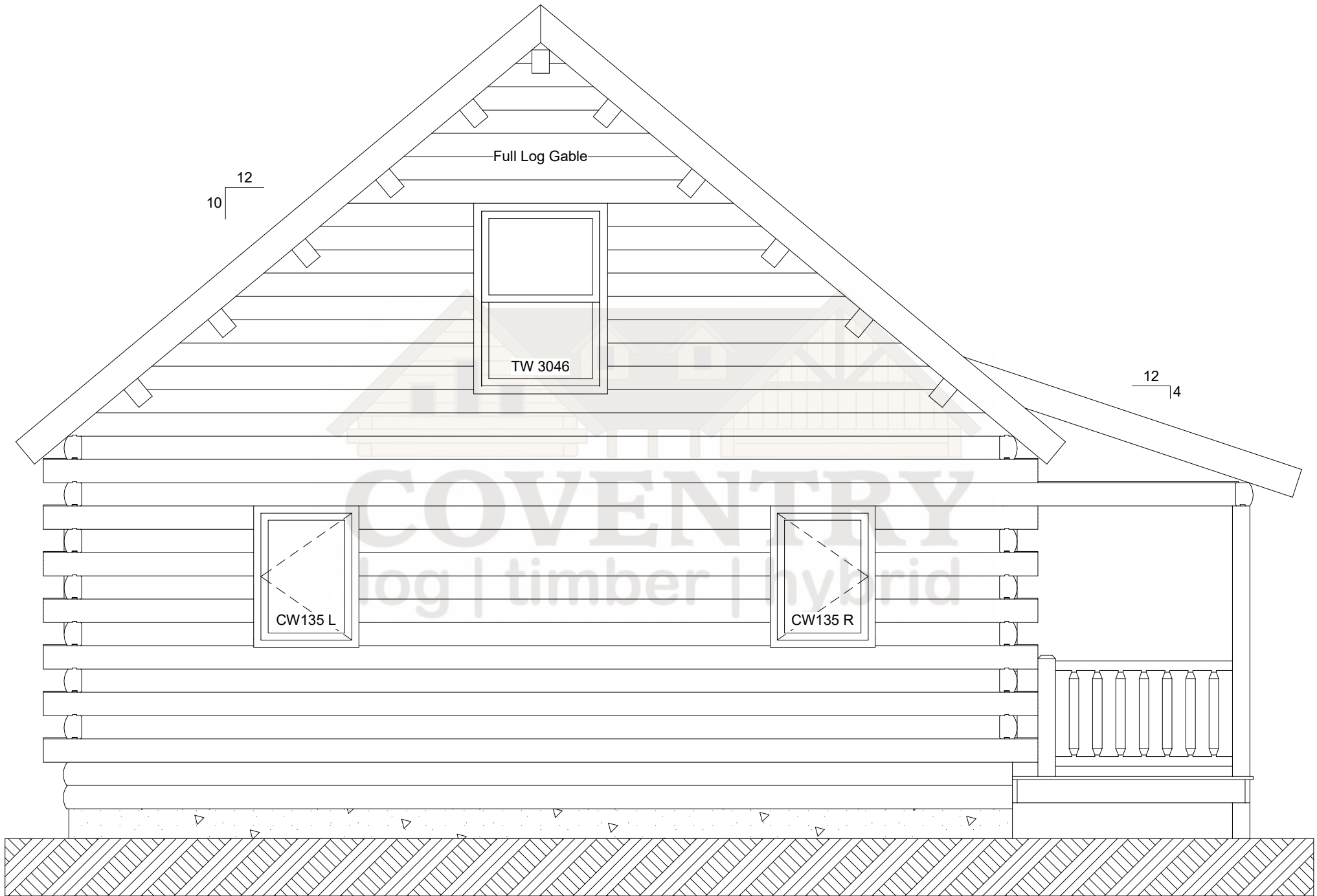
Hickory Left Elevation
