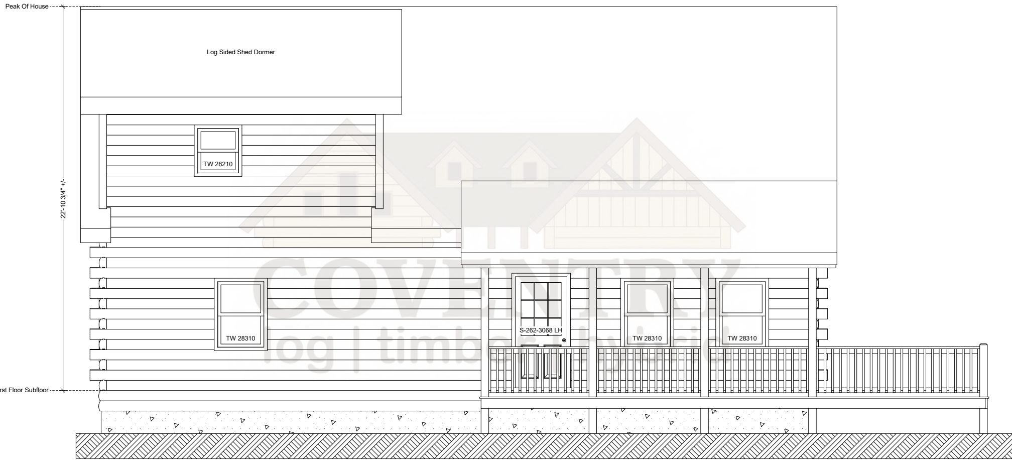
Hillside Left Elevation
