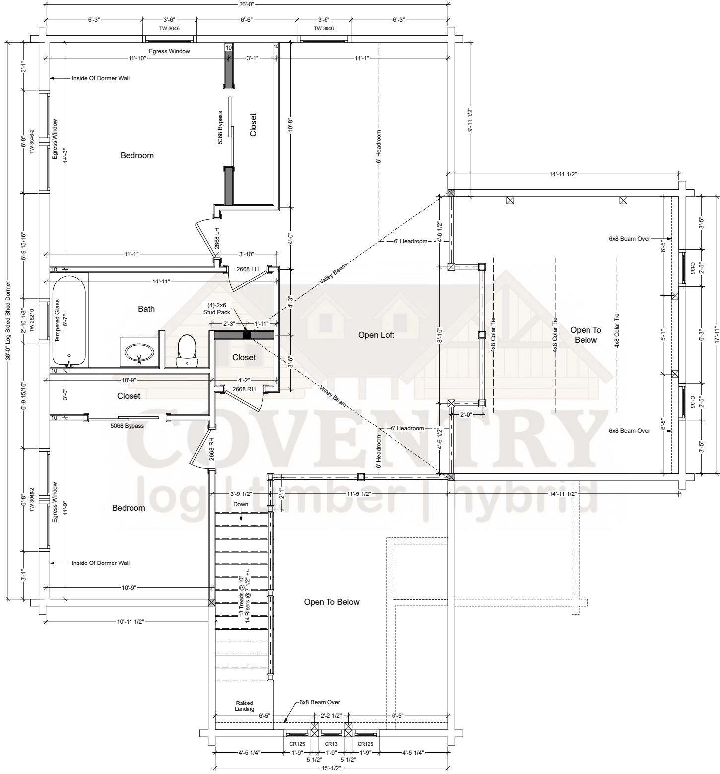
Ironwood Second Floor Plan
