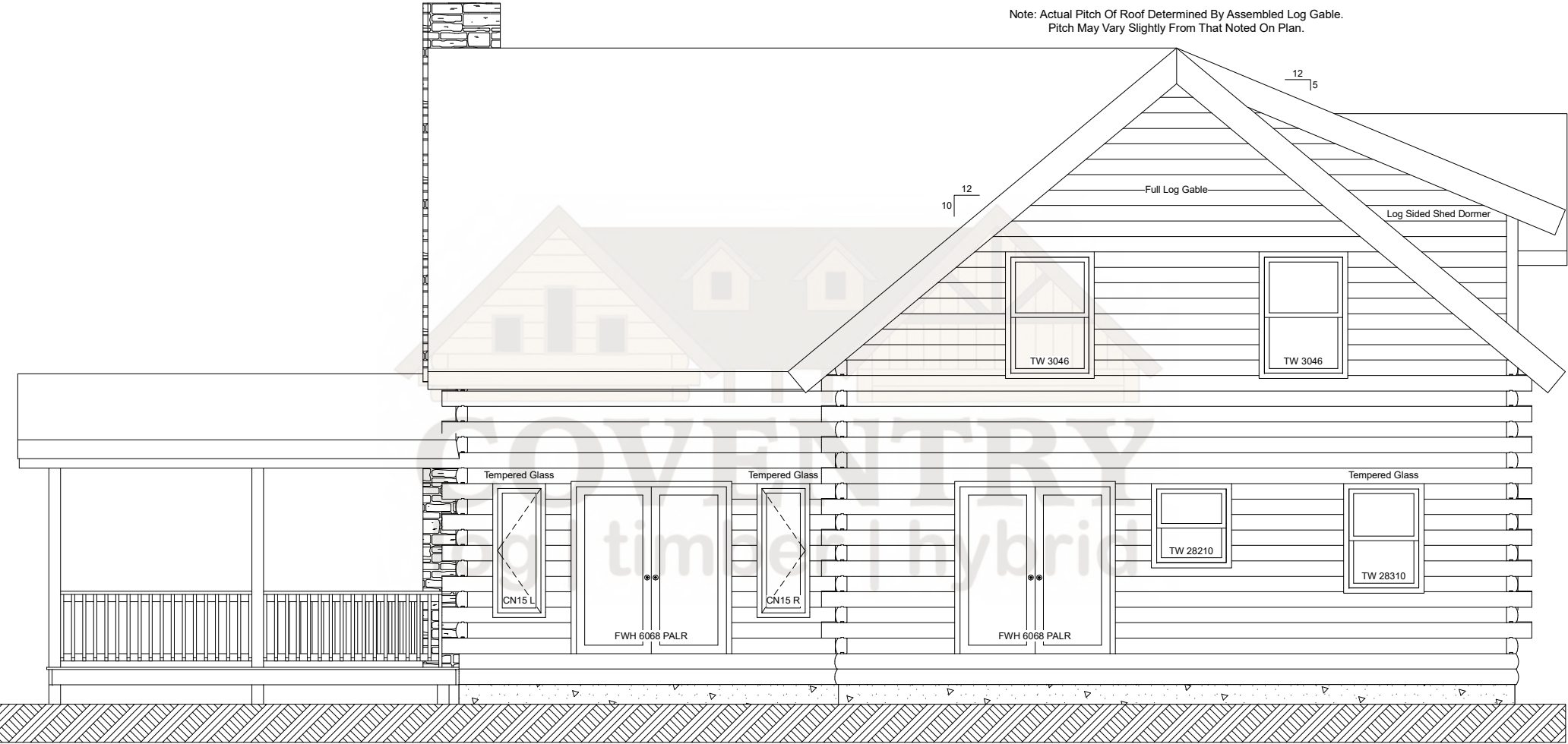
Ironwood Rear Elevation
