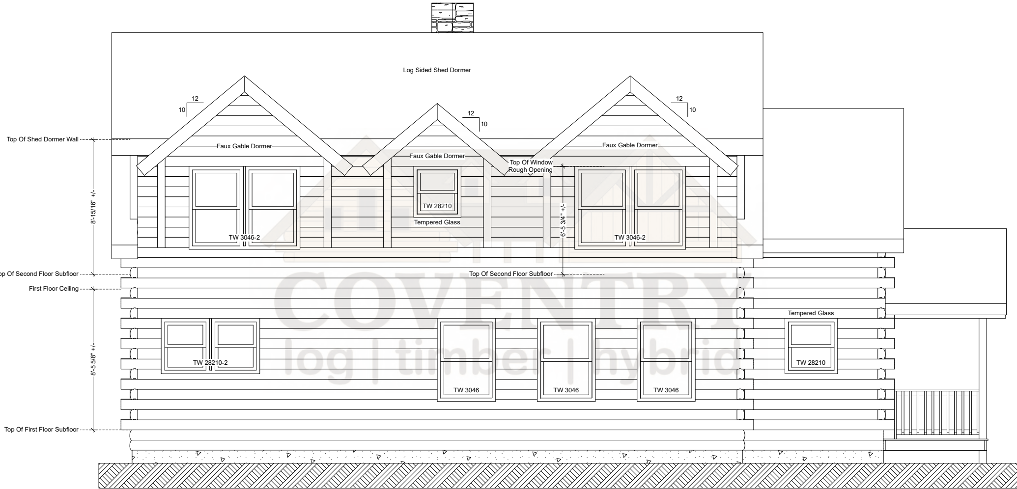
Ironwood Left Elevation
