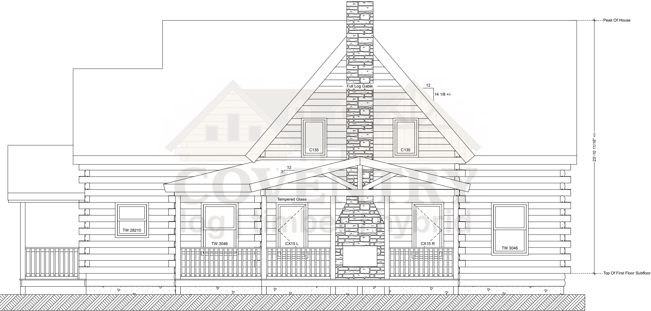
Ironwood Right Elevation
