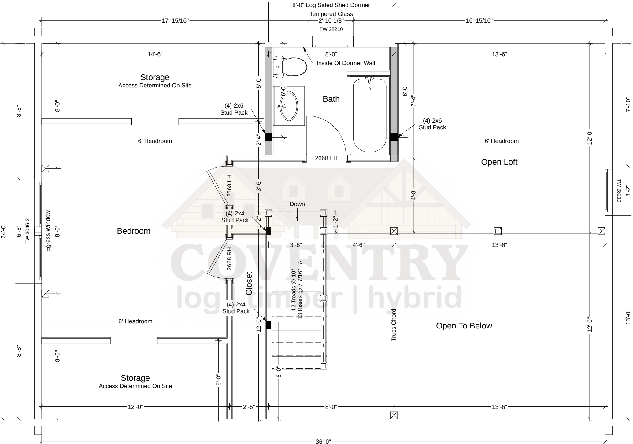
Killington Second Floor Plan
