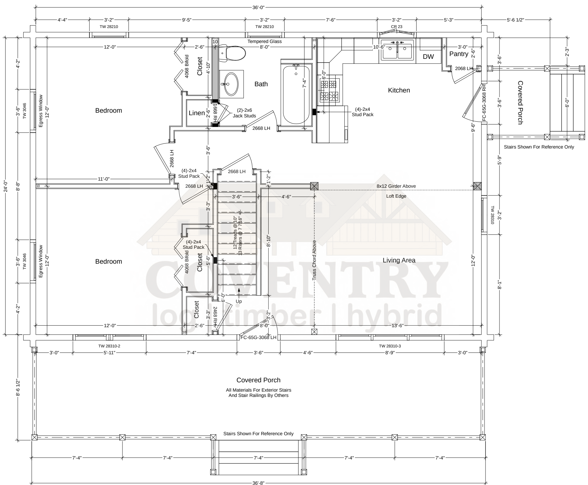
Killington First Floor Plan
