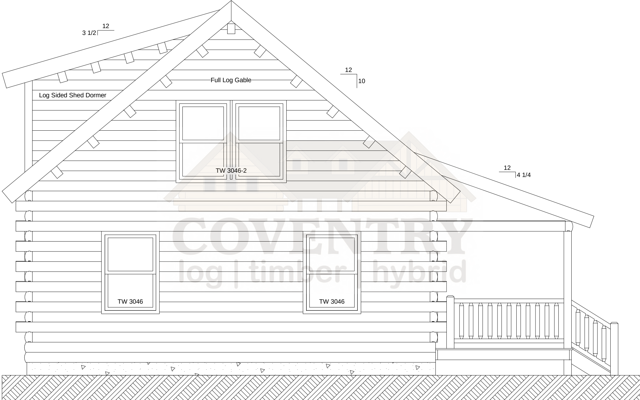
Killington Left Elevation
