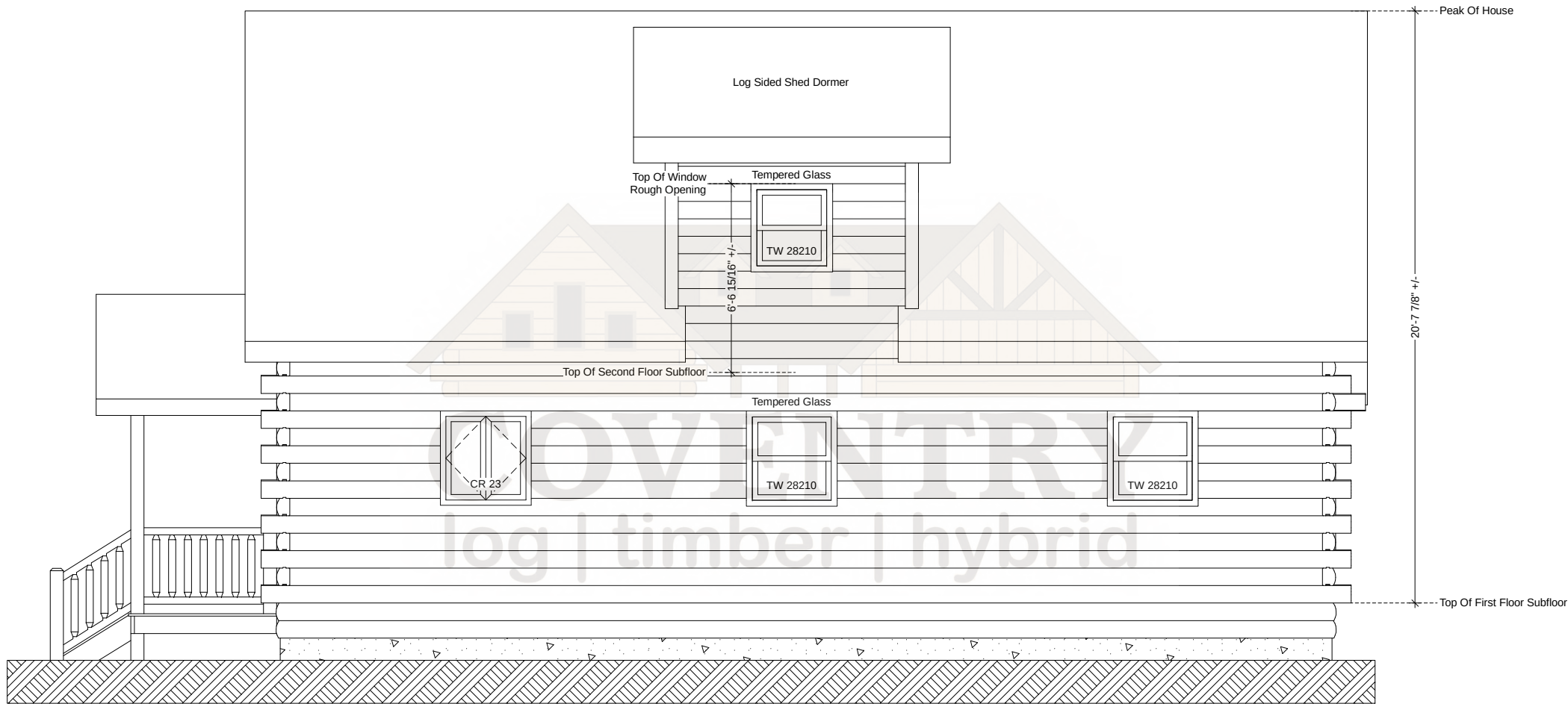
Killington Rear Elevation
