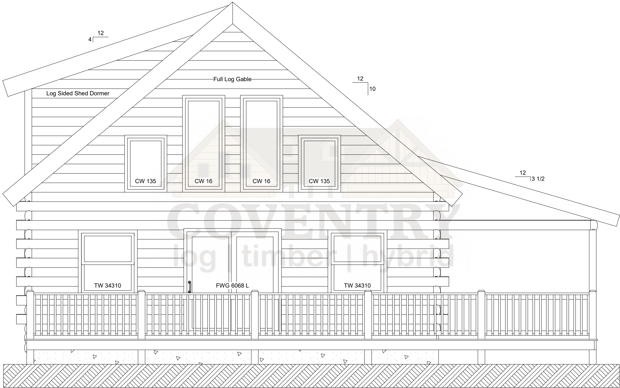
Kinsman Left Elevation
