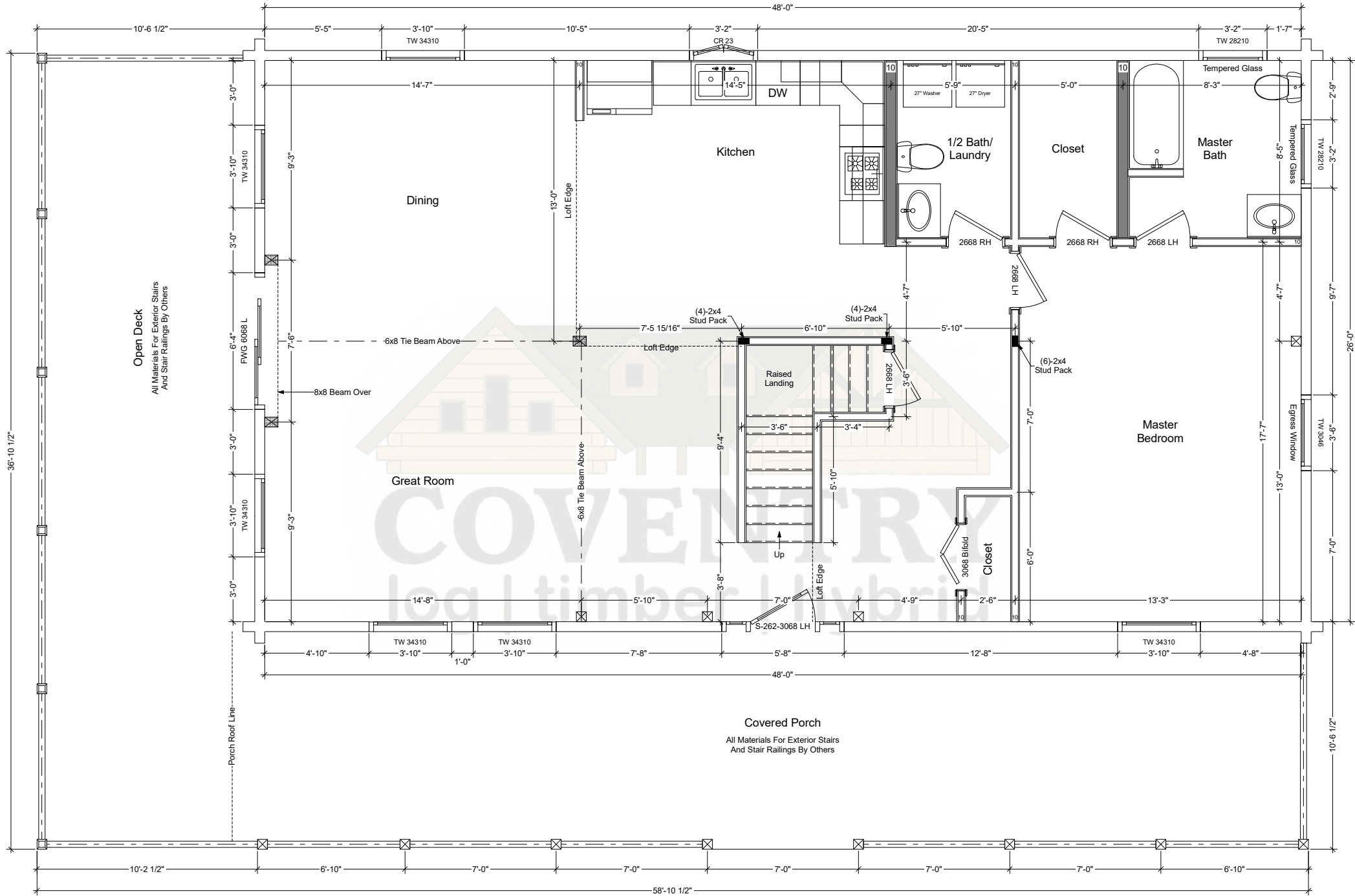
Kinsman First Floor Plan
