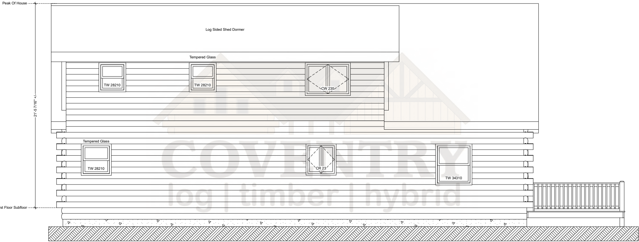
Kinsman Rear Elevation
