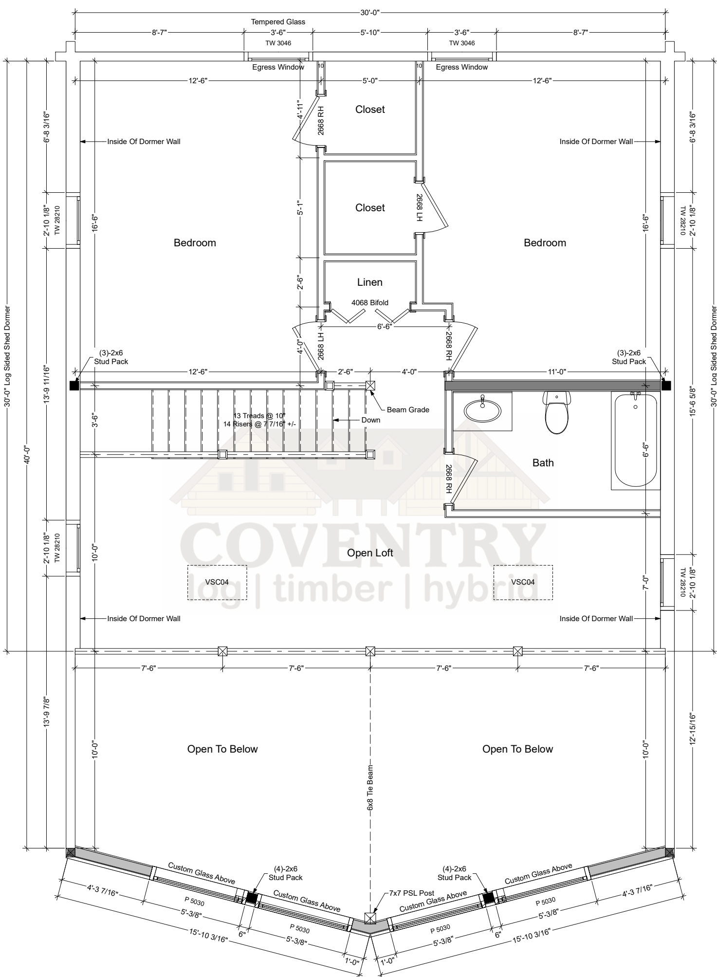
Lancaster Second Floor Plan
