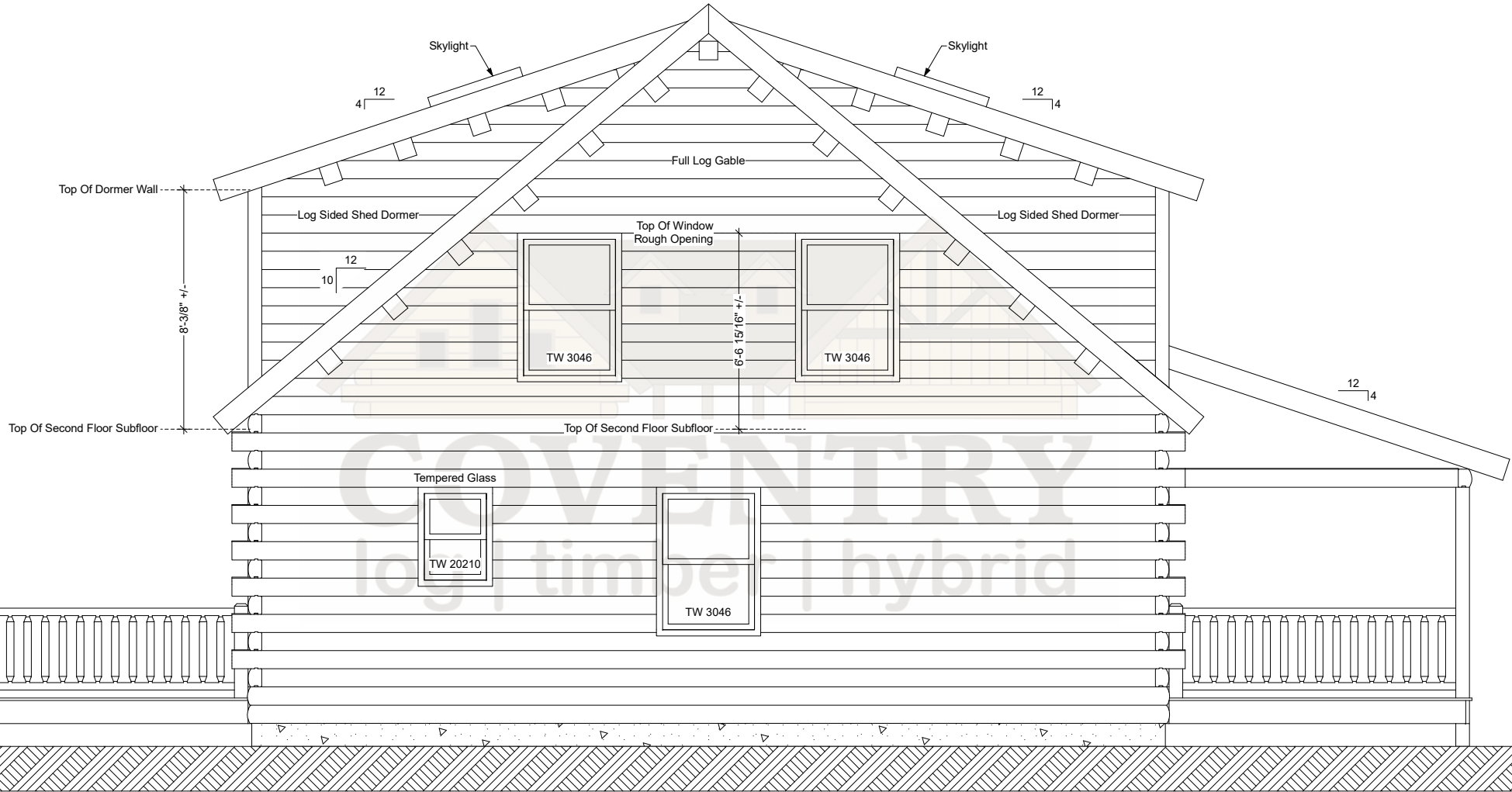
Lancaster Rear Elevation
