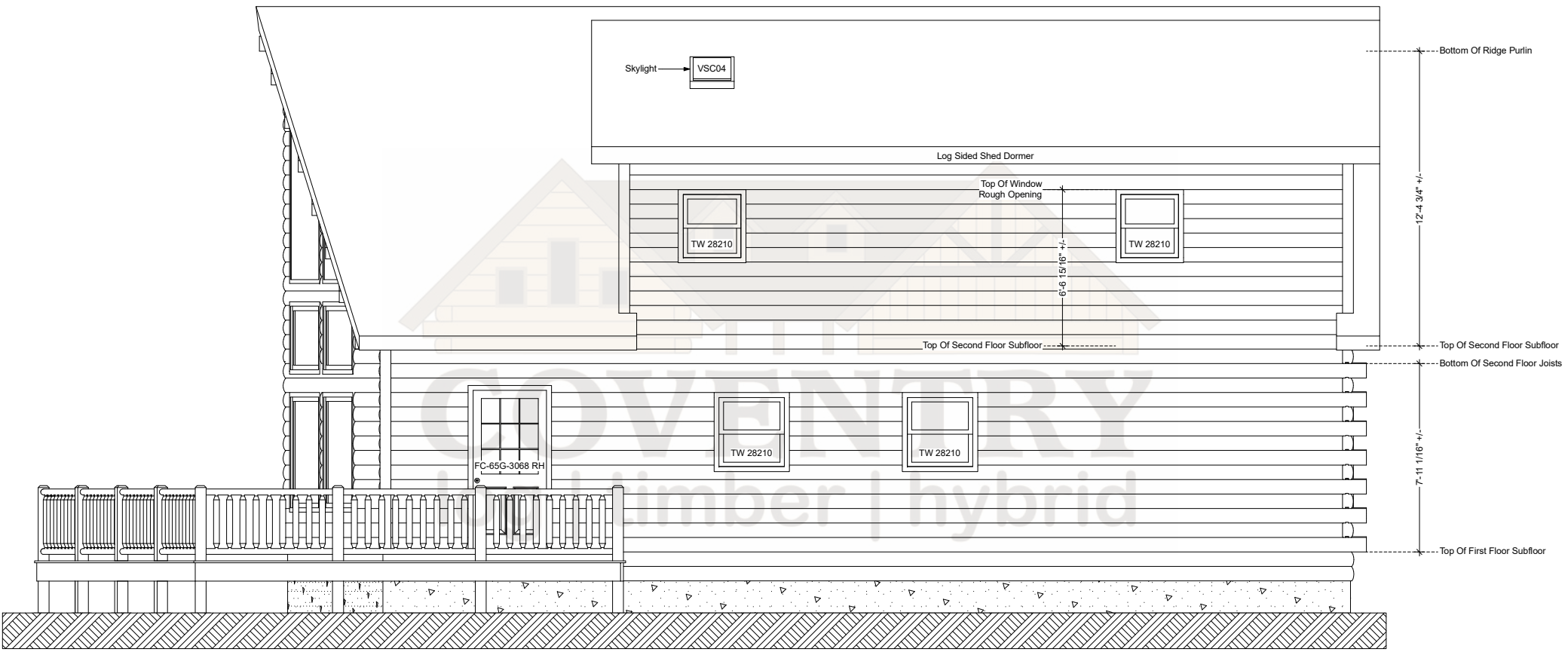
Lancaster Right Elevation
