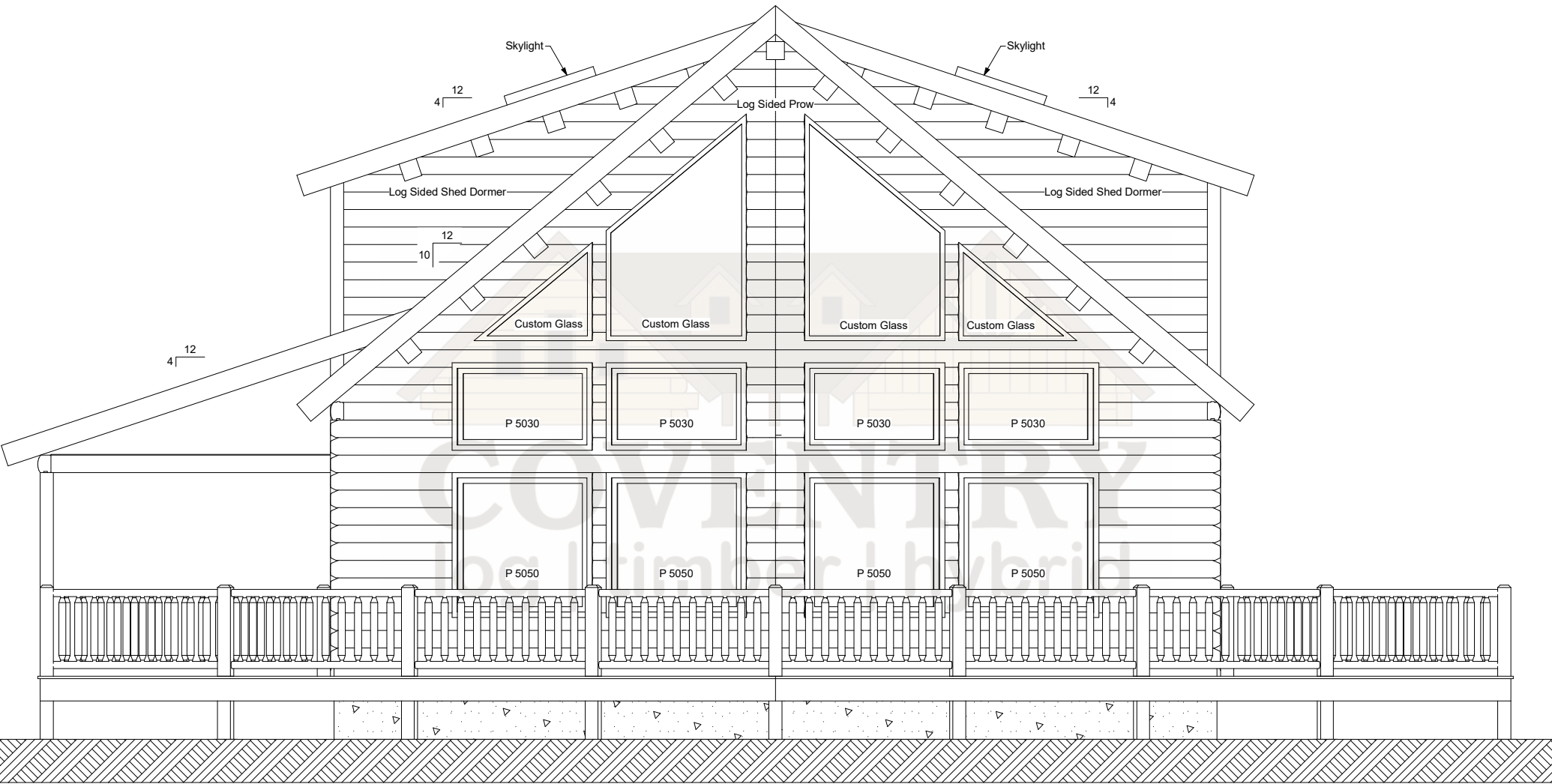
Lancaster Front Elevation
