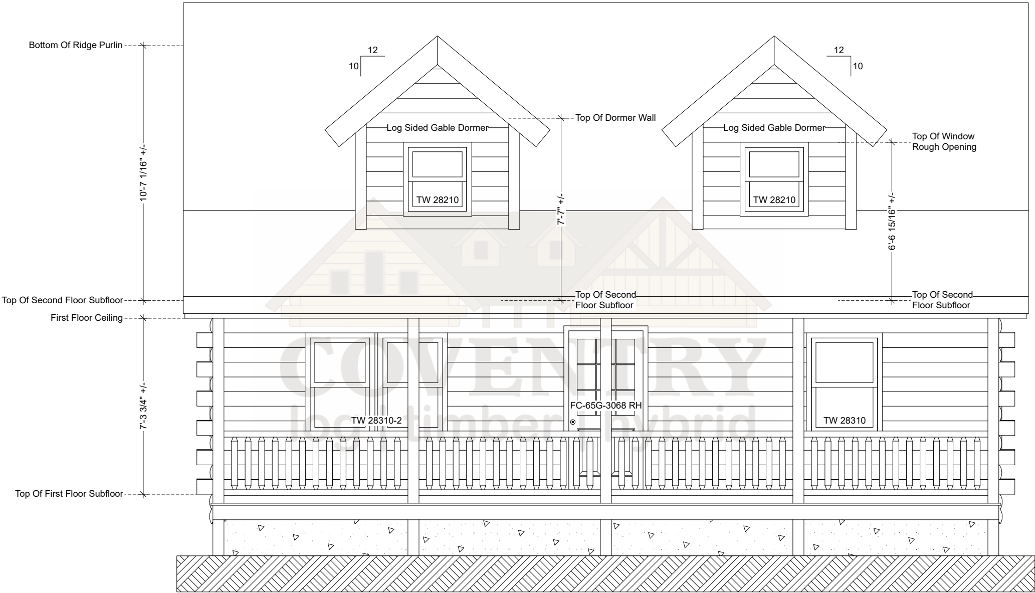
Mansfield Front Elevation
