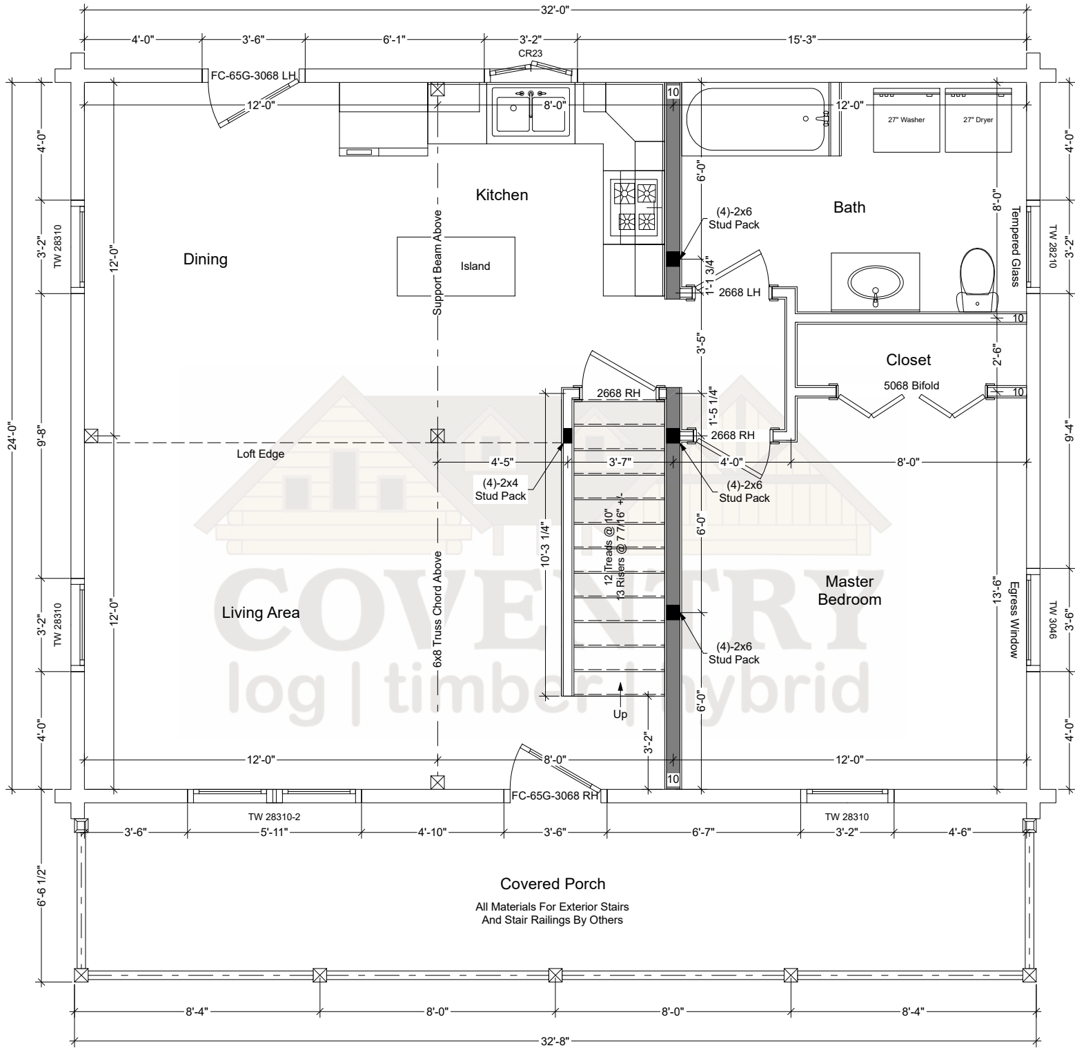
Mansfield First Floor Plan
