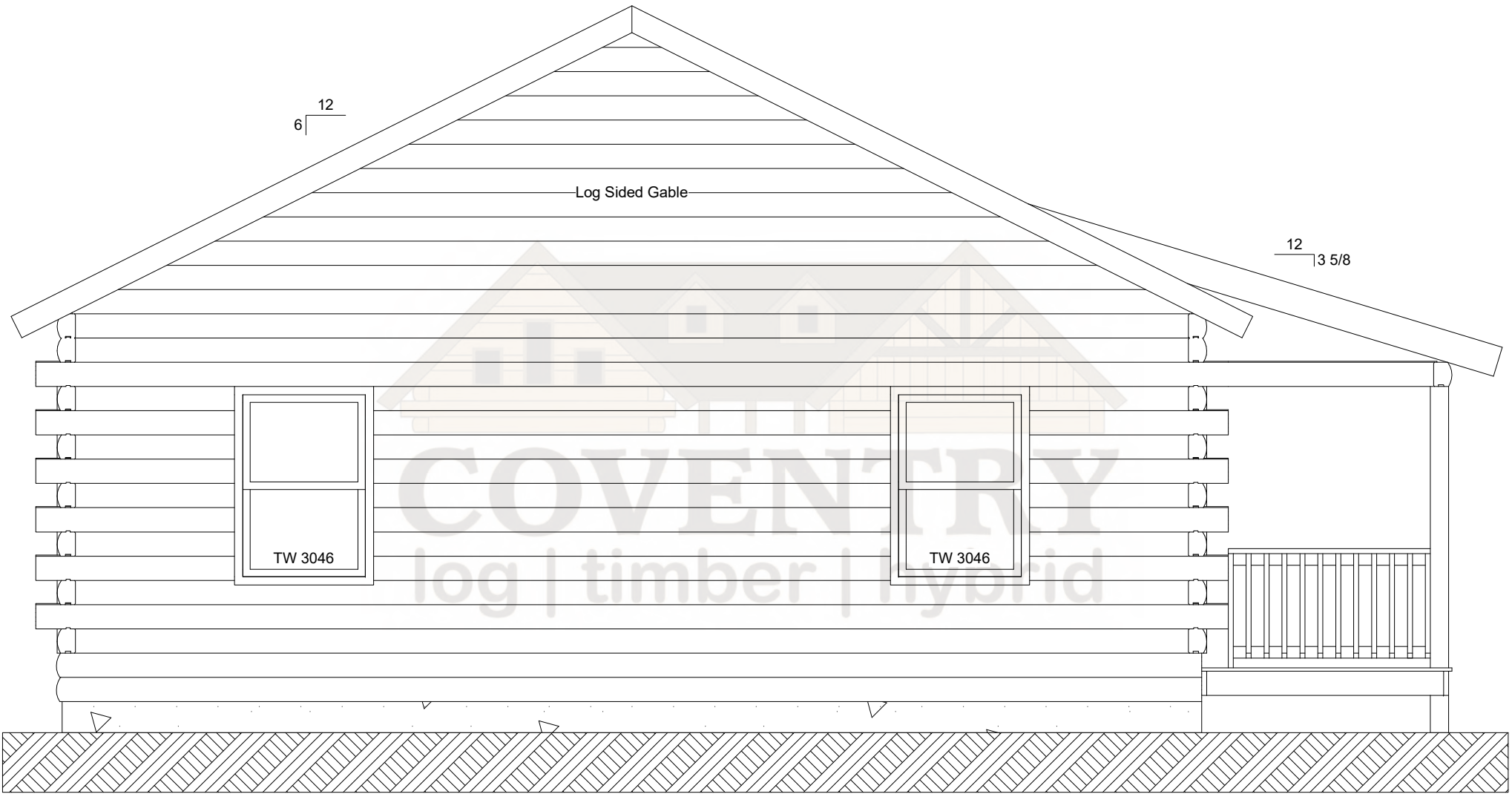
Meadows Left Elevation
