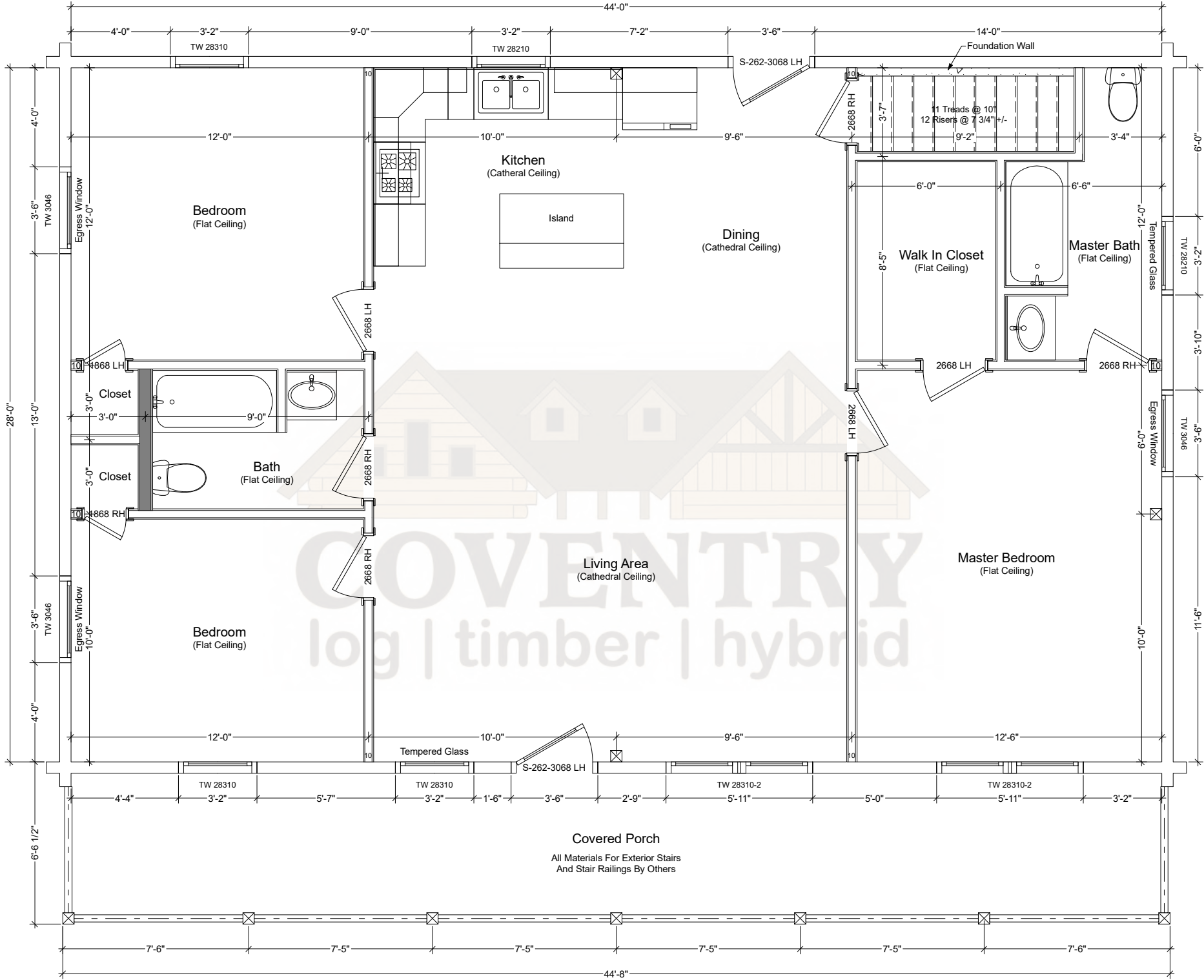
Meadows First Floor Plan
