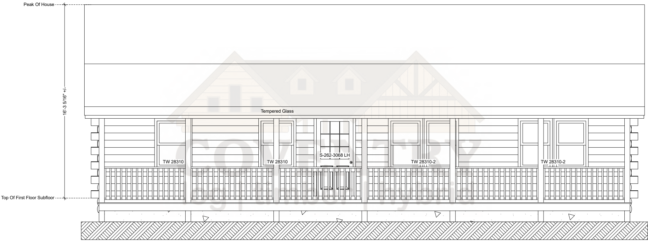
Meadows Front Elevation
