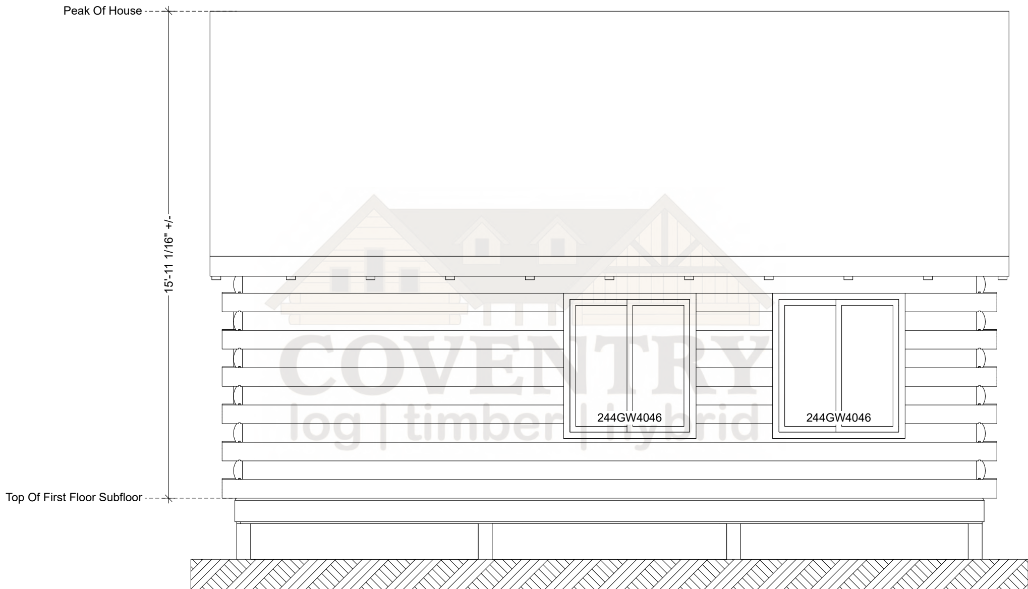
Mountaineer Rear Elevation
