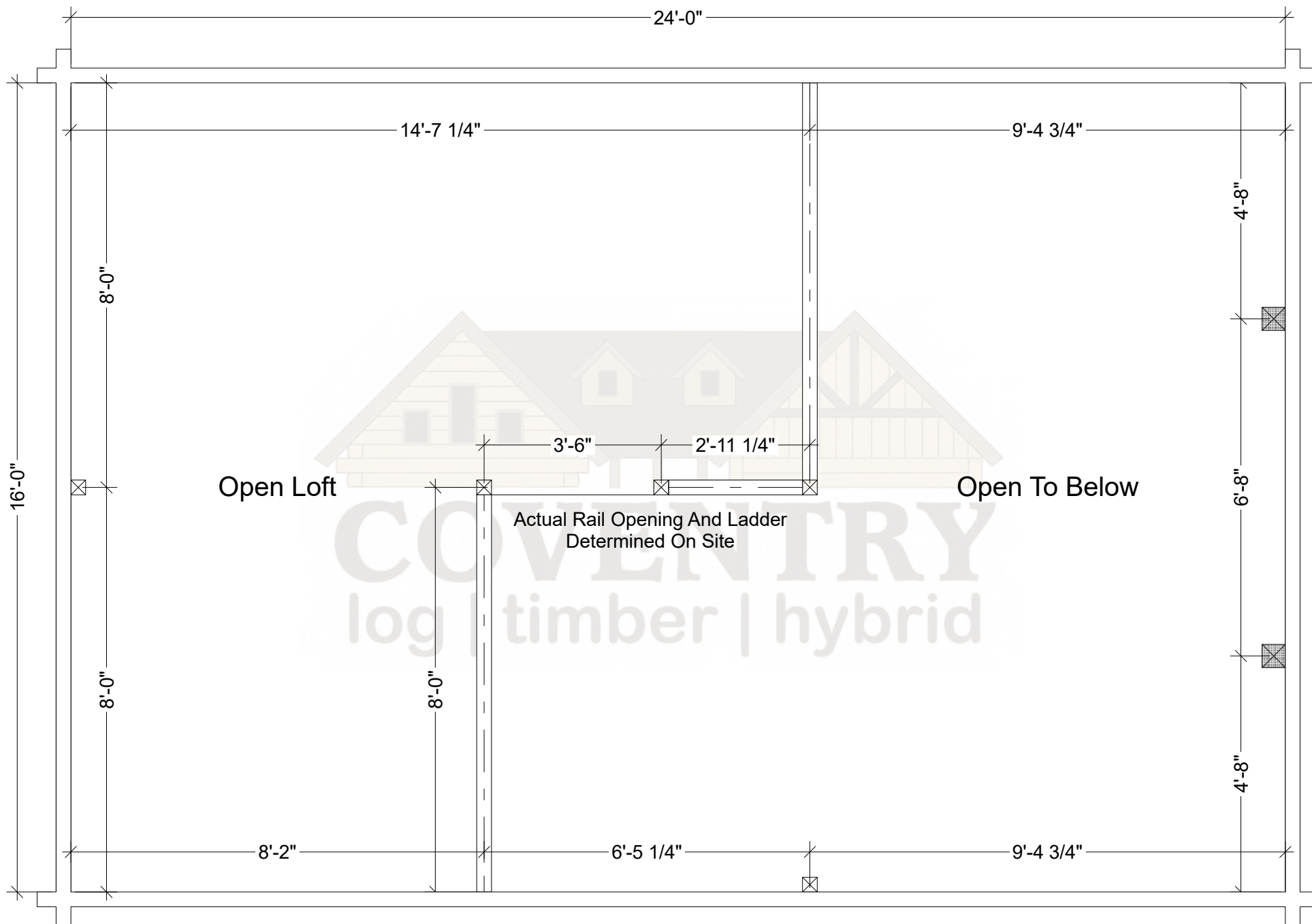
Mountaineer Second Floor Plan
