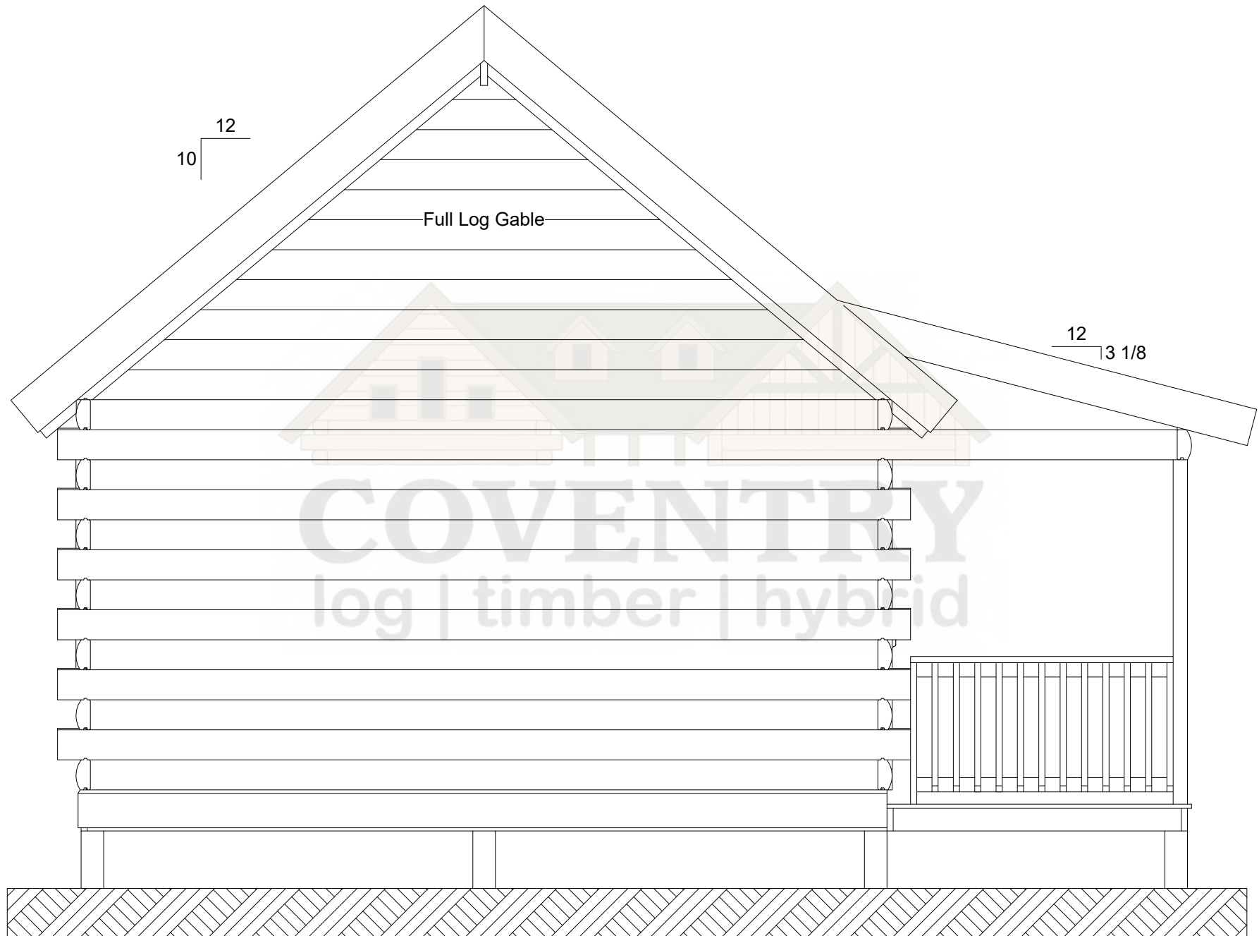
Mountaineer Left Elevation
