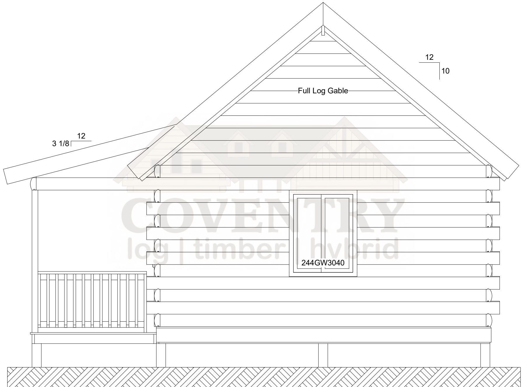
Mountaineer Right Elevation
