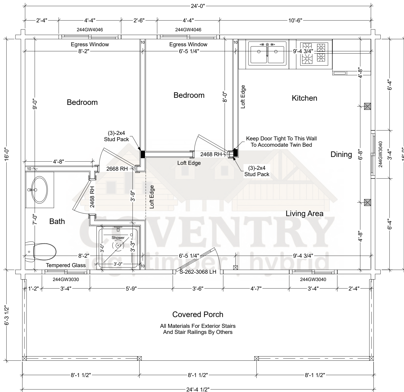
Mountaineer First Floor Plan
