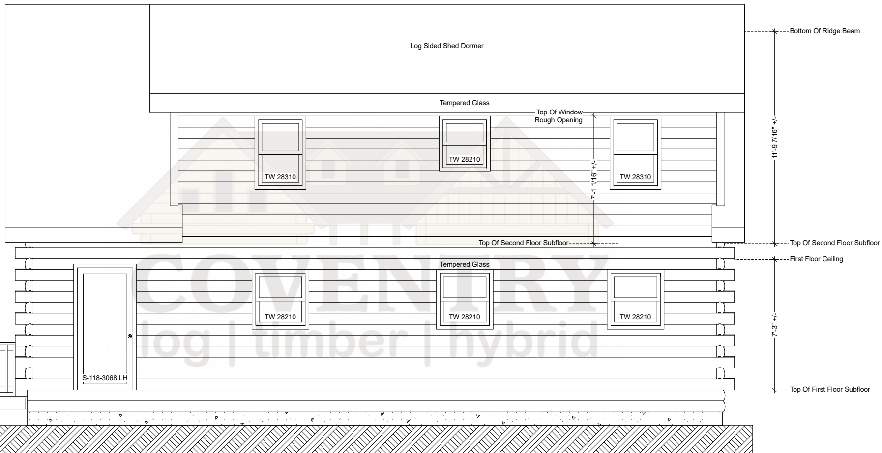
Oak Ridge Right Elevation
