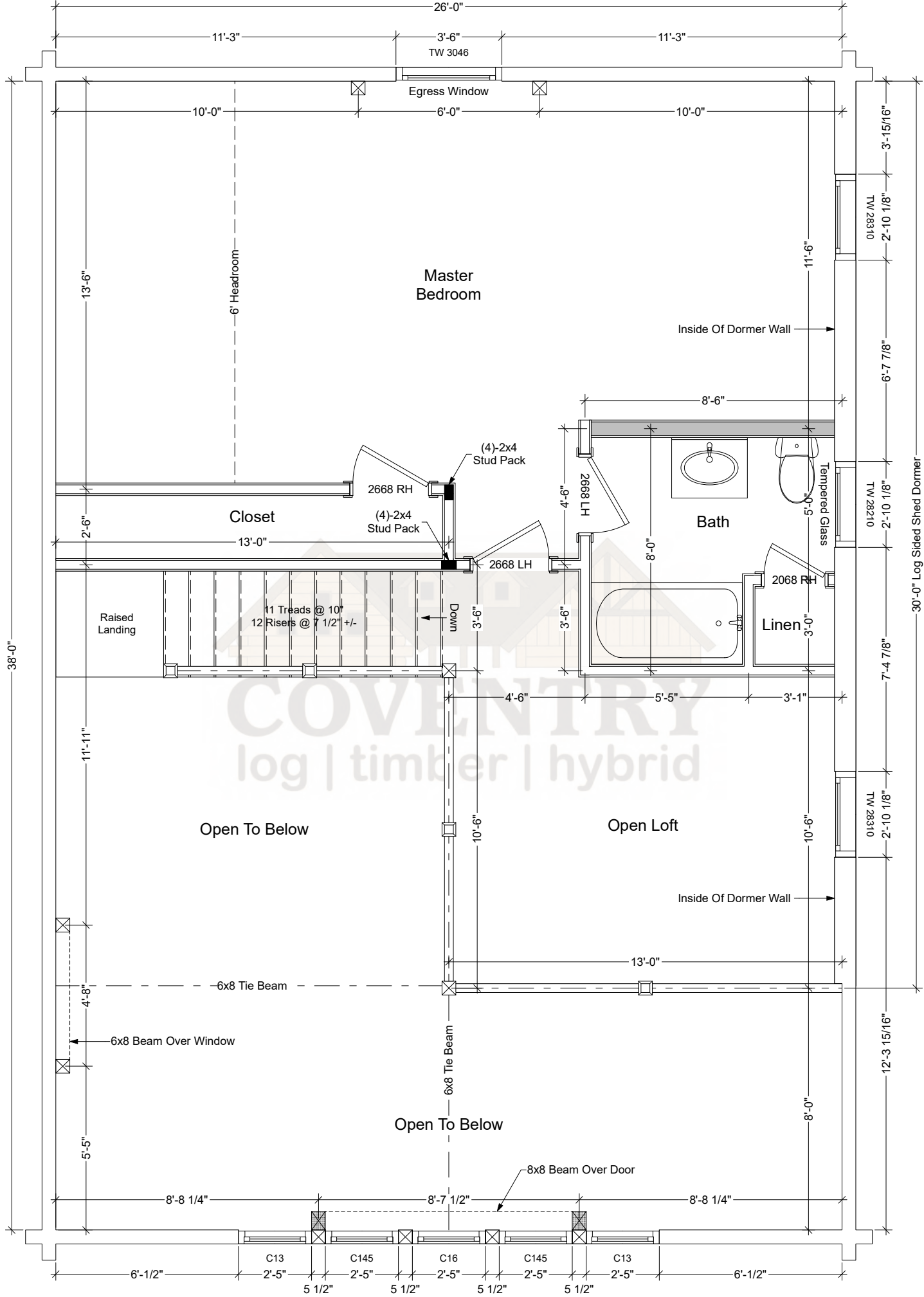
Oak Ridge Second Floor Plan
