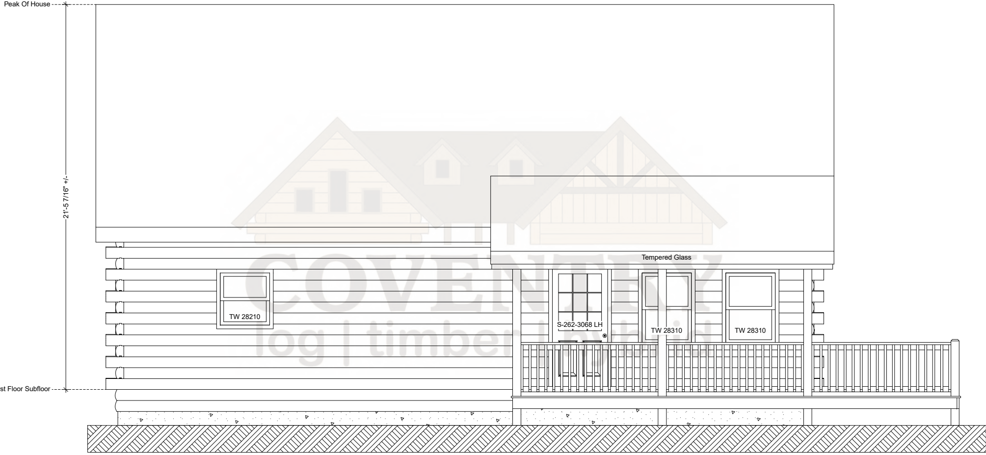
Oak Ridge Left Elevation
