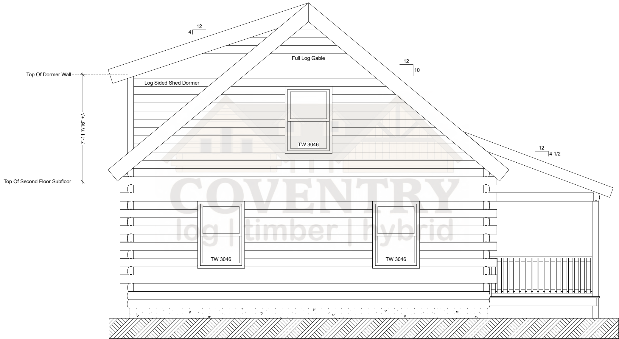
Oak Ridge Rear Elevation
