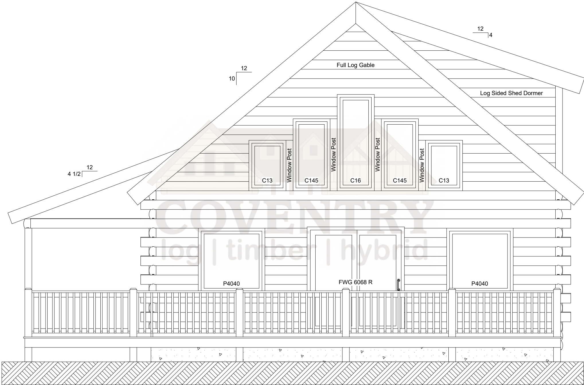
Oak Ridge Front Elevation
