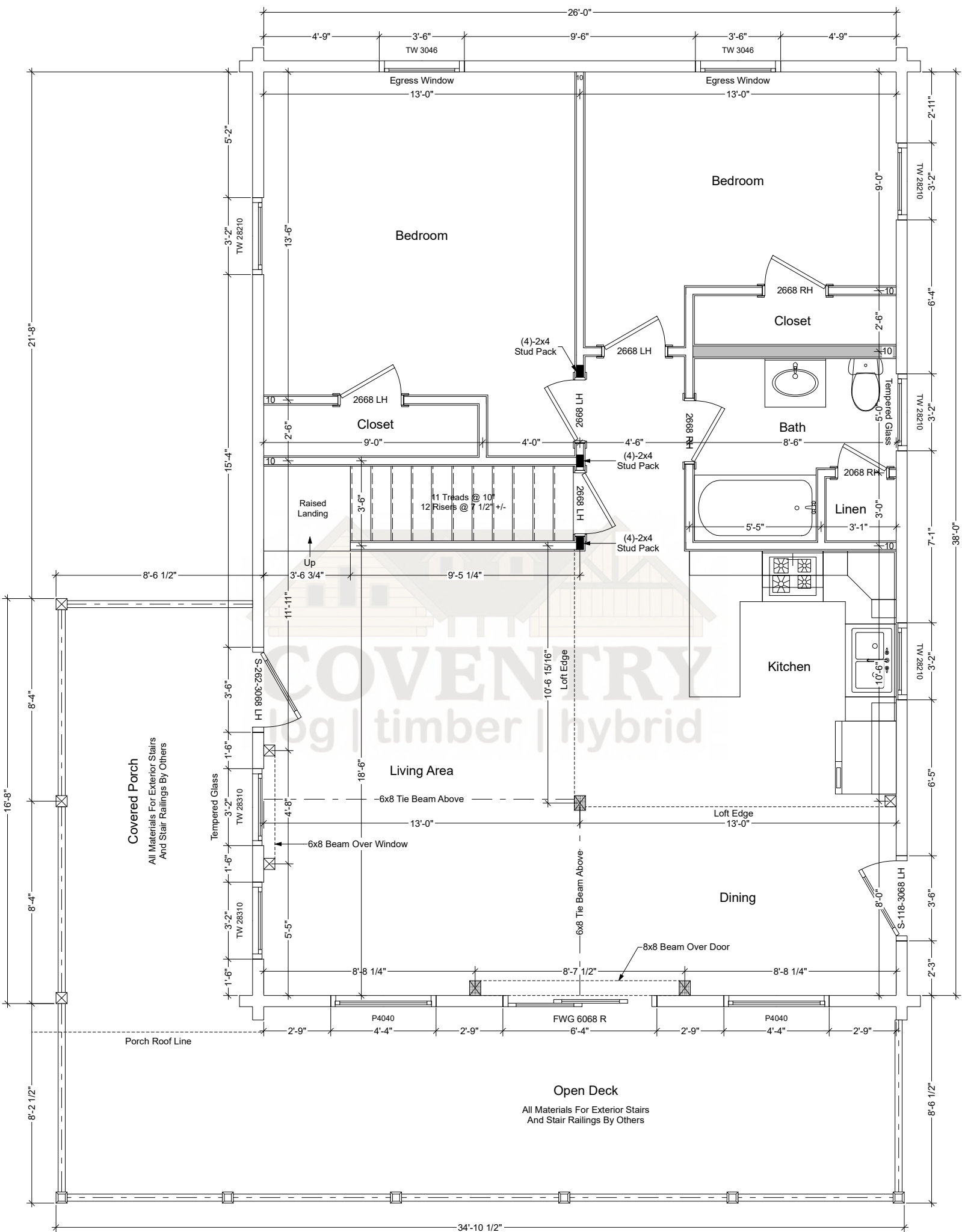
Oak Ridge First Floor Plan
