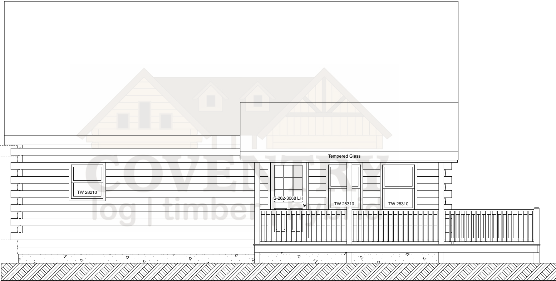
Riverside Left Elevation
