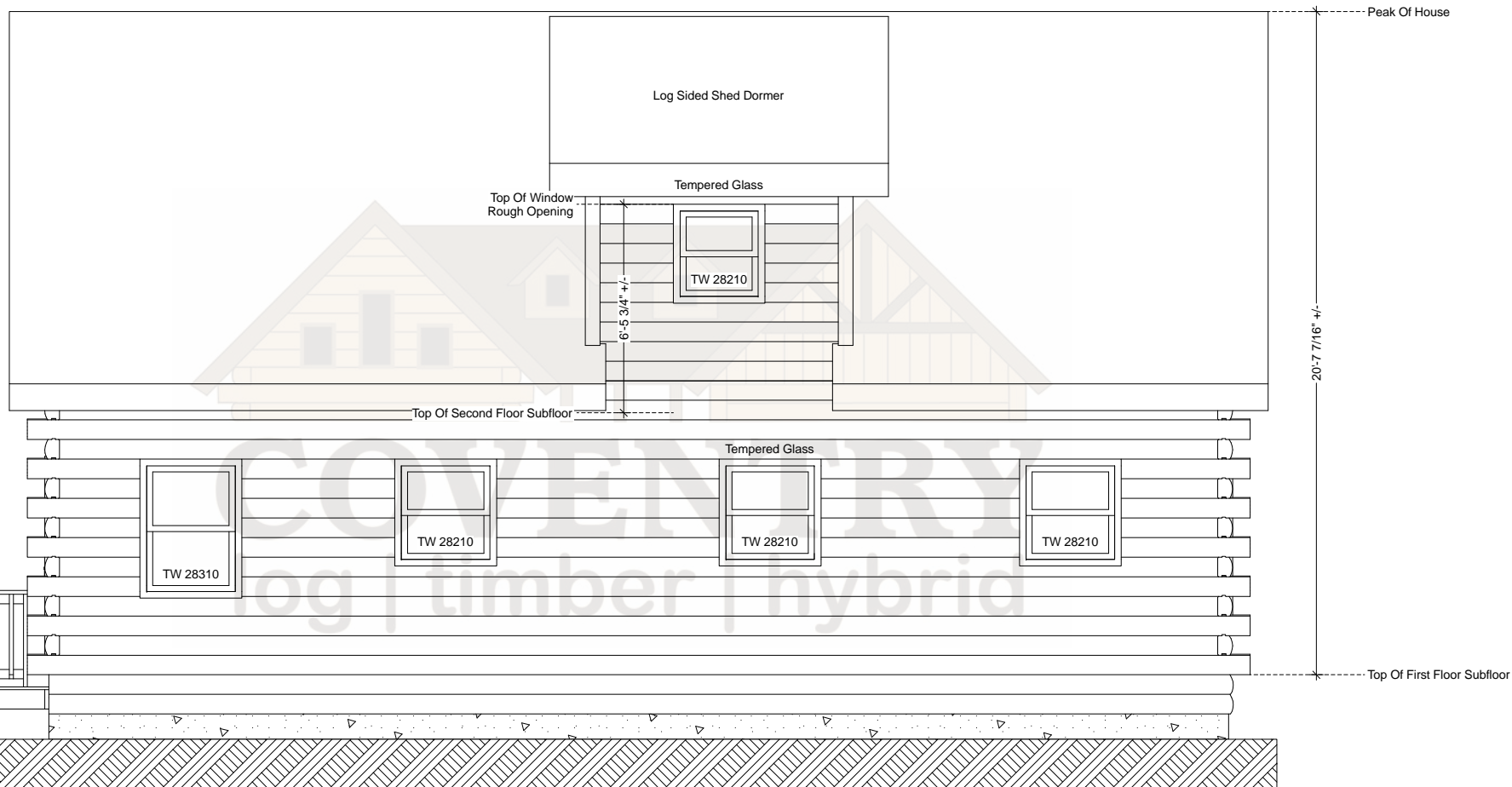
Riverside Right Elevation
