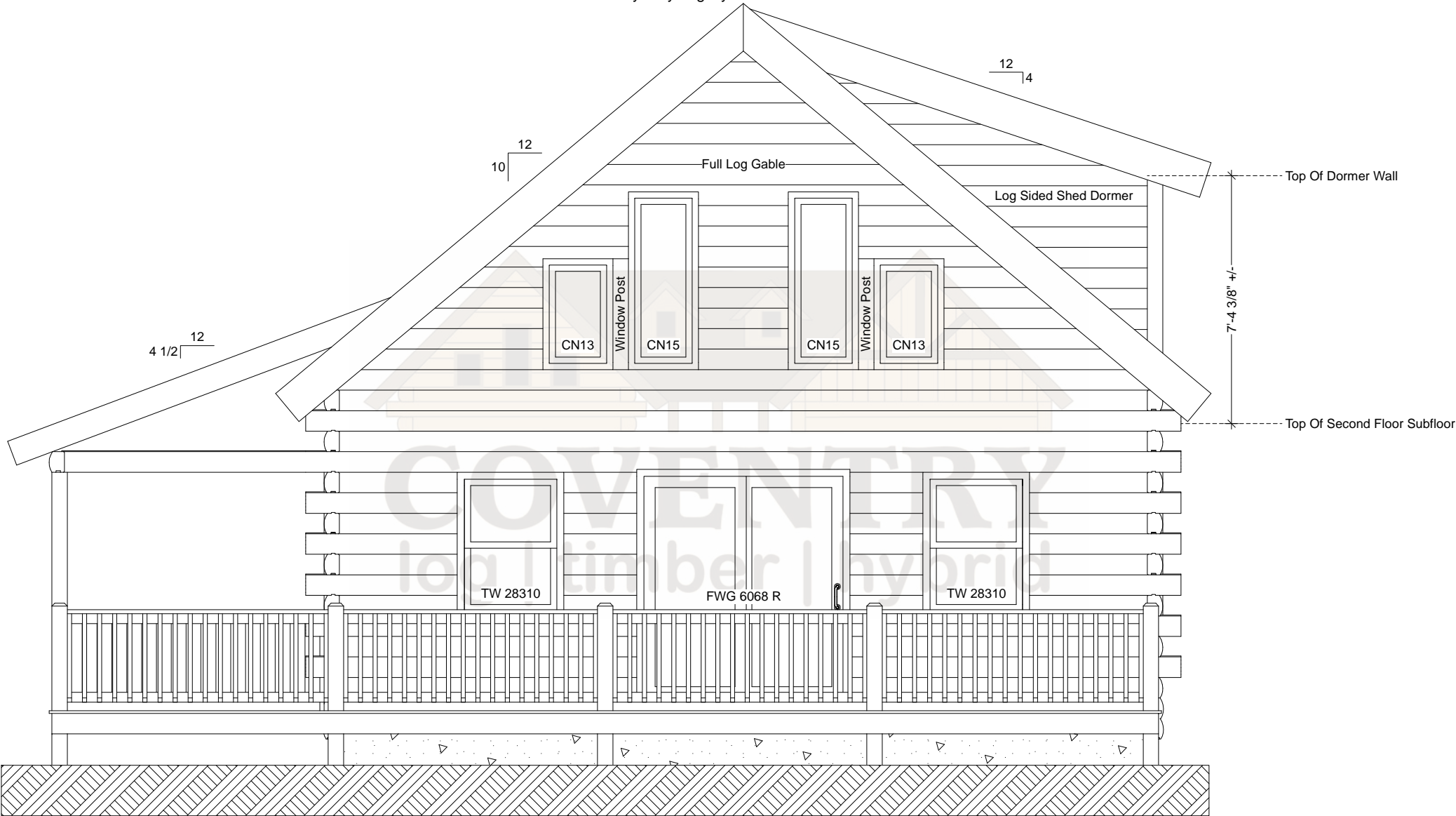
Riverside Front Elevation
