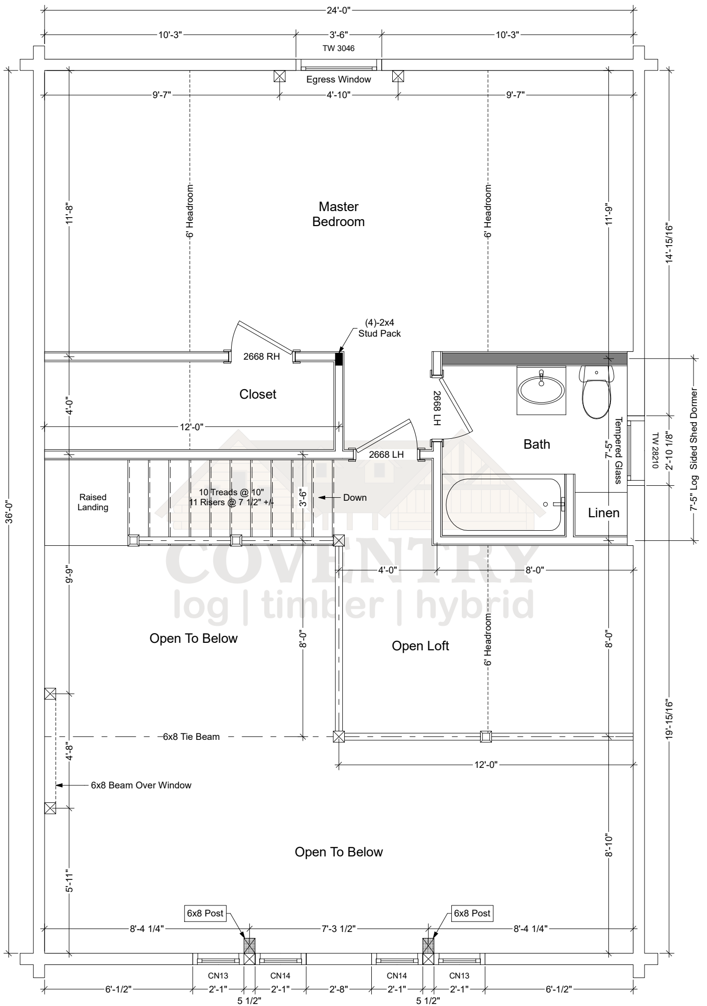
Riverside Second Floor Plan
