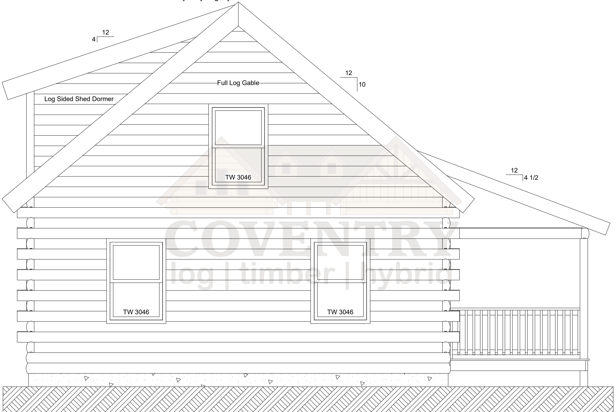
Riverside Rear Elevation
