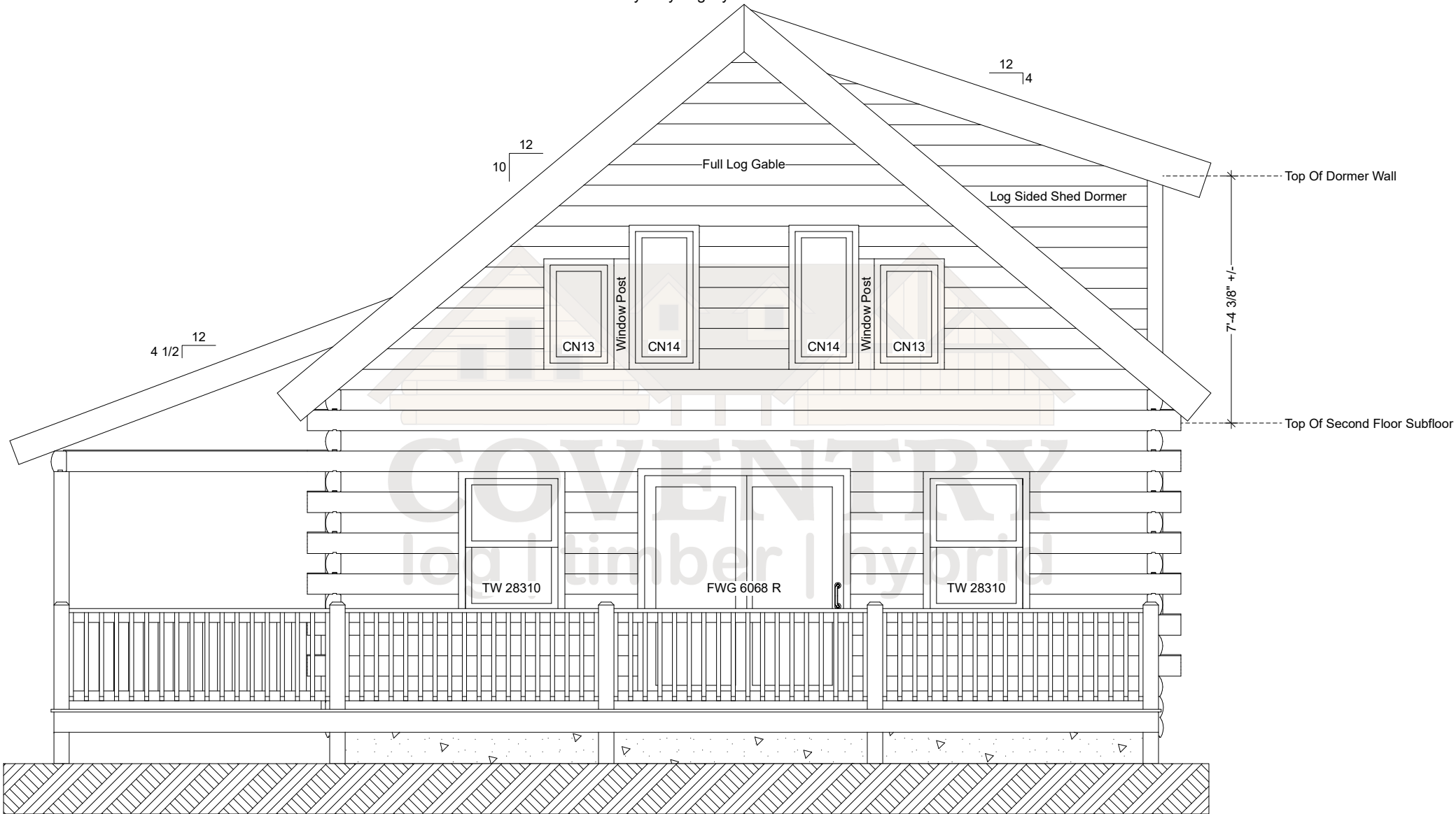
Riverside Front Elevation
