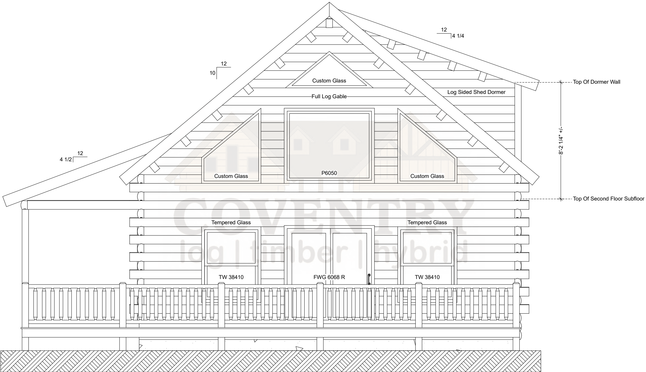
Skyline Front Elevation
