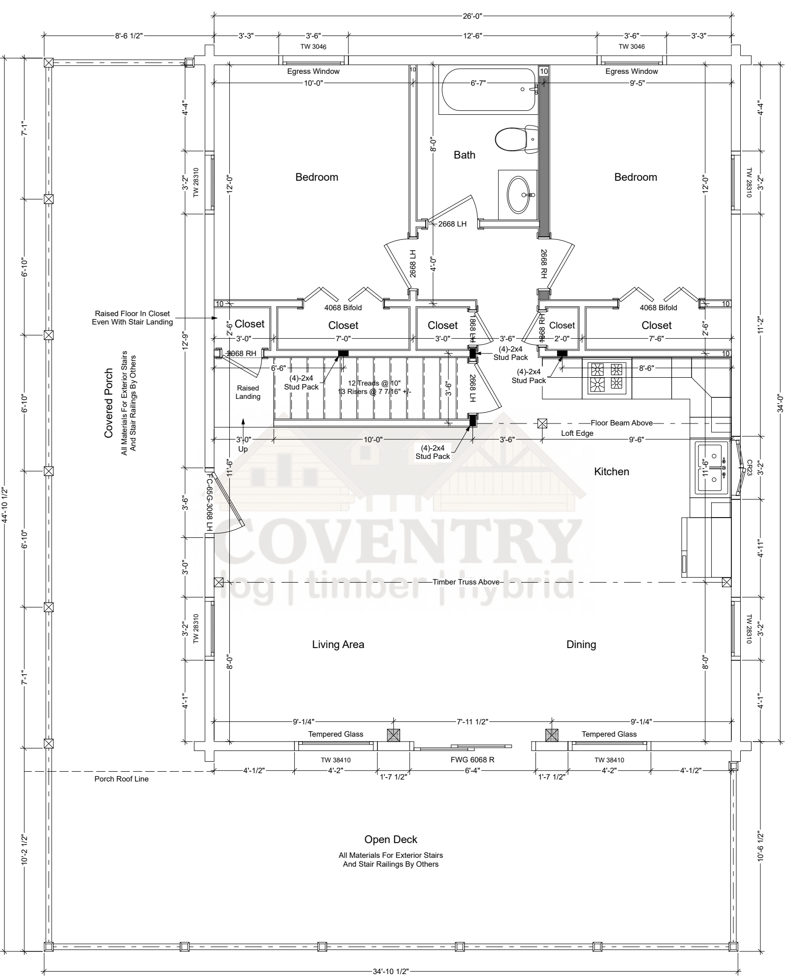
Skyline First Floor Plan
