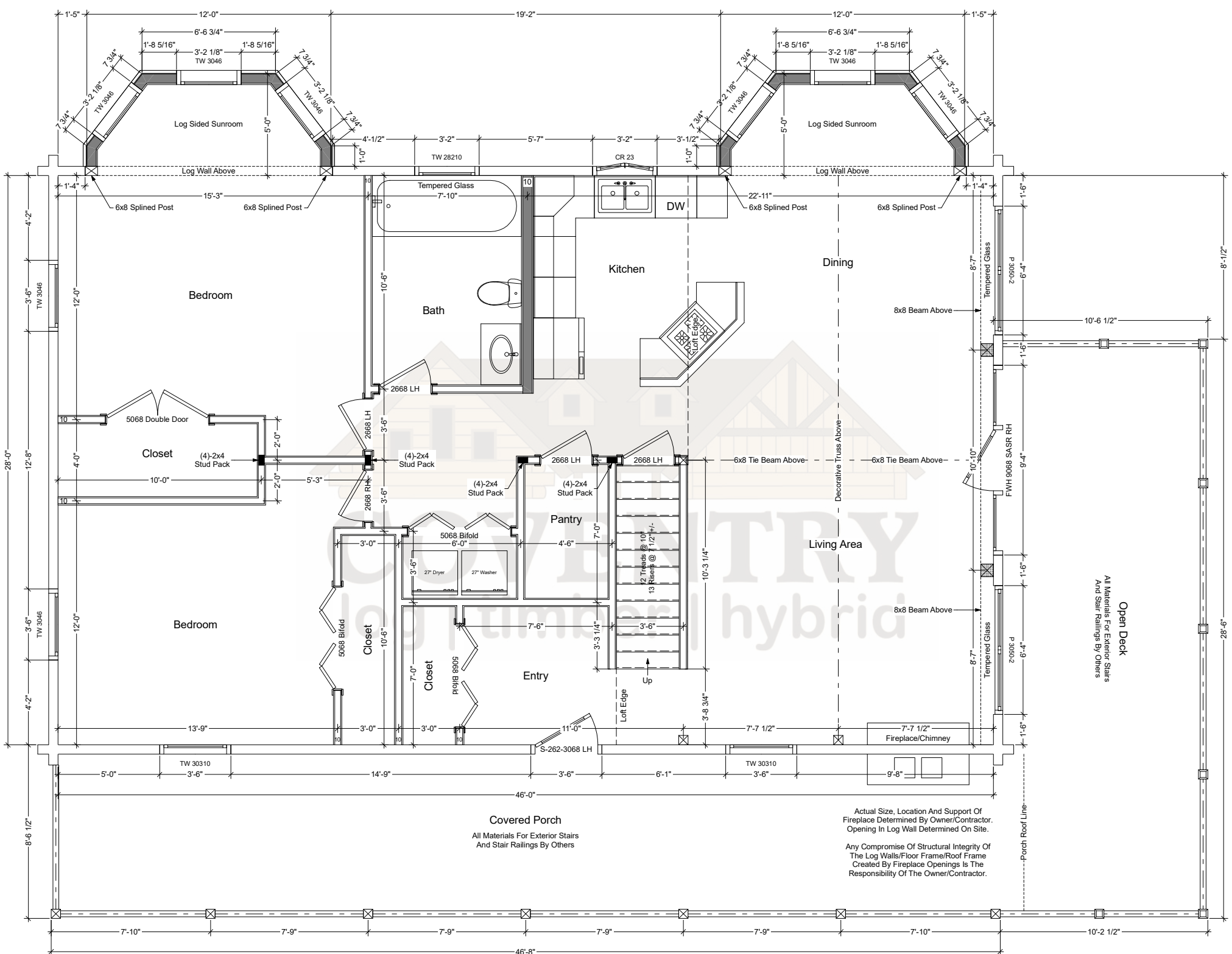
Spokane First Floor Plan
