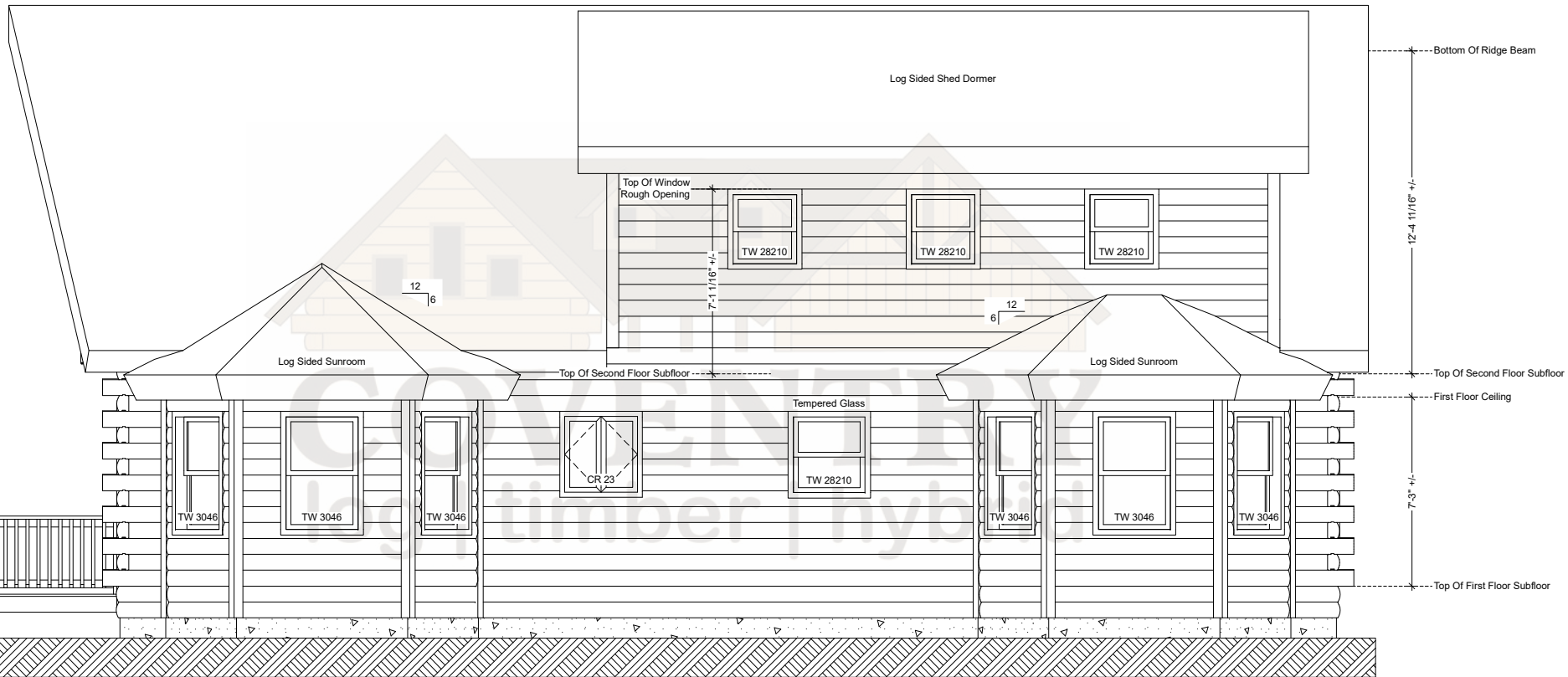
Spokane Rear Elevation
