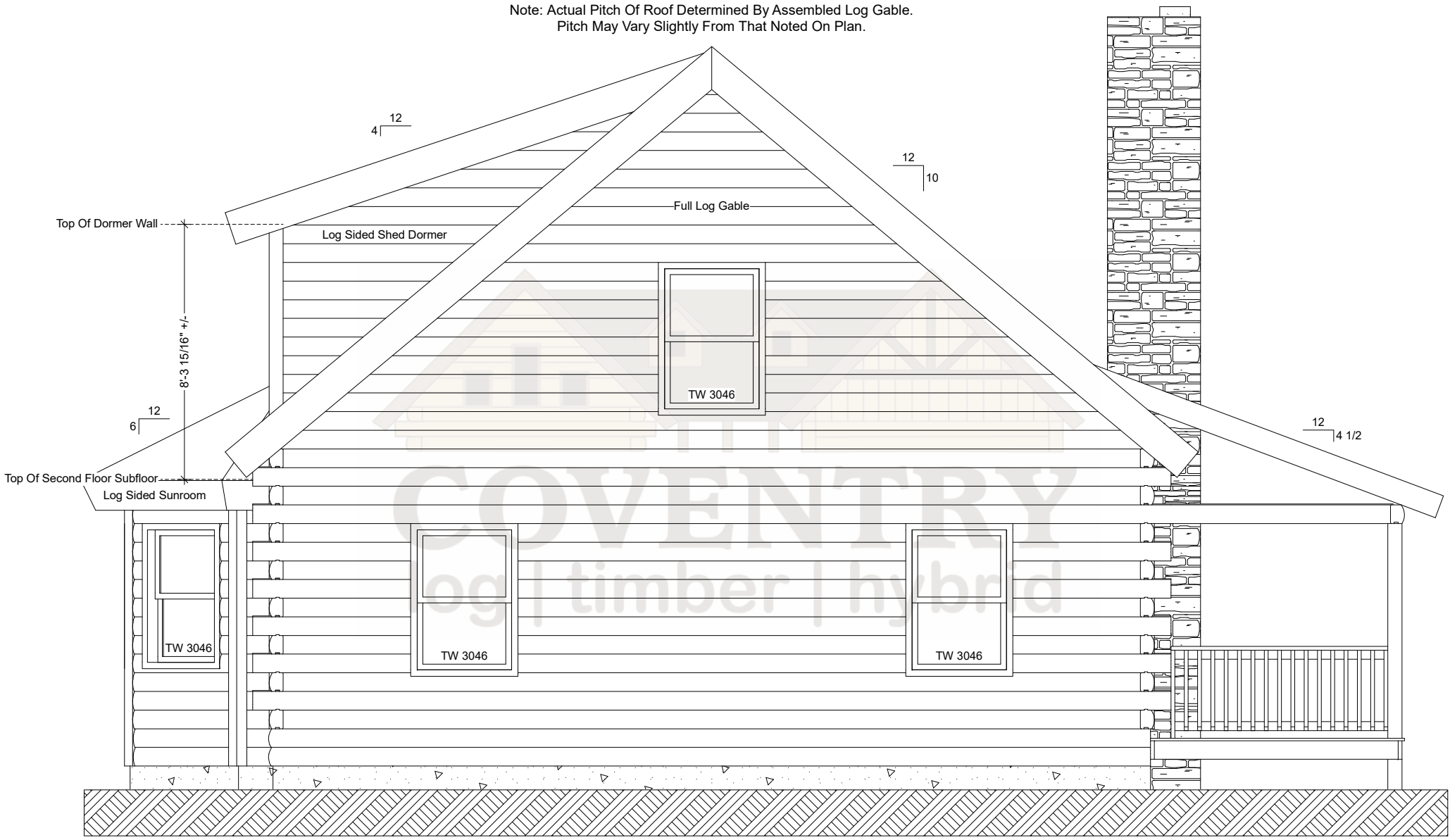
Spokane Left Elevation
