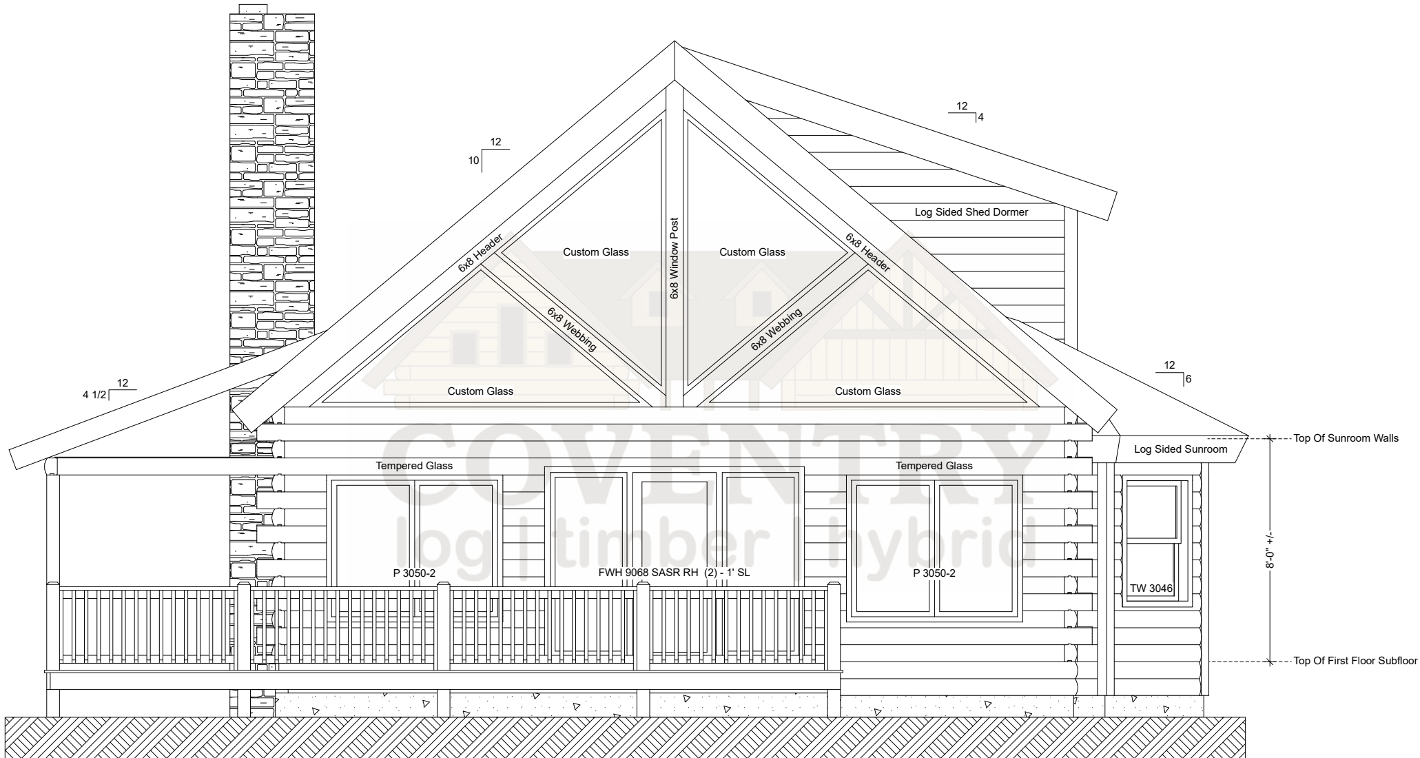
Spokane Right Elevation
