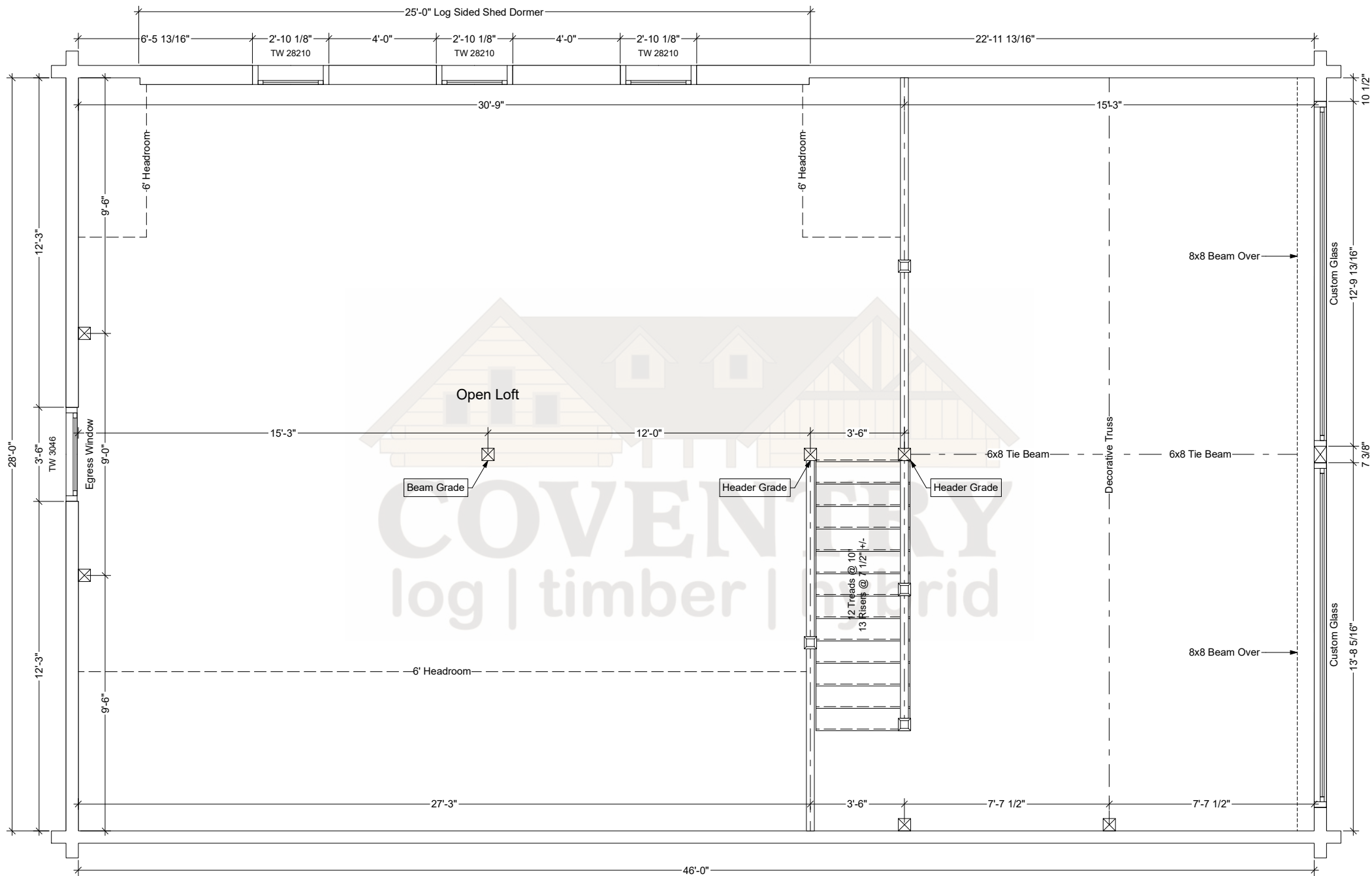
Spokane Second Floor Plan
