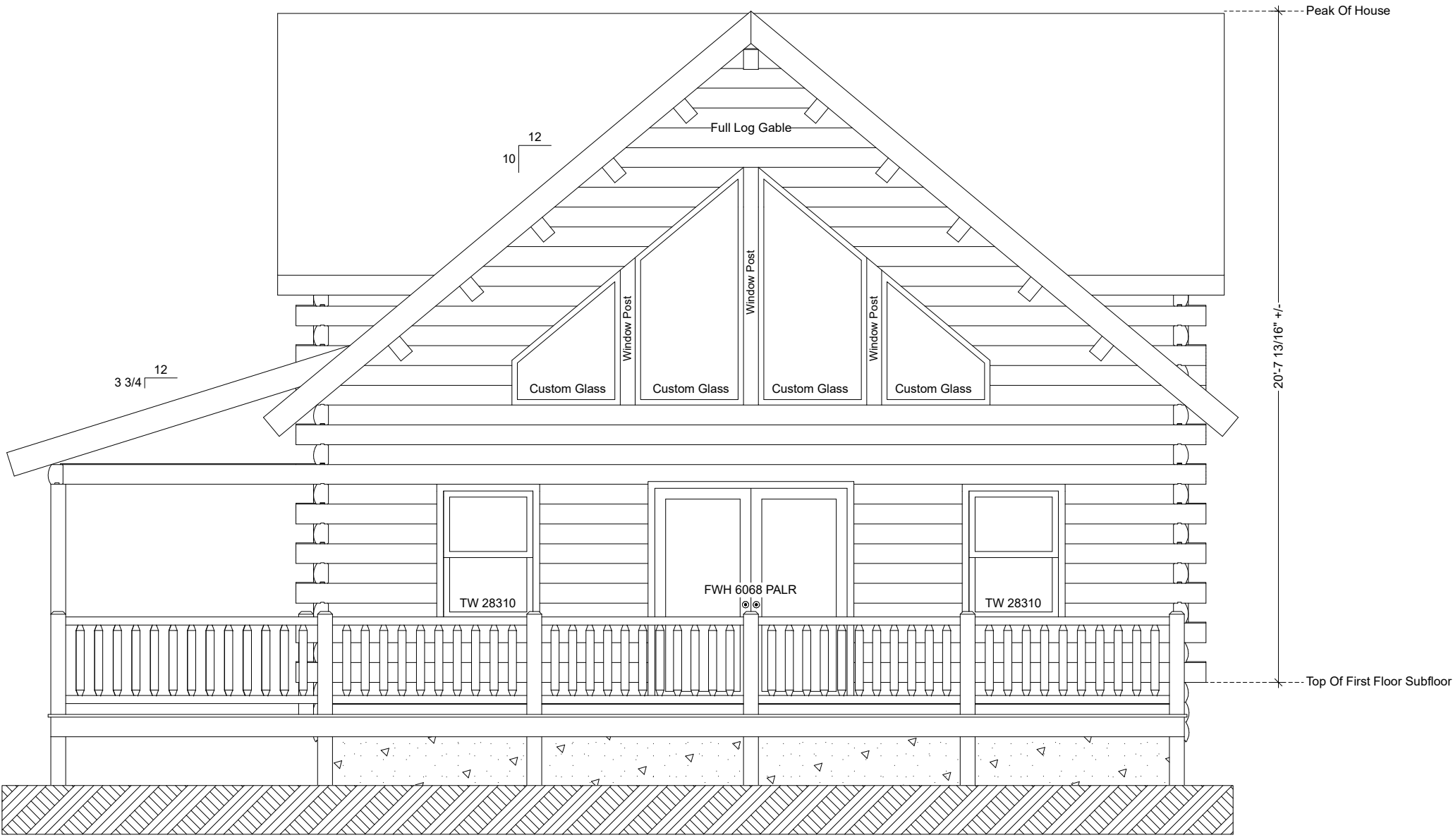
Summit View Front Elevation
