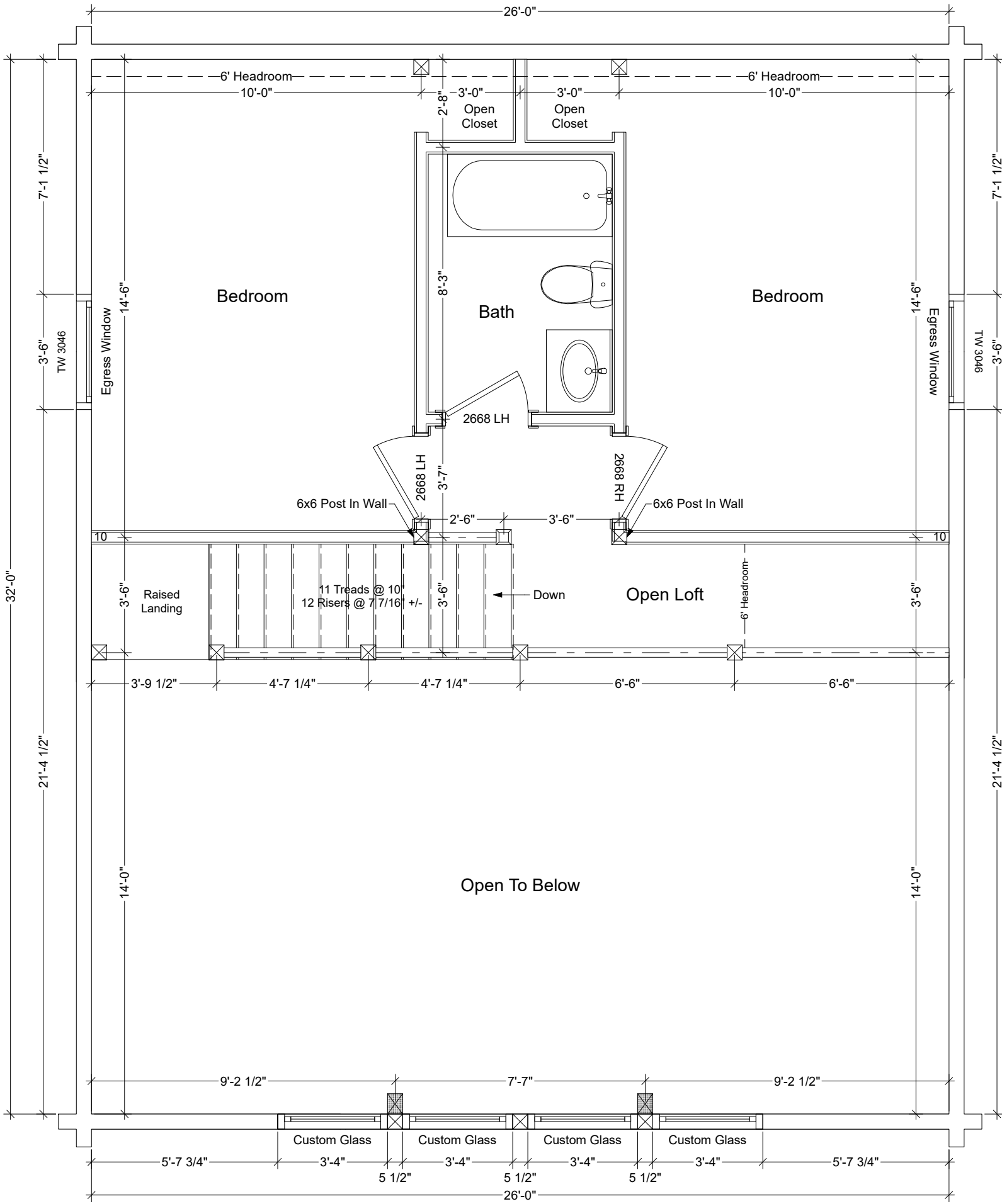
Summit View Second Floor Plan
