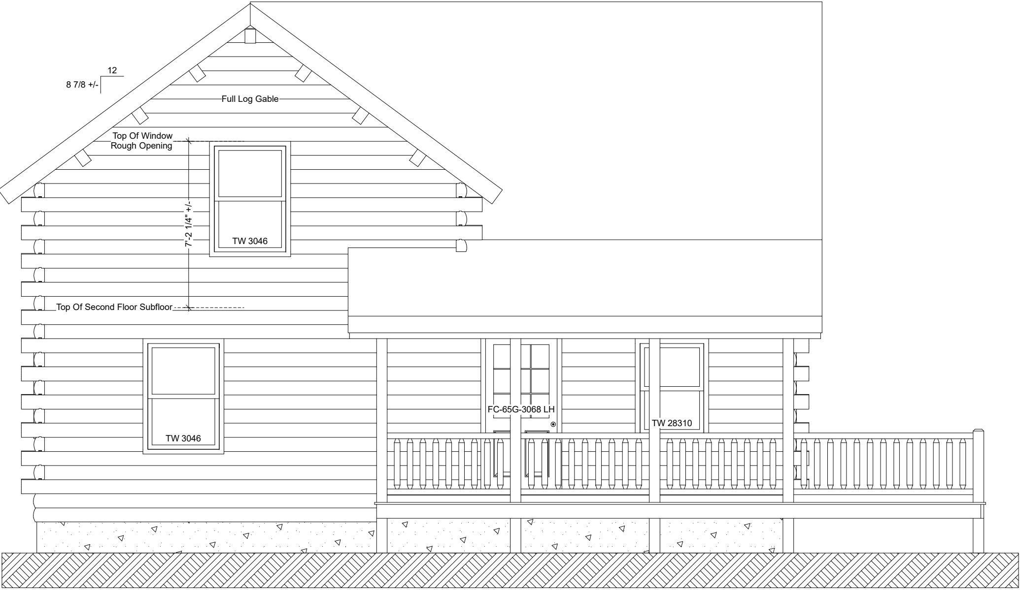
Summit View Left Elevation
