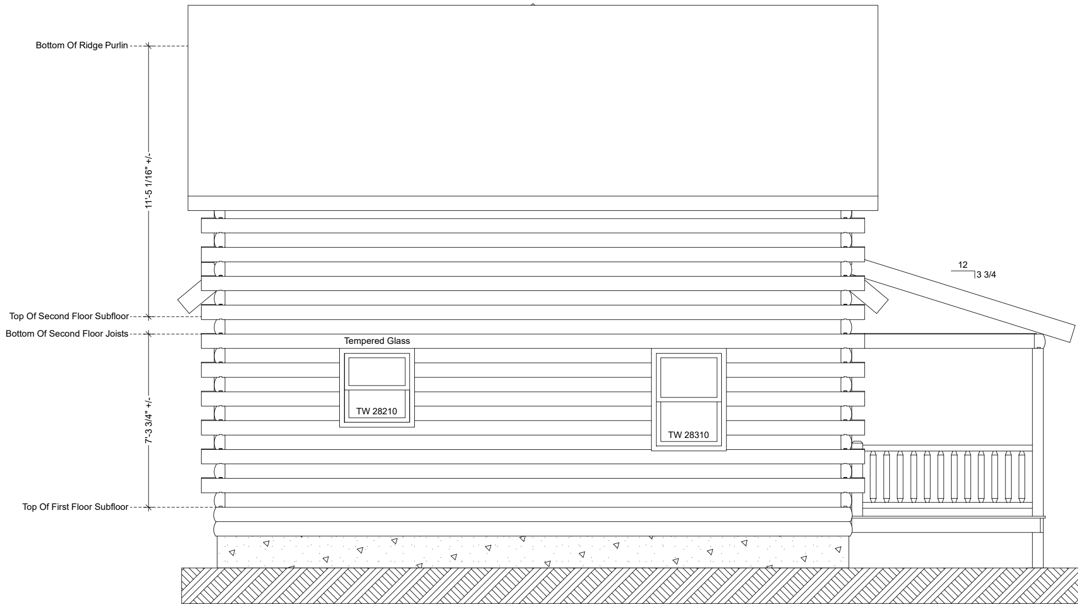
Summit View Rear Elevation
