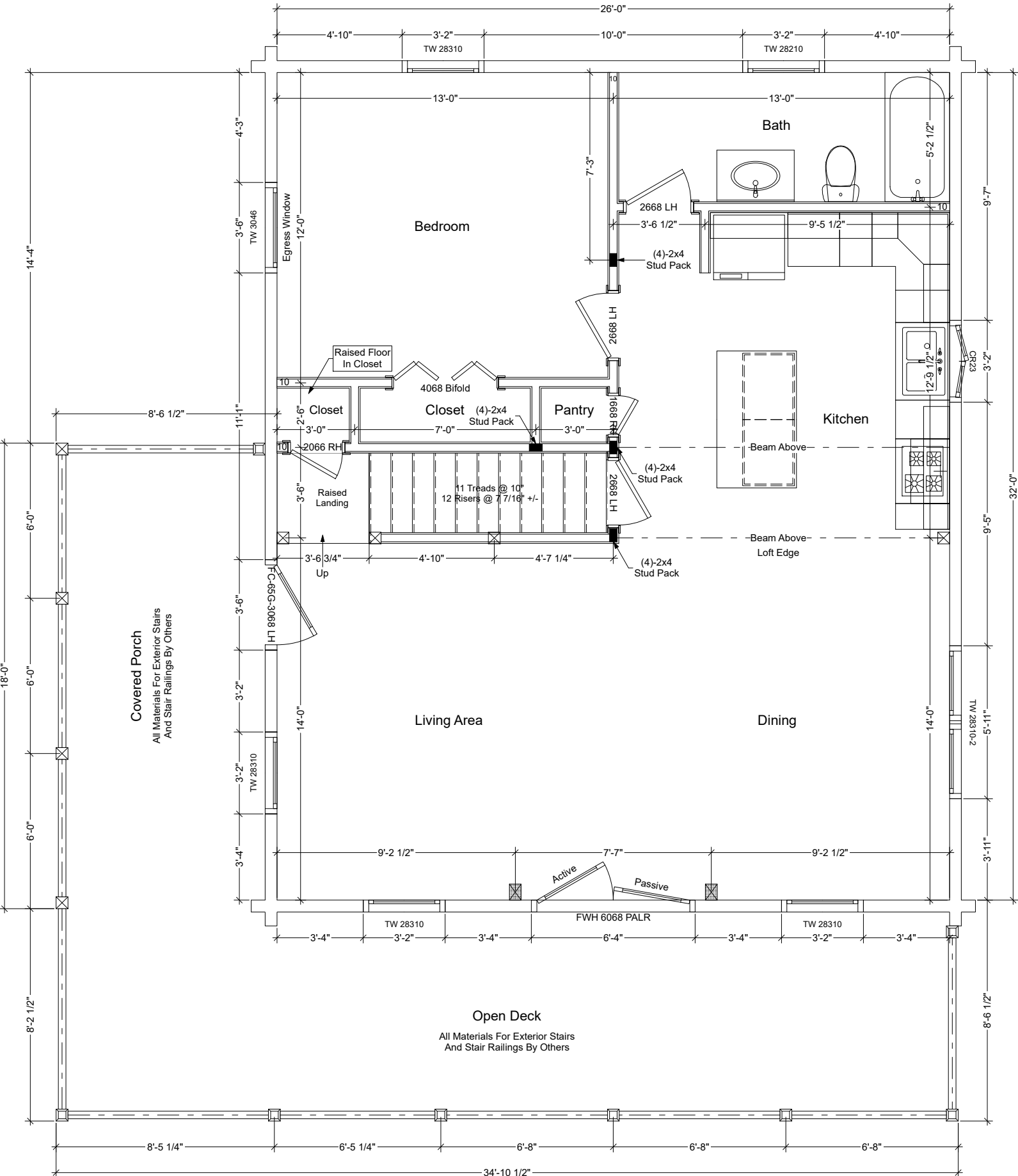
Summit View First Floor Plan
