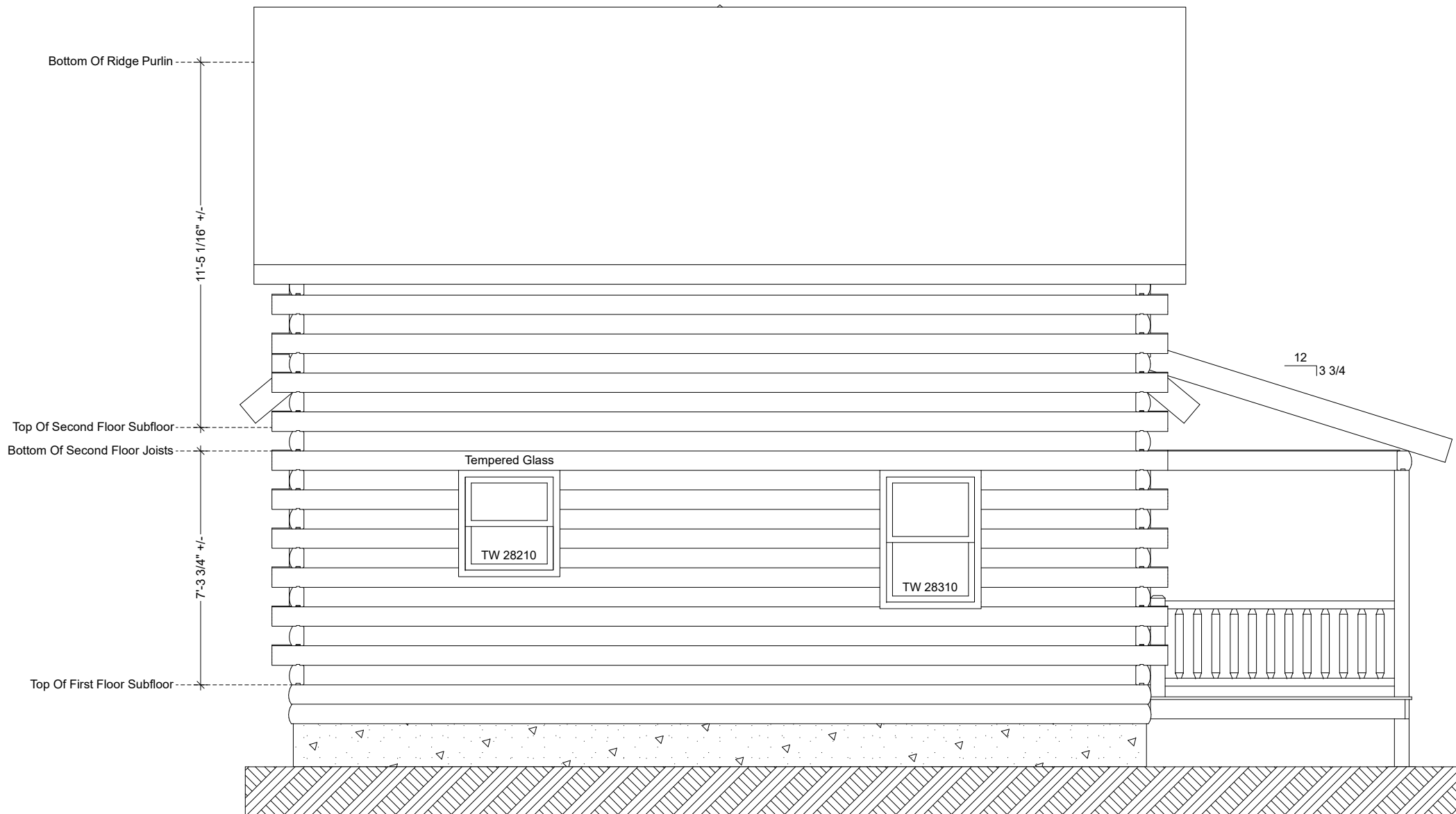
Summit View Rear Elevation
