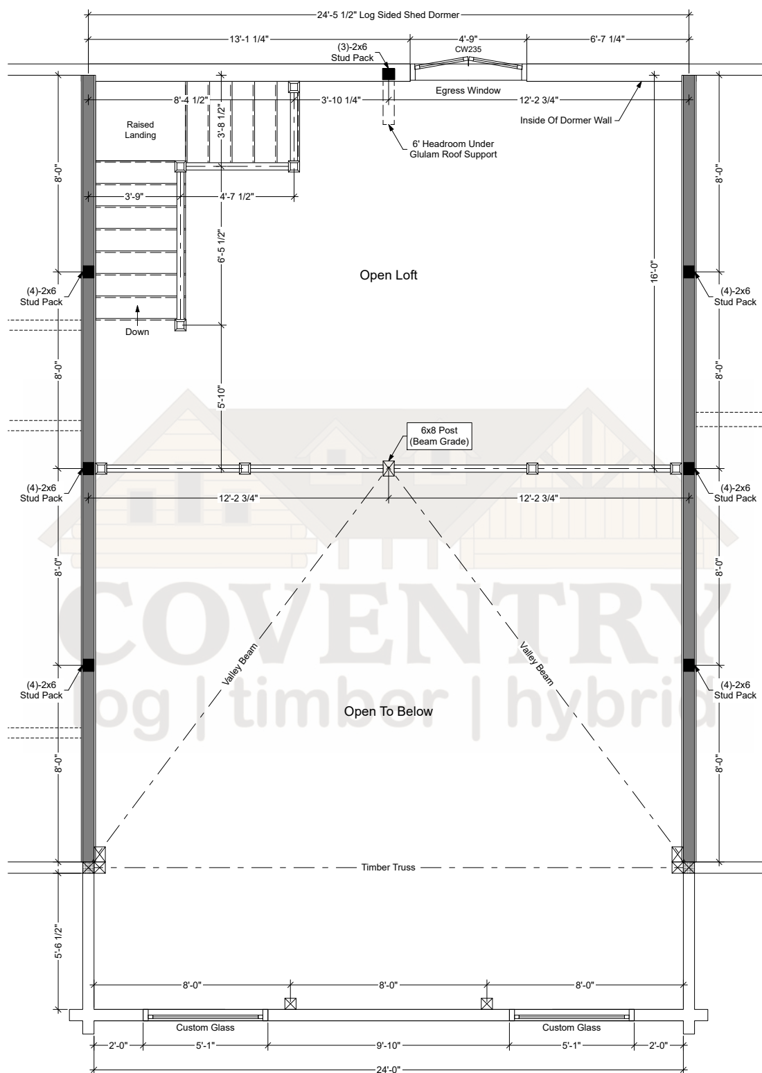
Sunapee Second Floor Plan
