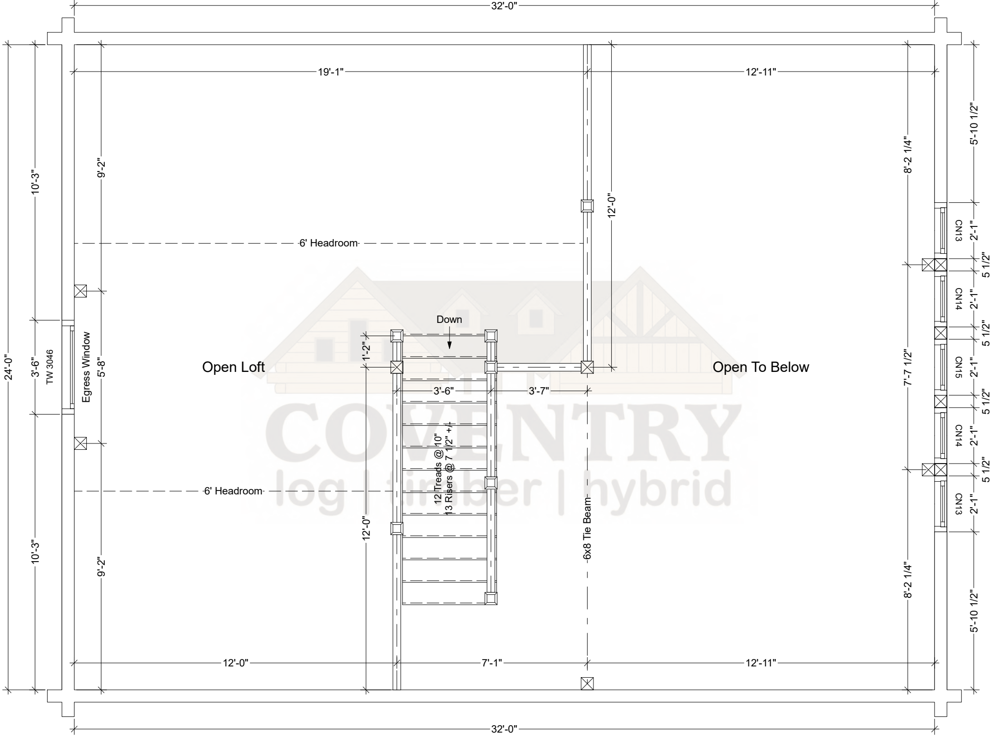
Swiftwater Second Floor Plan
