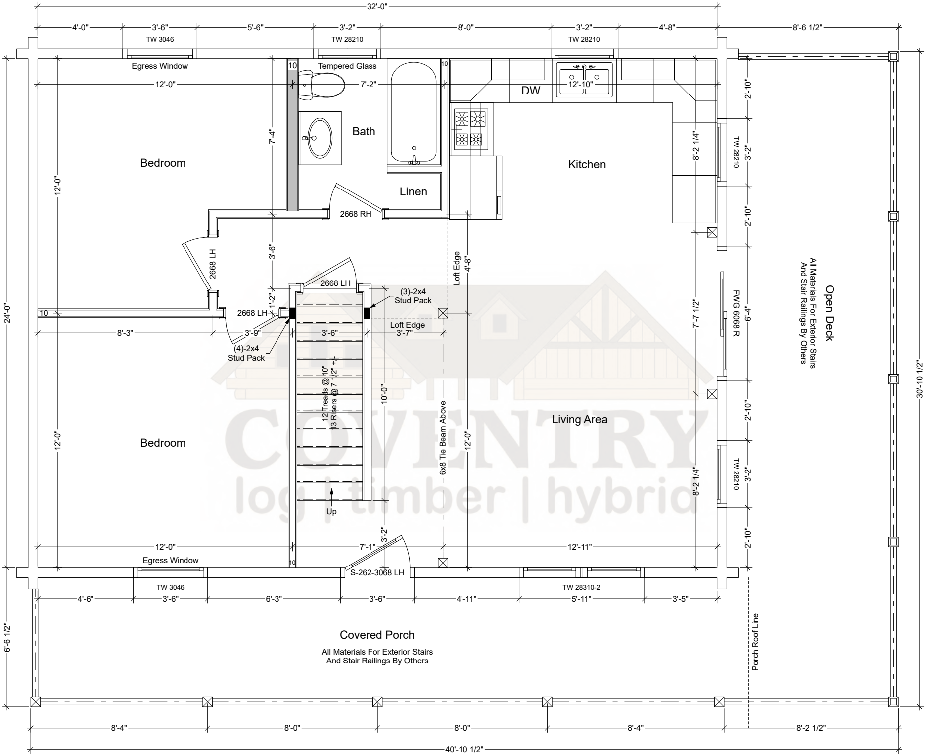
Swiftwater First Floor Plan
