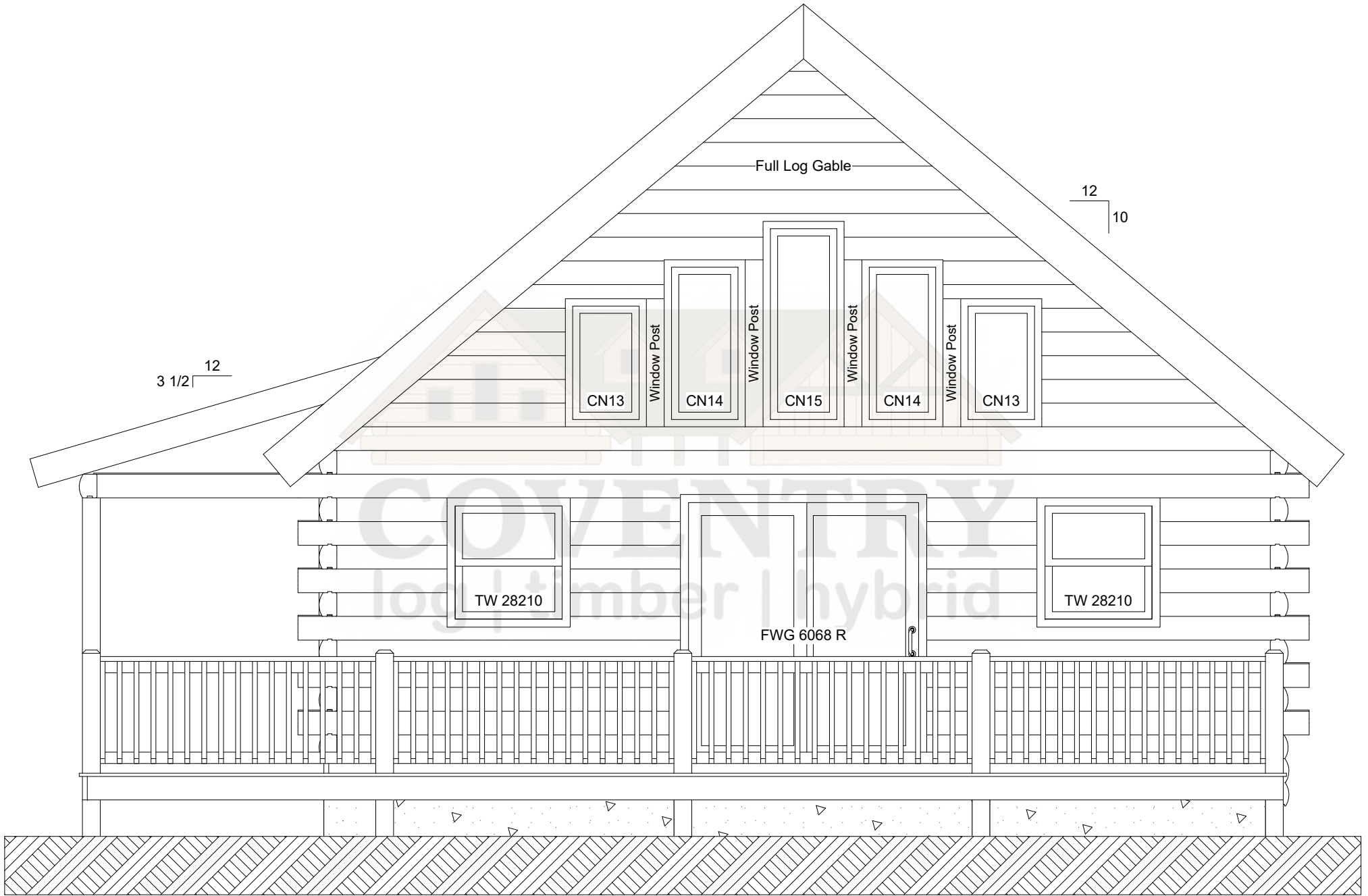
Swiftwater Right Elevation
