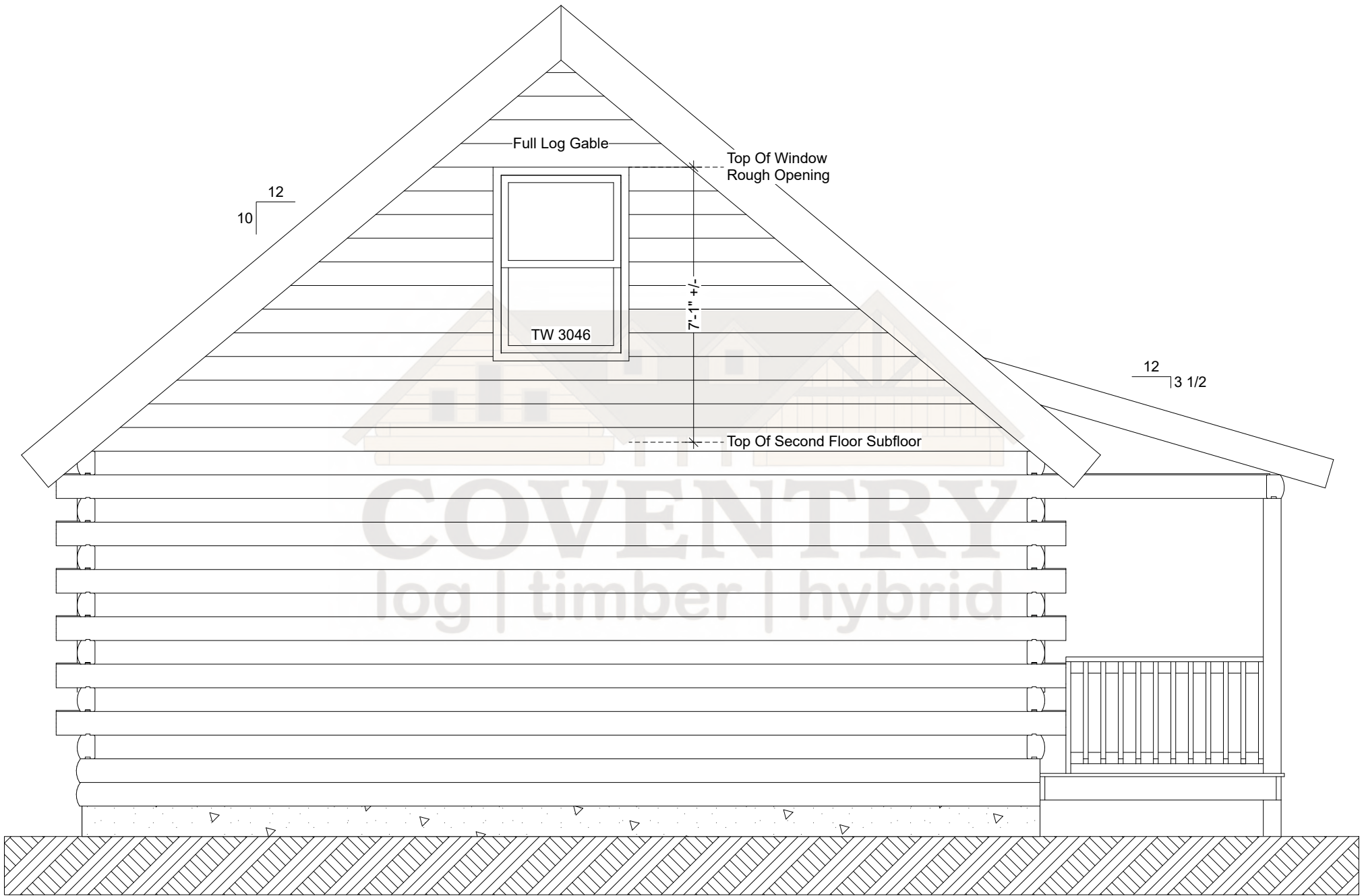
Swiftwater Left Elevation
