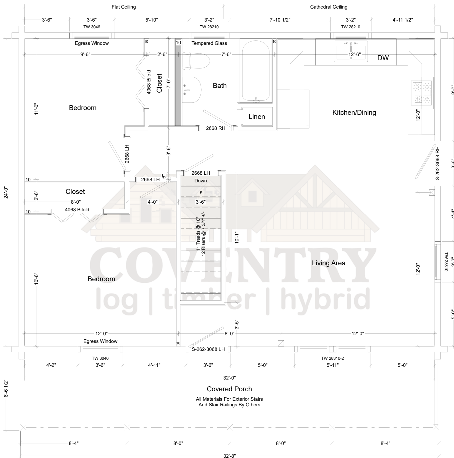
Westport First Floor Plan
