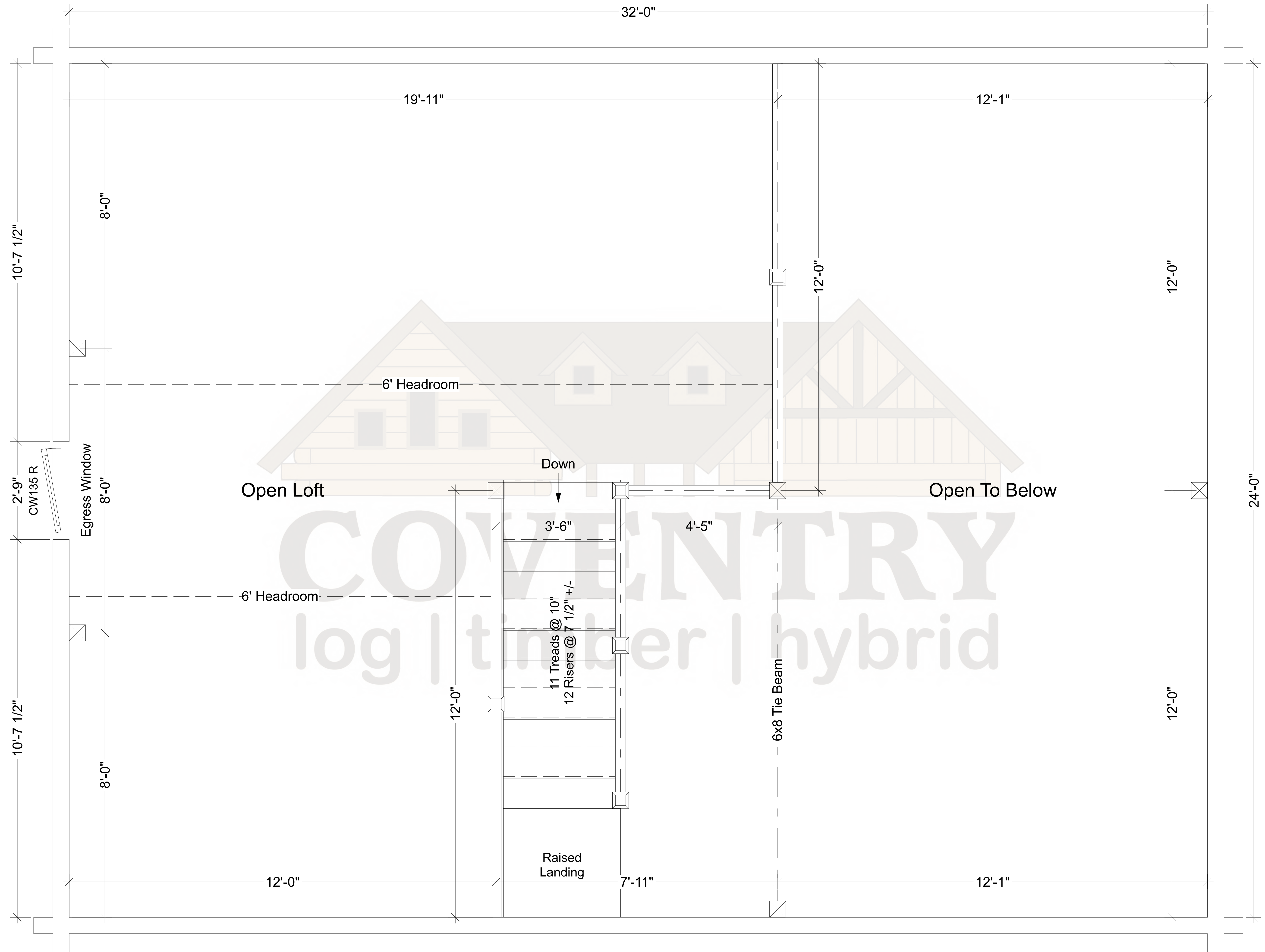
Woodland Second Floor Plan
