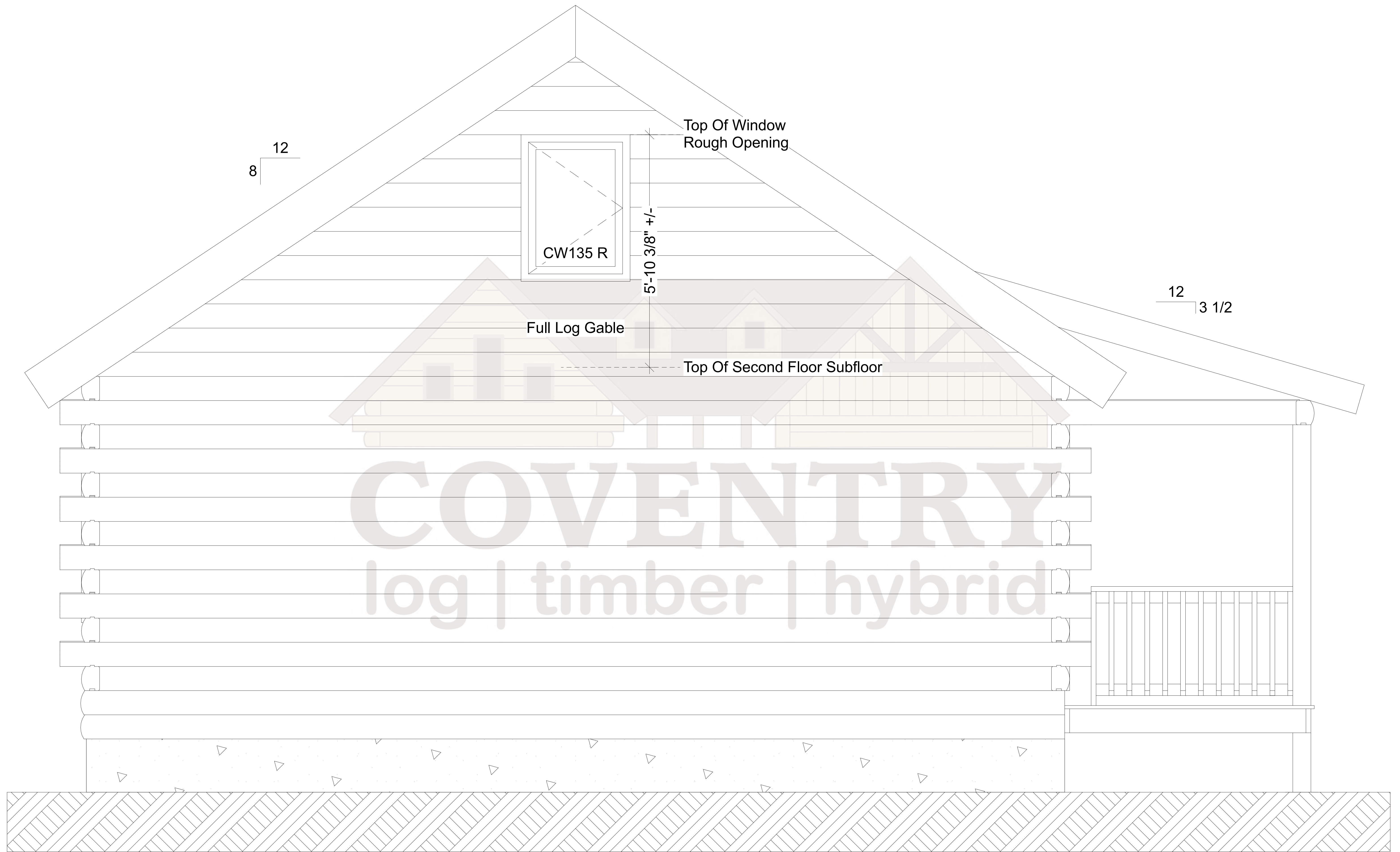
Woodland Left Elevation
