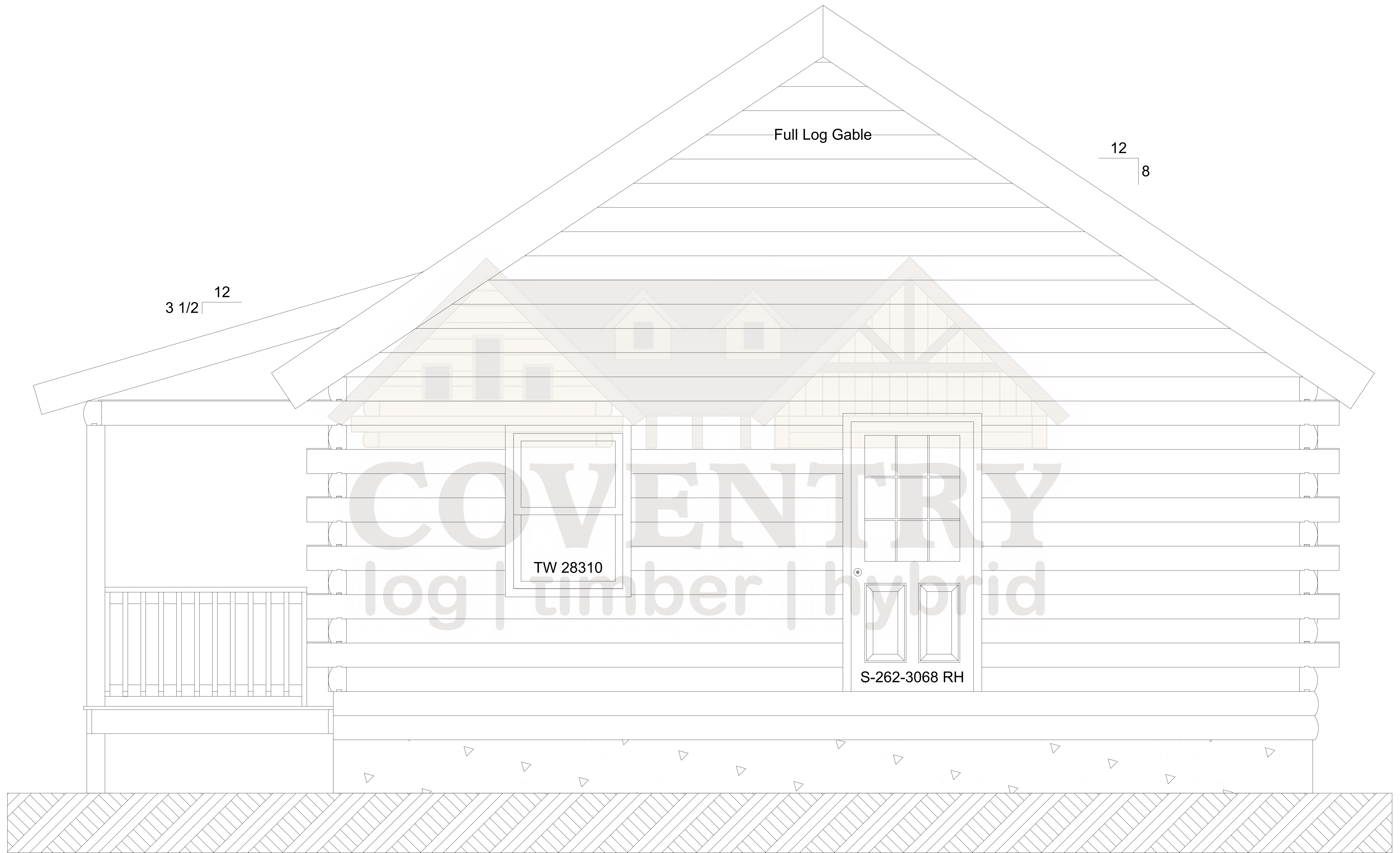
Woodland Right Elevation
