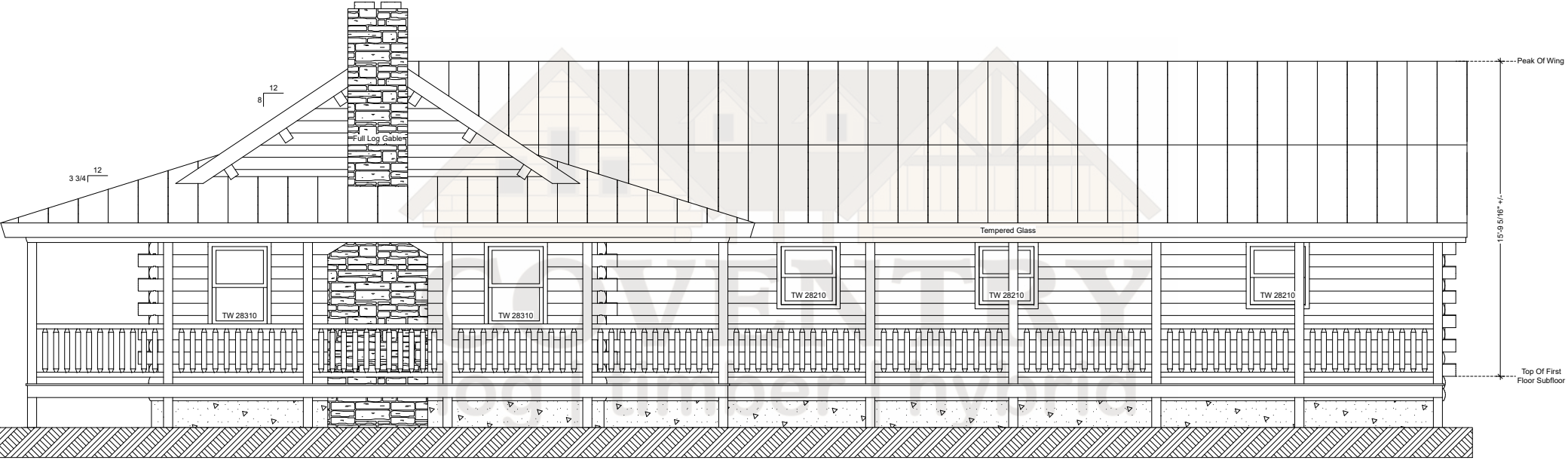
Woodsman Front Elevation
