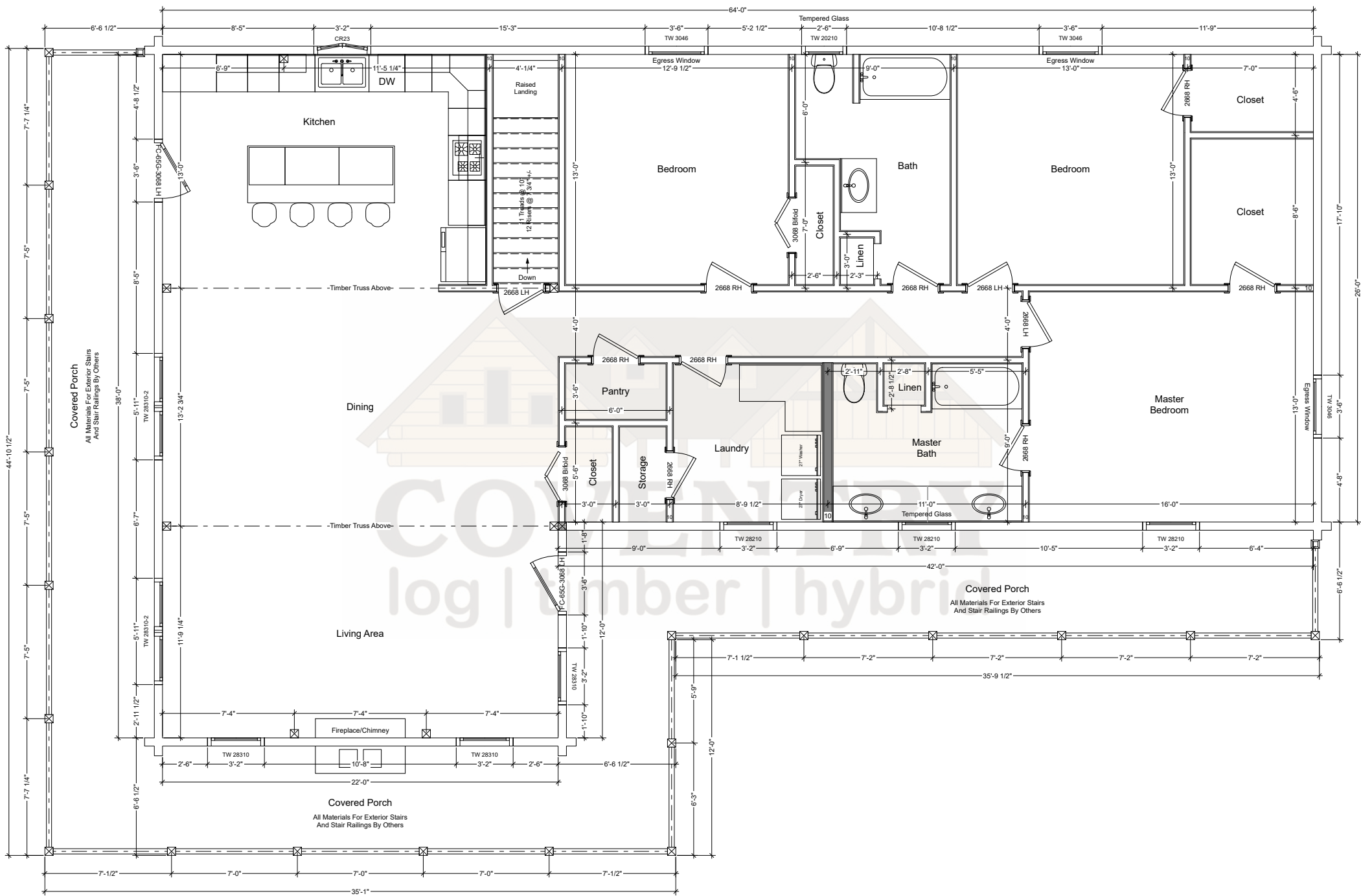
Woodsman First Floor Plan
