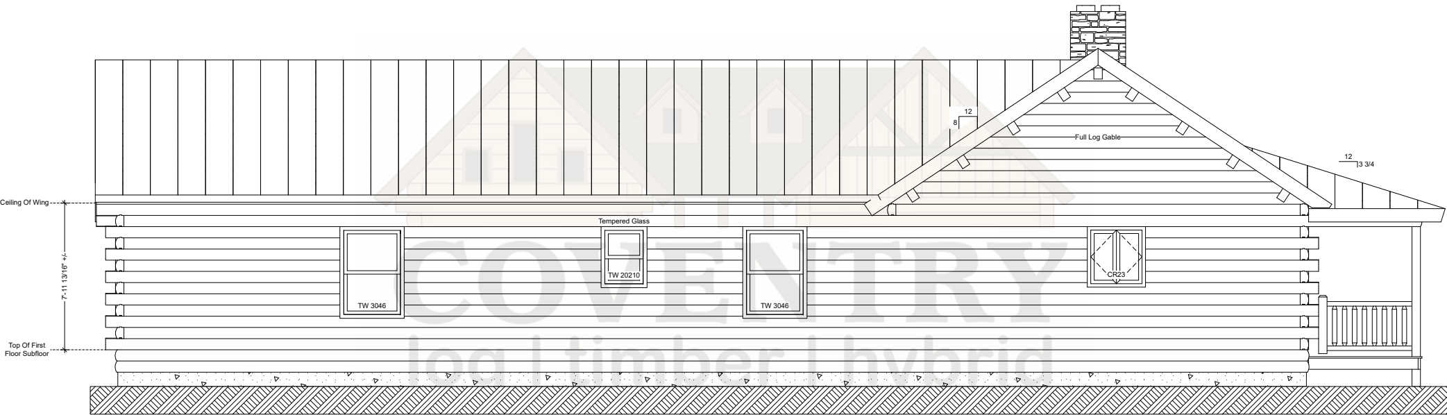
Woodsman Rear Elevation
