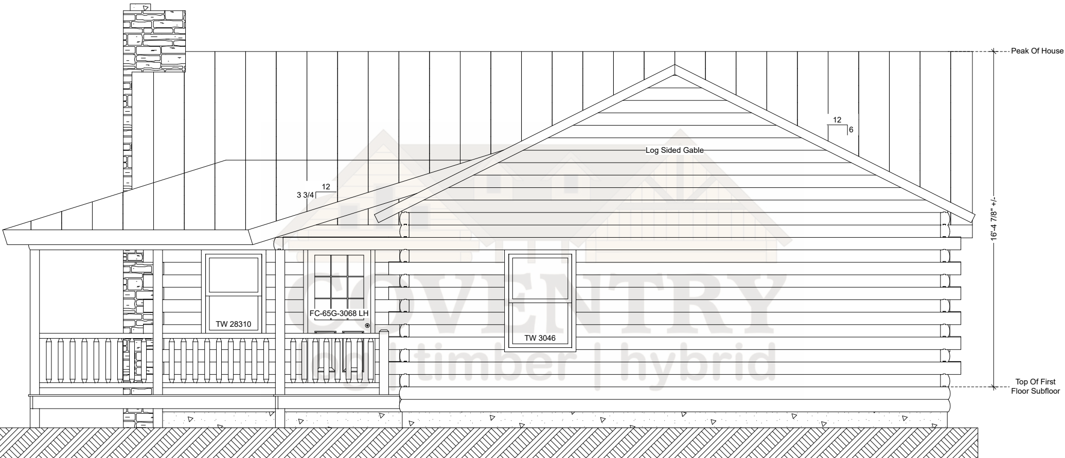
Woodsman Right Elevation
