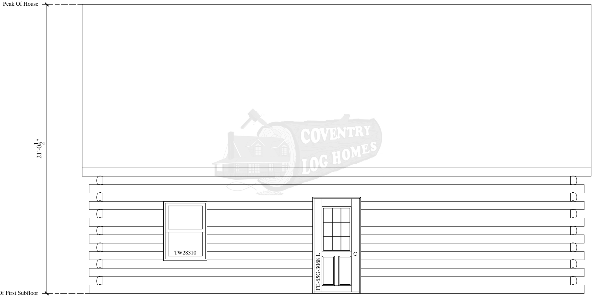
Elevation D
