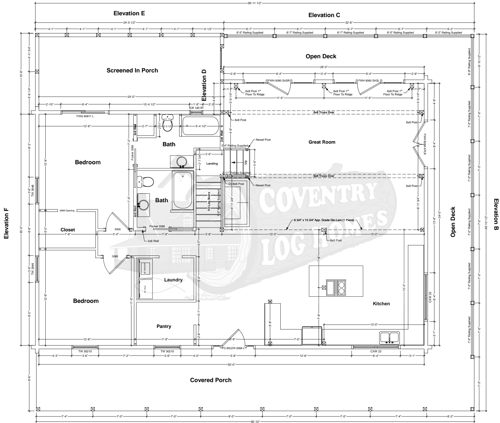
FLOOR PLAN
