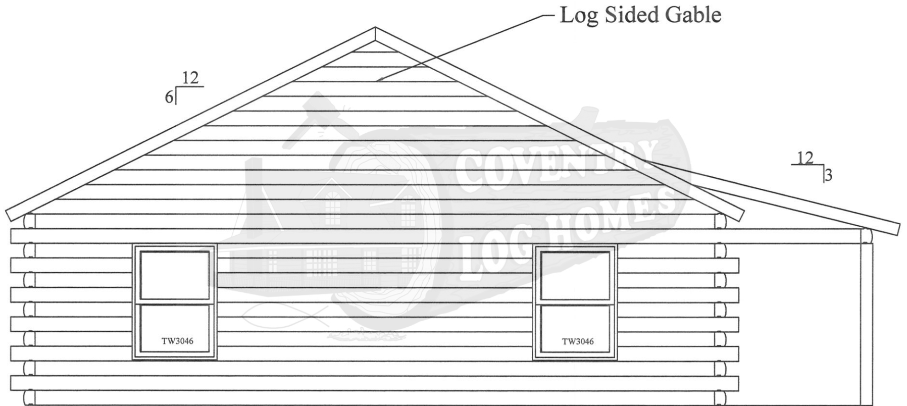
ELEVATION "D"
