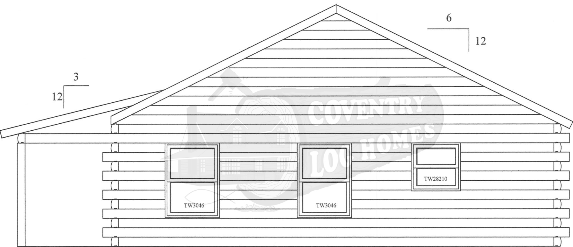
ELEVATION "B"
