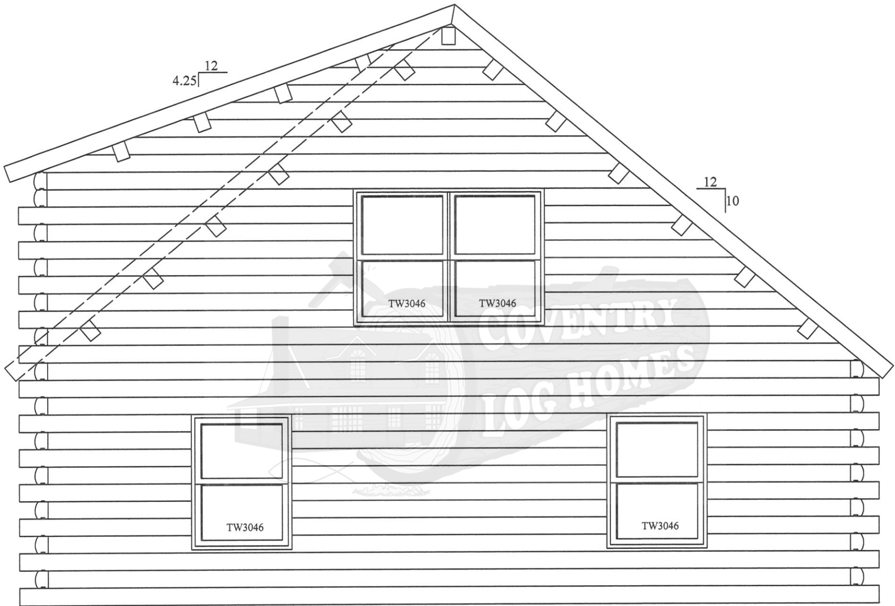
Elevation "C" Standard "Mountain View"
