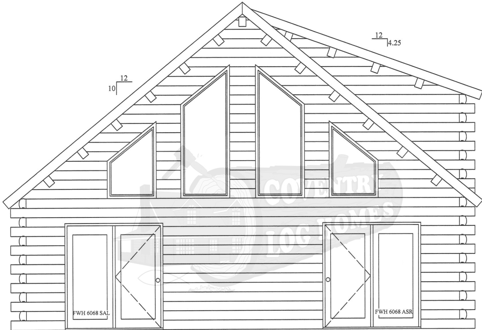
Elevation "A"
