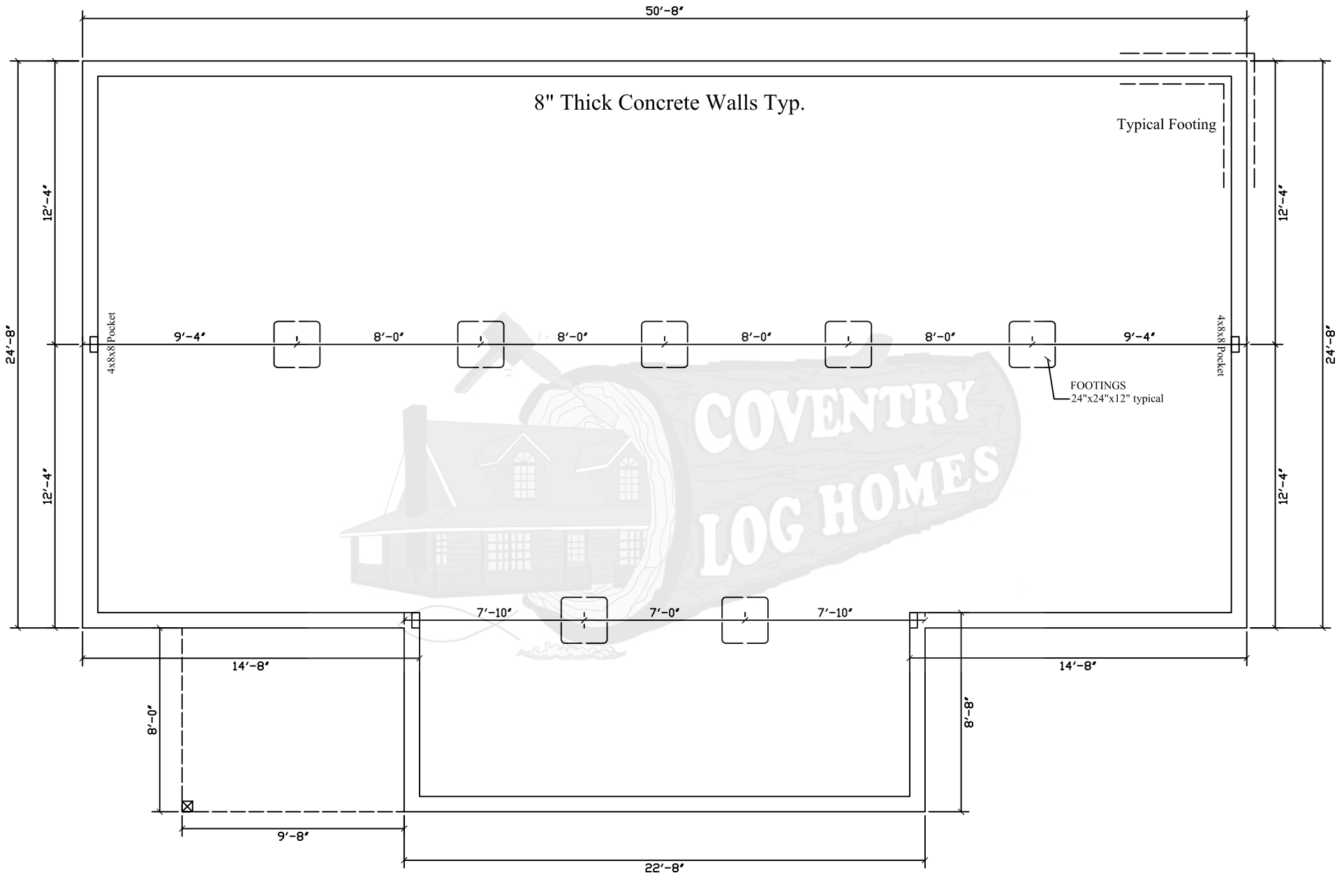
Foundation Plan
